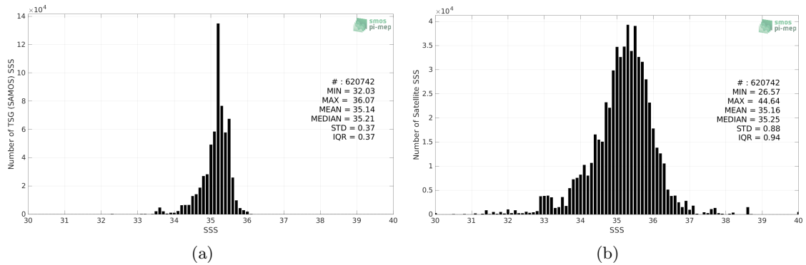
Figure 2: Histograms of SSS from TSG (SAMOS) (a) and SMAP SSS L2 v5.0 (JPL) (b) considering all match-up pairs per bins of 0.1 over the South Pacific Ocean Pi-MEP region and for the full satellite product period.
