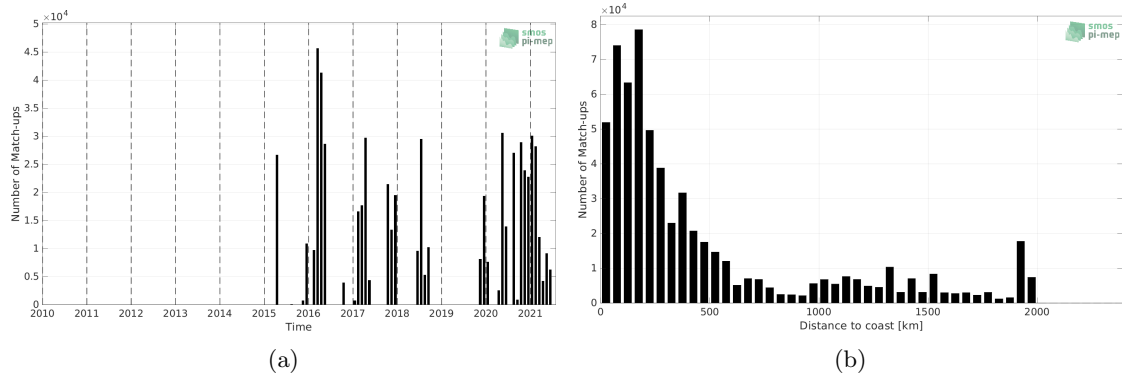
Figure 1: Number of match-ups between TSG (SAMOS) and SMAP SSS L2 v5.0 (JPL) SSS as a function of time (a) and as function of the distance to coast (b) over the South Pacific Ocean Pi-MEP region and for the full satellite product period.
