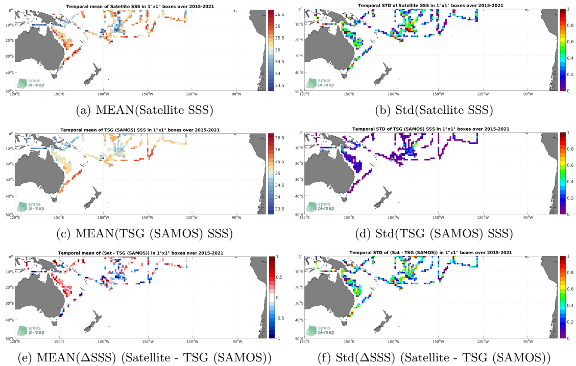
Figure 6: Temporal mean (left) and Std (right) of SSS from SMAP SSS L2 v5.0 (JPL) (top), TSG (SAMOS) (middle), and of \Delta SSS (Satellite - TSG (SAMOS)). Only match-up pairs are used to generate these maps.
