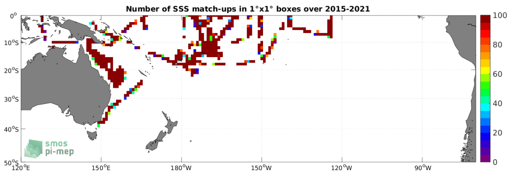
Figure 4: Number of SSS match-ups between TSG (SAMOS) SSS and the SMAP SSS L2 v5.0 (JPL) SSS product for the South Pacific Ocean Pi-MEP region over 1^\circ \times 1^\circ boxes and for the full satellite product period.
