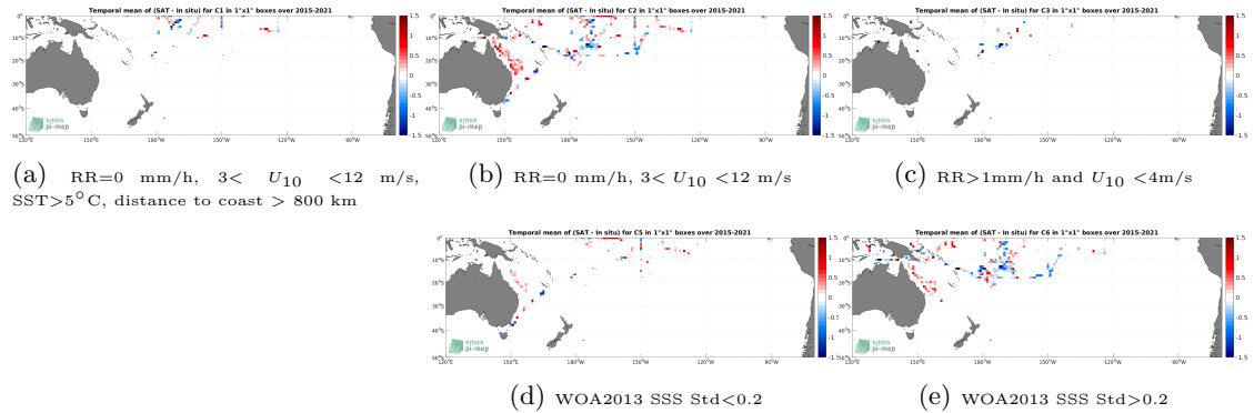
Figure 12: Temporal mean gridded over spatial boxes of size 1^\circ \times 1^\circ of \Delta SSS (SMAP SSS L2 v5.0 (JPL) - TSG (SAMOS)) for 5 different subdatasets corresponding to:RR=0 mm/h, 3 < U_{10} < 12 m/s, SST >5^\circ\text{C} , distance to coast > 800 km (a), RR=0 mm/h, 3 < U_{10} < 12 m/s (b), RR >1 mm/h and U_{10} < 4 m/s (c), WOA2013 SSS Std <0.2 (d), WOA2013 SSS Std >0.2 (e).
