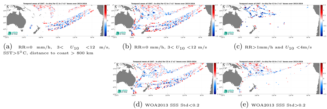
Figure 14: Temporal mean gridded over spatial boxes of size 1^\circ \times 1^\circ of \Delta\text{SSS} (SMAP SSS L2 v5.0 (JPL) - TSG (LEGOS-DM)) for 5 different subdatasets corresponding to:RR=0 mm/h, 3 < U_{10} < 12 m/s, SST>5°C, distance to coast > 800 km (a), RR=0 mm/h, 3 < U_{10} < 12 m/s (b), RR>1mm/h and U_{10} < 4 m/s (c), WOA2013 SSS Std<0.2 (d), WOA2013 SSS Std>0.2 (e).
