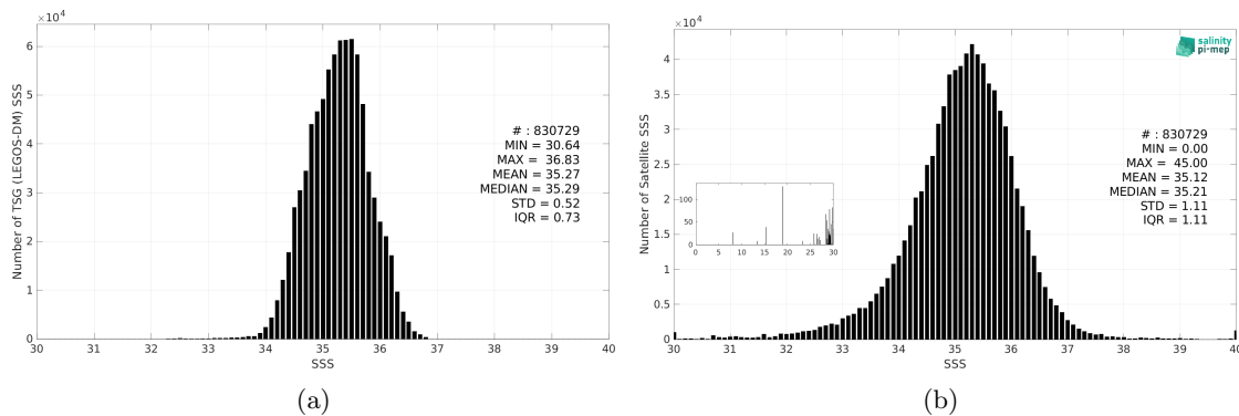
Figure 3: Histograms of SSS from TSG (LEGOS-DM) (a) and SMAP SSS L2 v5.0 (JPL) (b) considering all match-up pairs per bins of 0.1 over the South Pacific Ocean Pi-MEP region and for the full satellite product period.
