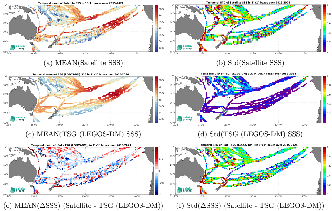
Figure 7: Temporal mean (left) and Std (right) of SSS from SMAP SSS L2 v5.0 (JPL) (top), TSG (LEGOS-DM) (middle), and of \Delta SSS (Satellite - TSG (LEGOS-DM)). Only match-up pairs are used to generate these maps.
