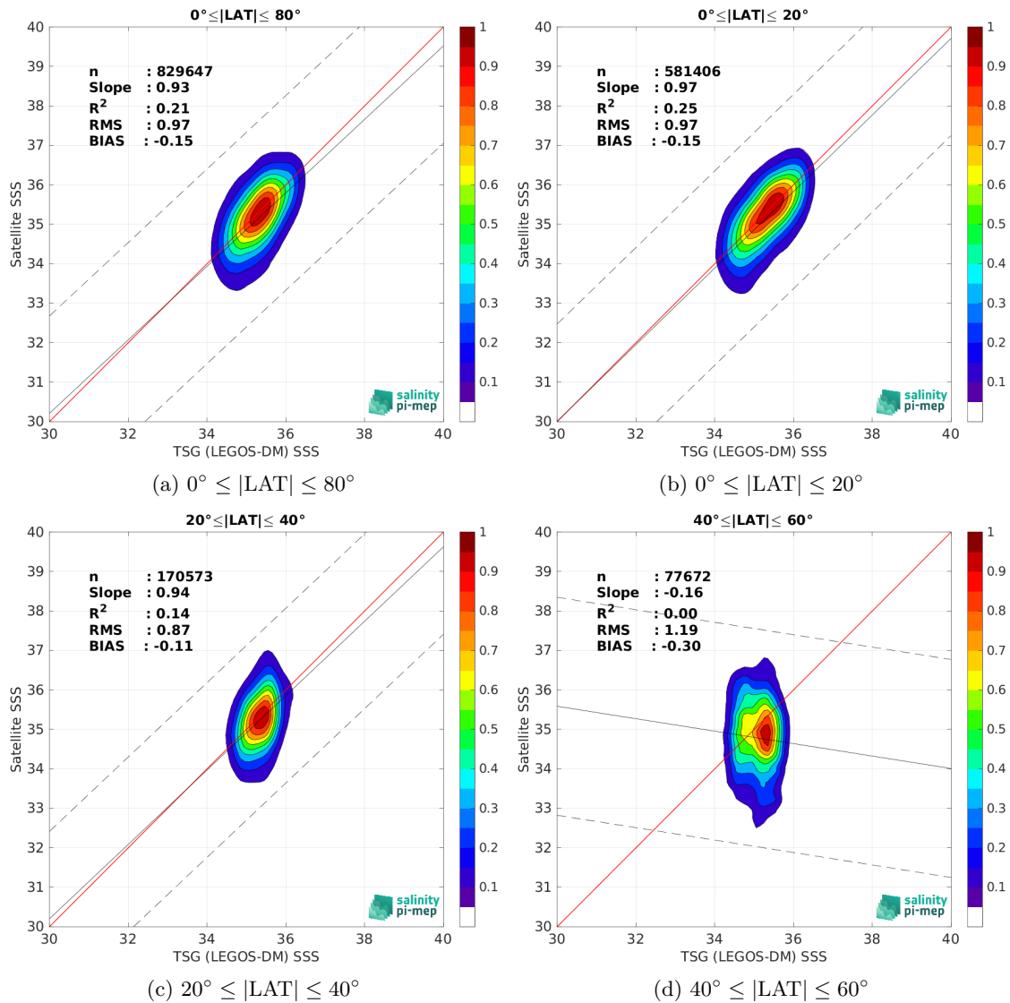
Figure 10: Contour maps of the concentration of SMAP SSS L2 v5.0 (JPL) SSS (y-axis) versus TSG (LEGOS-DM) SSS (x-axis) at match-up pairs for different latitude bands. For each plot, the red line shows x=y . The black thin and dashed lines indicate a linear fit through the data cloud and the \pm 95\% confidence levels, respectively. The number match-up pairs n , the slope and R^2 coefficient of the linear fit, the root mean square (RMS) and the mean bias between satellite and in situ data are indicated for each latitude band in each plots.
