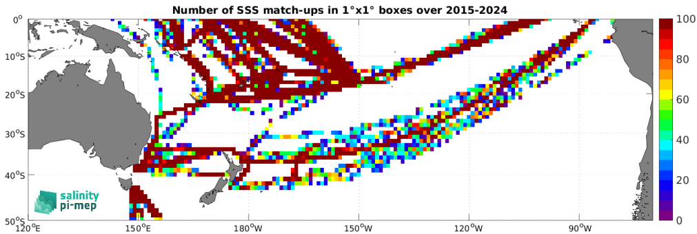
Figure 5: Number of SSS match-ups between TSG (LEGOS-DM) SSS and the SMAP SSS L2 v5.0 (JPL) SSS product for the South Pacific Ocean Pi-MEP region over 1^\circ \times 1^\circ boxes and for the full satellite product period.
