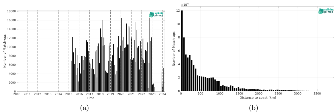
Figure 2: Number of match-ups between TSG (LEGOS-DM) and SMAP SSS L2 v5.0 (JPL) SSS as a function of time (a) and as function of the distance to coast (b) over the South Pacific Ocean Pi-MEP region and for the full satellite product period.
