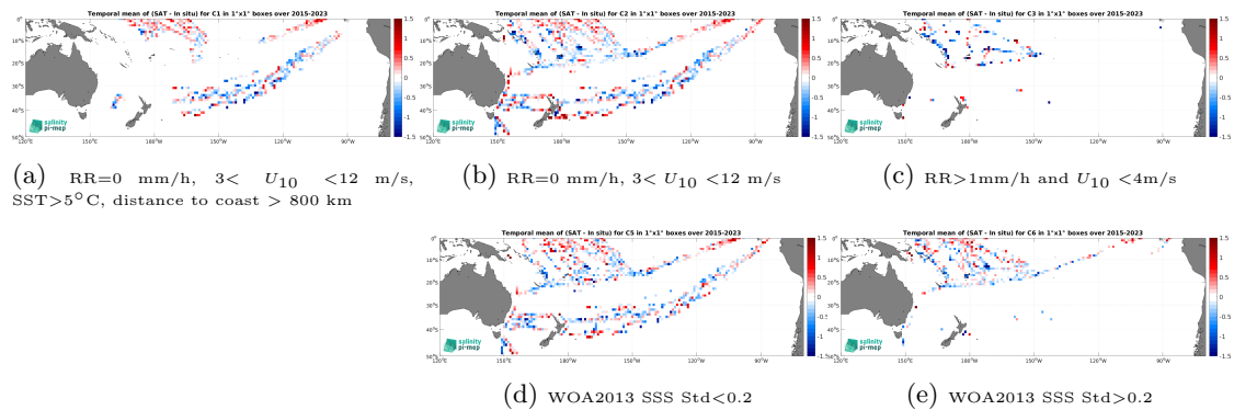
Figure 14: Temporal mean gridded over spatial boxes of size 1^\circ \times 1^\circ of \Delta SSS (SMAP SSS L2 v5.0 (JPL) - TSG (LEGOS-DM)) for 5 different subdatasets corresponding to:RR=0 mm/h, 3 < U_{10} < 12 m/s, SST>5°C, distance to coast > 800 km (a), RR=0 mm/h, 3 < U_{10} < 12 m/s (b), RR>1mm/h and U_{10} < 4 m/s (c), WOA2013 SSS Std<0.2 (d), WOA2013 SSS Std>0.2 (e).
