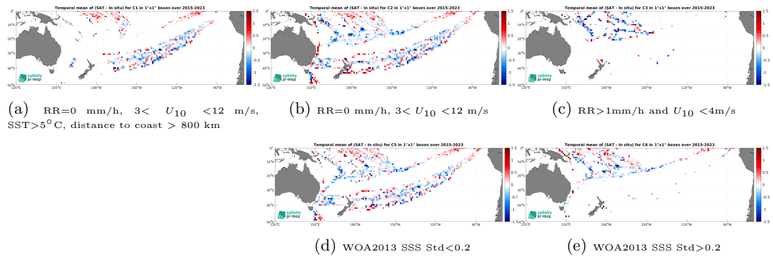
Figure 12: Temporal mean gridded over spatial boxes of size 1^\circ \times 1^\circ of \Delta\text{SSS} (SMAP SSS L2 v5.0 (JPL) - TSG (LEGOS-DM)) for 5 different subdatasets corresponding to:RR=0 mm/h, 3 < U_{10} < 12 m/s, SST >5^\circ\text{C} , distance to coast > 800 km (a), RR=0 mm/h, 3 < U_{10} < 12 m/s (b), RR >1 mm/h and U_{10} < 4 m/s (c), WOA2013 SSS Std <0.2 (d), WOA2013 SSS Std >0.2 (e).
