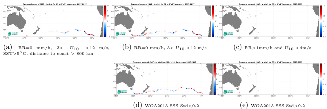
Figure 14: Temporal mean gridded over spatial boxes of size 1^\circ \times 1^\circ of \Delta SSS (SMAP SSS L2 v5.0 (JPL) - TSG (GOSUD-Sailing-ship)) for 5 different subdatasets corresponding to:RR=0 mm/h, 3 < U_{10} < 12 m/s, SST>5°C, distance to coast > 800 km (a), RR=0 mm/h, 3 < U_{10} < 12 m/s (b), RR>1mm/h and U_{10} < 4 m/s (c), WOA2013 SSS Std<0.2 (d), WOA2013 SSS Std>0.2 (e).
