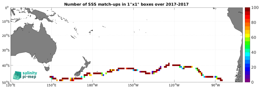
Figure 5: Number of SSS match-ups between TSG (GOSUD-Sailing-ship) SSS and the SMAP SSS L2 v5.0 (JPL) SSS product for the South Pacific Ocean Pi-MEP region over 1^\circ \times 1^\circ boxes and for the full satellite product period.
