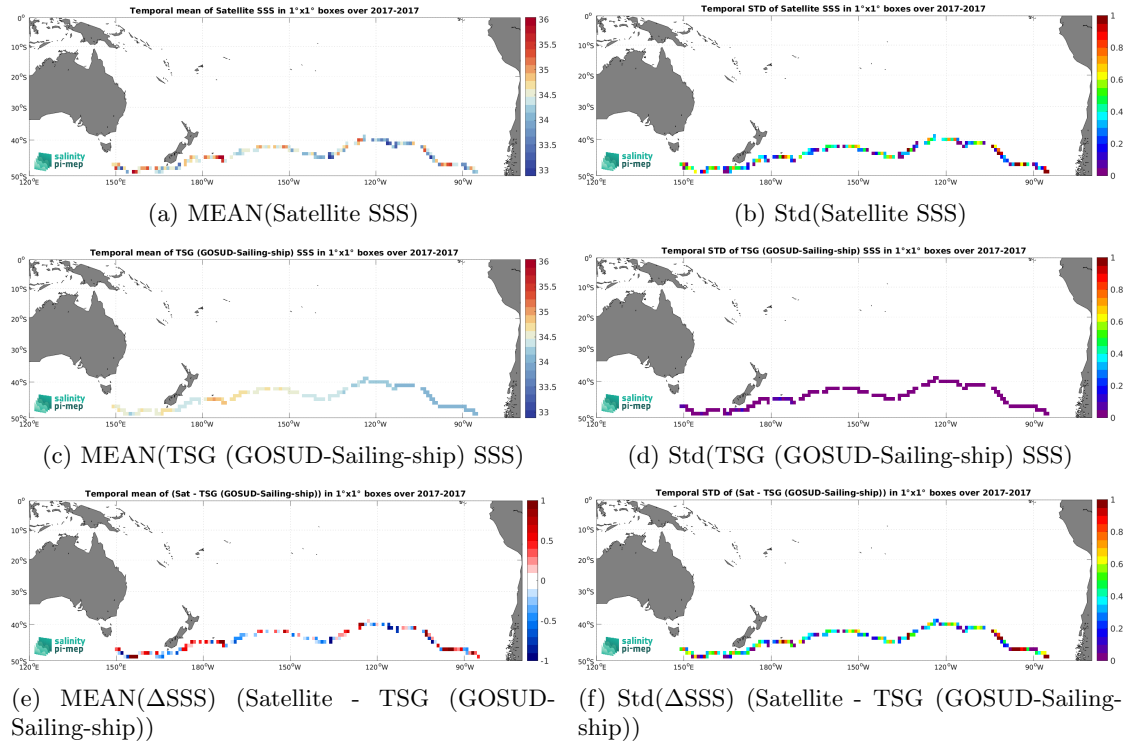
Figure 7: Temporal mean (left) and Std (right) of SSS from SMAP SSS L2 v5.0 (JPL) (top), TSG (GOSUD-Sailing-ship) (middle), and of \Delta SSS (Satellite - TSG (GOSUD-Sailing-ship)). Only match-up pairs are used to generate these maps.
