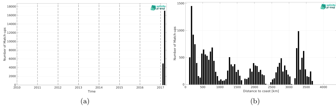
Figure 2: Number of match-ups between TSG (GOSUD-Sailing-ship) and SMAP SSS L2 v5.0 (JPL) SSS as a function of time (a) and as function of the distance to coast (b) over the South Pacific Ocean Pi-MEP region and for the full satellite product period.
