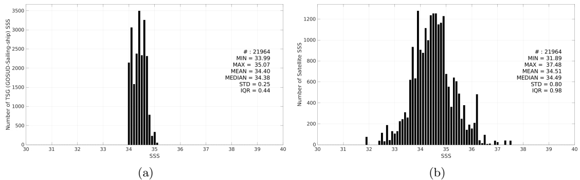
Figure 3: Histograms of SSS from TSG (GOSUD-Sailing-ship) (a) and SMAP SSS L2 v5.0 (JPL) (b) considering all match-up pairs per bins of 0.1 over the South Pacific Ocean Pi-MEP region and for the full satellite product period.
