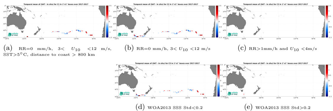
Figure 14: Temporal mean gridded over spatial boxes of size 1^\circ \times 1^\circ of \Delta\text{SSS} (SMAP SSS L2 v5.0 (JPL) - TSG (GOSUD-Sailing-ship)) for 5 different subdatasets corresponding to:RR=0 mm/h, 3 < U_{10} < 12 m/s, SST >5^\circ\text{C} , distance to coast > 800 km (a), RR=0 mm/h, 3 < U_{10} < 12 m/s (b), RR >1 mm/h and U_{10} < 4 m/s (c), WOA2013 SSS Std <0.2 (d), WOA2013 SSS Std >0.2 (e).
