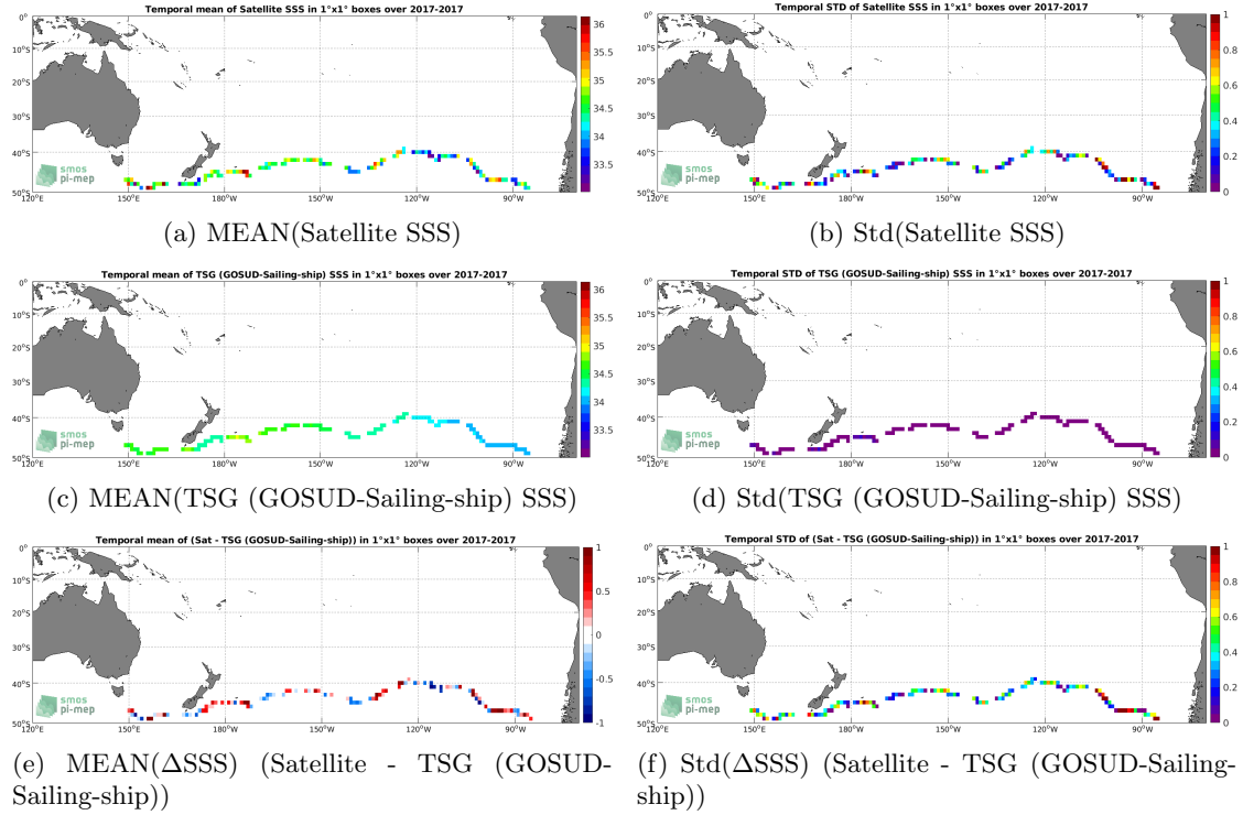
Figure 6: Temporal mean (left) and Std (right) of SSS from SMAP SSS L2 v5.0 (JPL) (top), TSG (GOSUD-Sailing-ship) (middle), and of \Delta SSS (Satellite - TSG (GOSUD-Sailing-ship)). Only match-up pairs are used to generate these maps.
