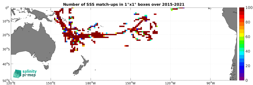
Figure 5: Number of SSS match-ups between TSG (GOSUD-Research-vessel) SSS and the SMAP SSS L2 v5.0 (JPL) SSS product for the South Pacific Ocean Pi-MEP region over 1^\circ \times 1^\circ boxes and for the full satellite product period.
