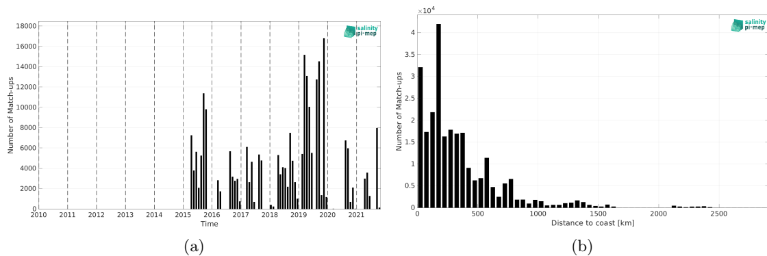
Figure 2: Number of match-ups between TSG (GOSUD-Research-vessel) and SMAP SSS L2 v5.0 (JPL) SSS as a function of time (a) and as function of the distance to coast (b) over the South Pacific Ocean Pi-MEP region and for the full satellite product period.
