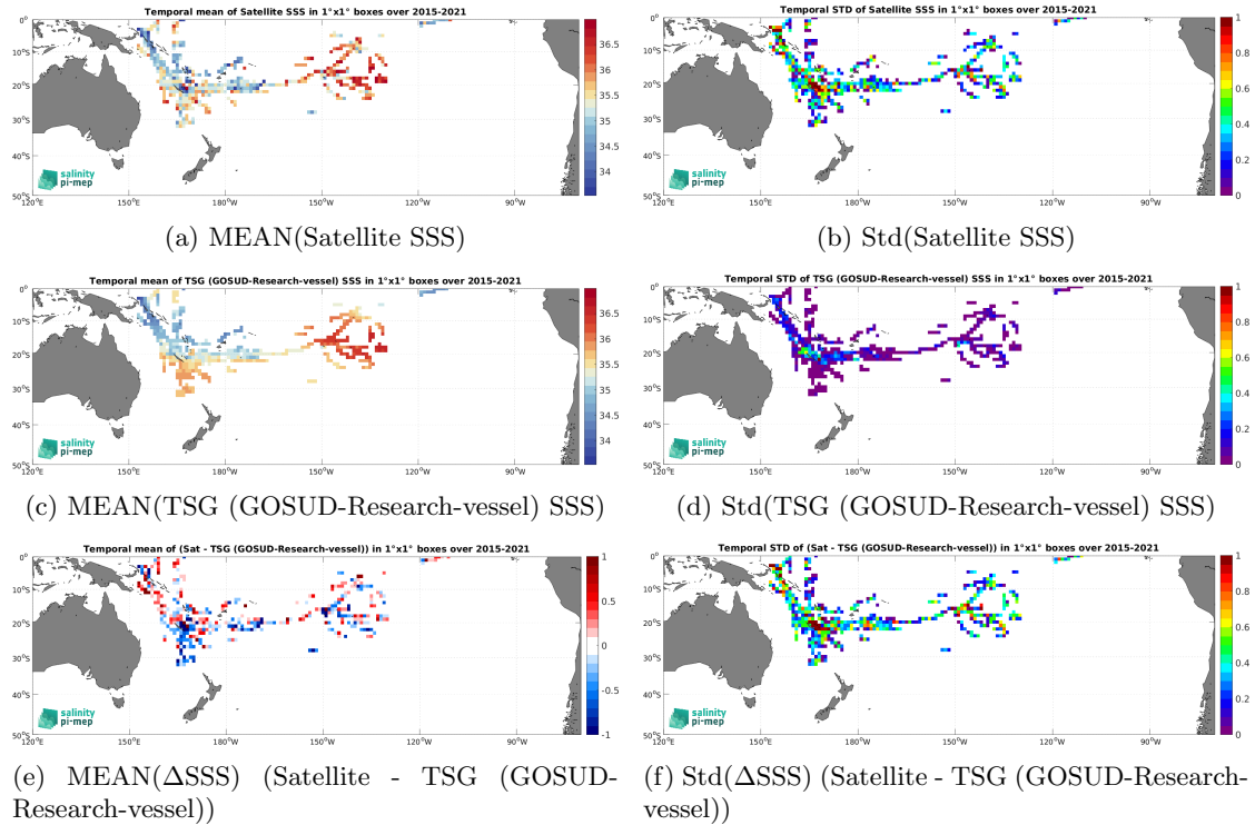
Figure 7: Temporal mean (left) and Std (right) of SSS from SMAP SSS L2 v5.0 (JPL) (top), TSG (GOSUD-Research-vessel) (middle), and of \Delta SSS (Satellite - TSG (GOSUD-Research-vessel)). Only match-up pairs are used to generate these maps.
