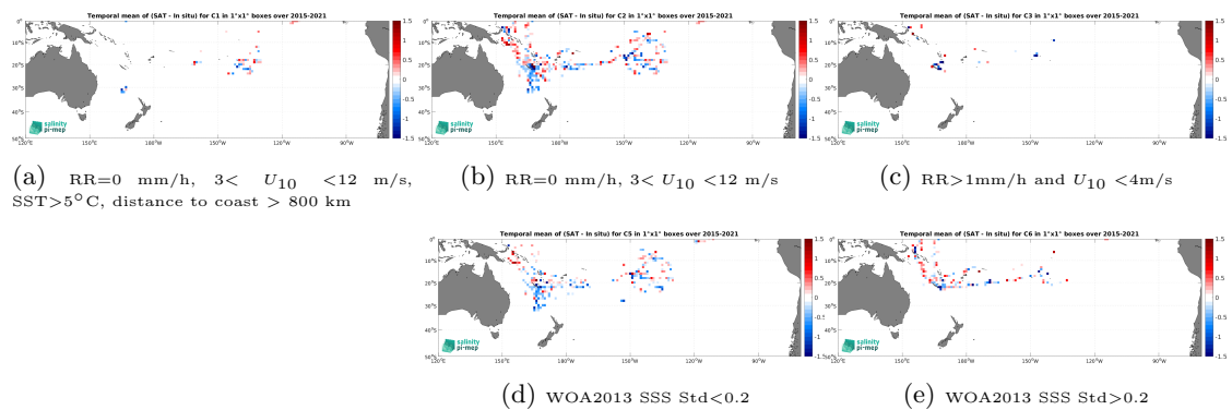
Figure 14: Temporal mean gridded over spatial boxes of size 1^\circ \times 1^\circ of \Delta SSS (SMAP SSS L2 v5.0 (JPL) - TSG (GOSUD-Research-vessel)) for 5 different subdatasets corresponding to:RR=0 mm/h, 3 < U_{10} < 12 m/s, SST >5^\circ\text{C} , distance to coast > 800 km (a), RR=0 mm/h, 3 < U_{10} < 12 m/s (b), RR >1 mm/h and U_{10} < 4 m/s (c), WOA2013 SSS Std <0.2 (d), WOA2013 SSS Std >0.2 (e).
