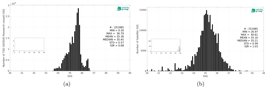
Figure 3: Histograms of SSS from TSG (GOSUD-Research-vessel) (a) and SMAP SSS L2 v5.0 (JPL) (b) considering all match-up pairs per bins of 0.1 over the South Pacific Ocean Pi-MEP region and for the full satellite product period.
