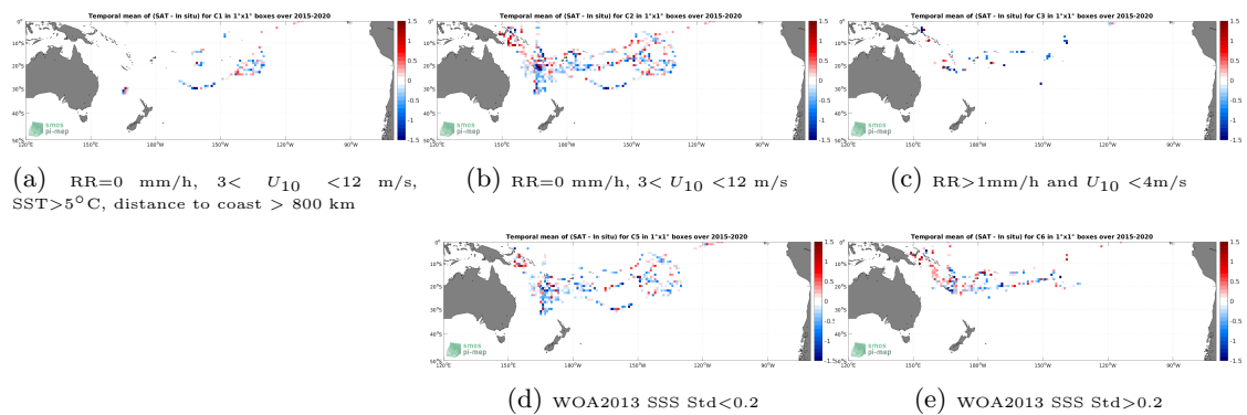
Figure 12: Temporal mean gridded over spatial boxes of size 1^\circ \times 1^\circ of \Delta SSS (SMAP SSS L2 v5.0 (JPL) - TSG (GOSUD-Research-vessel)) for 5 different subdatasets corresponding to:RR=0 mm/h, 3 < U_{10} < 12 m/s, SST >5^\circ\text{C} , distance to coast > 800 km (a), RR=0 mm/h, 3 < U_{10} < 12 m/s (b), RR >1 mm/h and U_{10} < 4 m/s (c), WOA2013 SSS Std <0.2 (d), WOA2013 SSS Std >0.2 (e).
