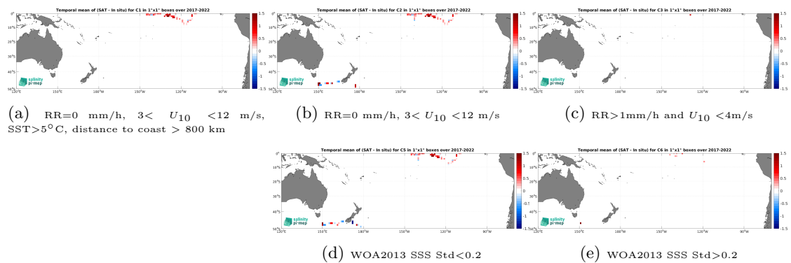
Figure 14: Temporal mean gridded over spatial boxes of size 1^\circ \times 1^\circ of \Delta\text{SSS} (SMAP SSS L2 v5.0 (JPL) - Saildrone) for 5 different subdatasets corresponding to:RR=0 mm/h, 3 < U_{10} < 12 m/s, SST >5^\circ\text{C} , distance to coast > 800 km (a), RR=0 mm/h, 3 < U_{10} < 12 m/s (b), RR >1 mm/h and U_{10} < 4 m/s (c), WOA2013 SSS Std <0.2 (d), WOA2013 SSS Std >0.2 (e).
