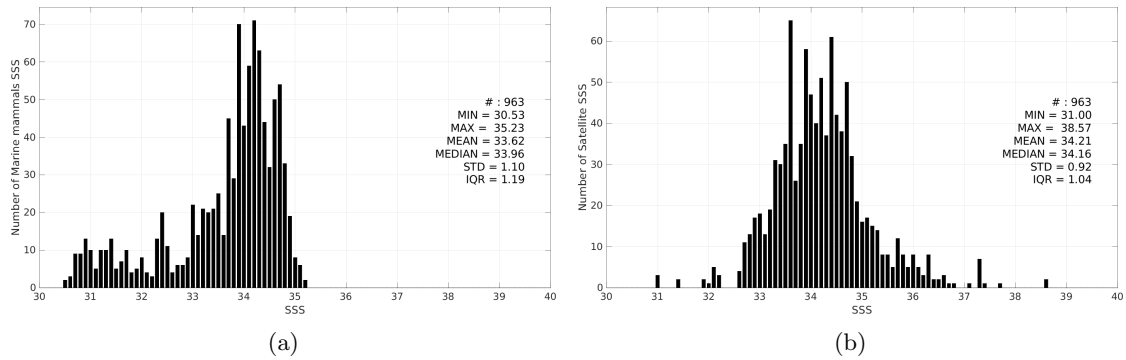
Figure 3: Histograms of SSS from Marine mammals (a) and SMAP SSS L2 v5.0 (JPL) (b) considering all match-up pairs per bins of 0.1 over the South Pacific Ocean Pi-MEP region and for the full satellite product period.
