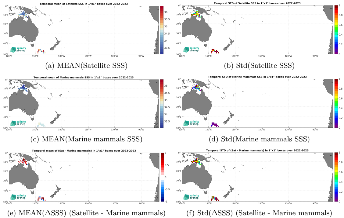
Figure 7: Temporal mean (left) and Std (right) of SSS from SMAP SSS L2 v5.0 (JPL) (top), Marine mammals (middle), and of \Delta SSS (Satellite - Marine mammals). Only match-up pairs are used to generate these maps.
