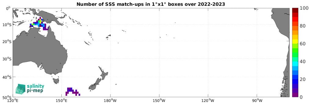
Figure 5: Number of SSS match-ups between Marine mammals SSS and the SMAP SSS L2 v5.0 (JPL) SSS product for the South Pacific Ocean Pi-MEP region over 1^\circ \times 1^\circ boxes and for the full satellite product period.
