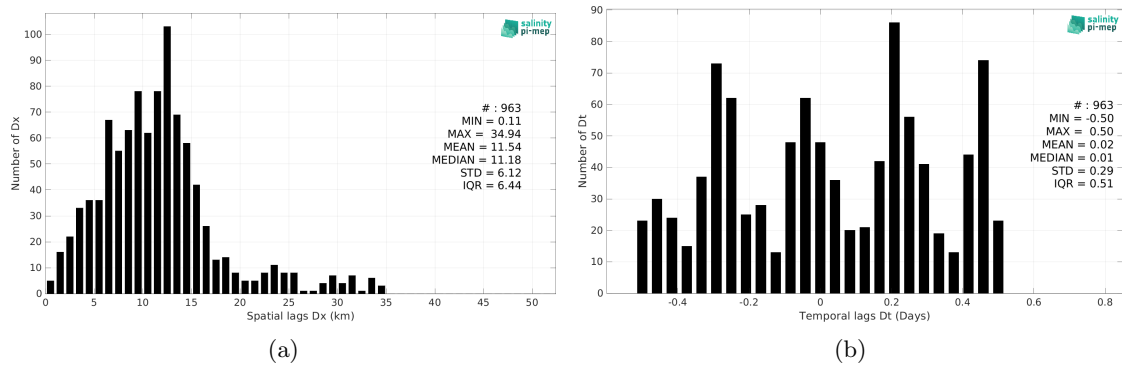
Figure 6: Histograms of the spatial (a) and temporal (b) lags between the location/time of the Marine mammals measurement and the date of the corresponding SMAP SSS L2 v5.0 (JPL) SSS pixel.
