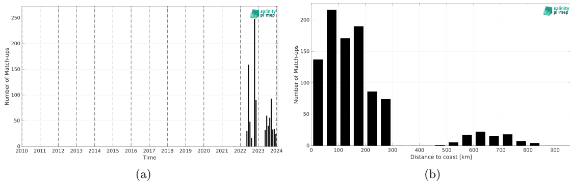
Figure 2: Number of match-ups between Marine mammals and SMAP SSS L2 v5.0 (JPL) SSS as a function of time (a) and as function of the distance to coast (b) over the South Pacific Ocean Pi-MEP region and for the full satellite product period.
