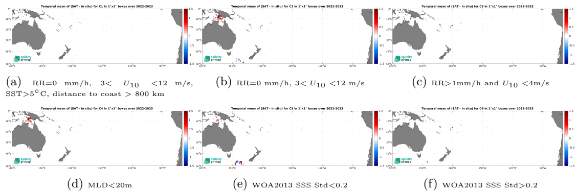
Figure 14: Temporal mean gridded over spatial boxes of size 1^\circ \times 1^\circ of \Delta SSS (SMAP SSS L2 v5.0 (JPL) - Marine mammals) for 6 different subdatasets corresponding to:RR=0 mm/h, 3 < U_{10} < 12 m/s, SST >5^\circ\text{C} , distance to coast > 800 km (a), RR=0 mm/h, 3 < U_{10} < 12 m/s (b), RR >1 mm/h and U_{10} < 4 m/s (c),MLD <20 m (d),WOA2013 SSS Std <0.2 (e),WOA2013 SSS Std >0.2 (f).
