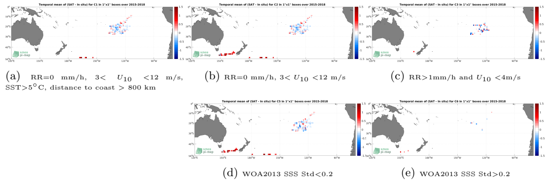
Figure 11: Temporal mean gridded over spatial boxes of size 1^\circ \times 1^\circ of \Delta SSS (SMAP SSS L2 v5.0 (JPL) - Surface drifters) for 5 different subdatasets corresponding to:RR=0 mm/h, 3 < U_{10} < 12 m/s, SST >5^\circ C, distance to coast > 800 km (a), RR=0 mm/h, 3 < U_{10} < 12 m/s (b), RR >1 mm/h and U_{10} < 4 m/s (c), WOA2013 SSS Std <0.2 (d), WOA2013 SSS Std >0.2 (e).
