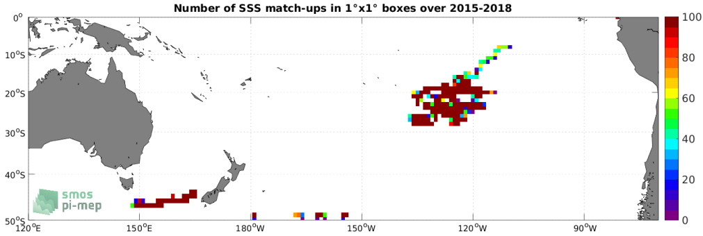
Figure 3: Number of SSS match-ups between Surface drifters SSS and the SMAP SSS L2 v5.0 (JPL) SSS product for the South Pacific Ocean Pi-MEP region over 1^\circ \times 1^\circ boxes and for the full satellite product period.
