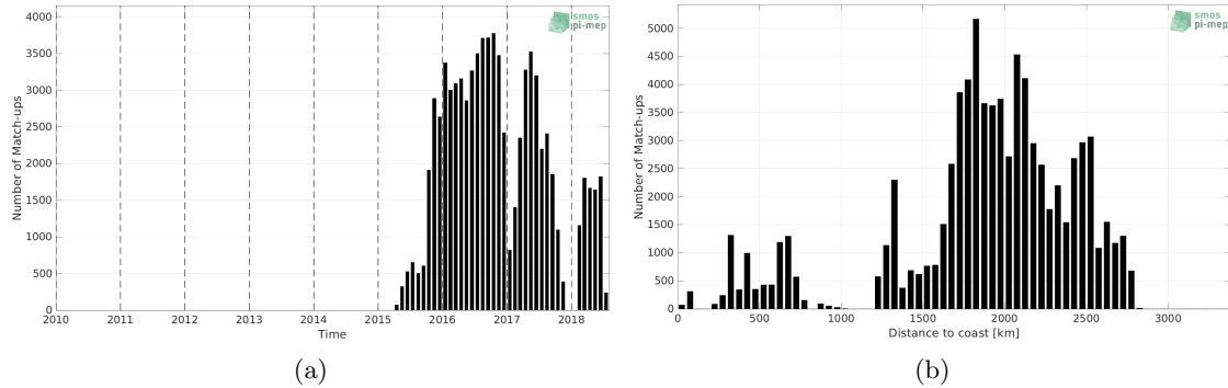
Figure 1: Number of match-ups between Surface drifters and SMAP SSS L2 v5.0 (JPL) SSS as a function of time (a) and as function of the distance to coast (b) over the South Pacific Ocean Pi-MEP region and for the full satellite product period.
