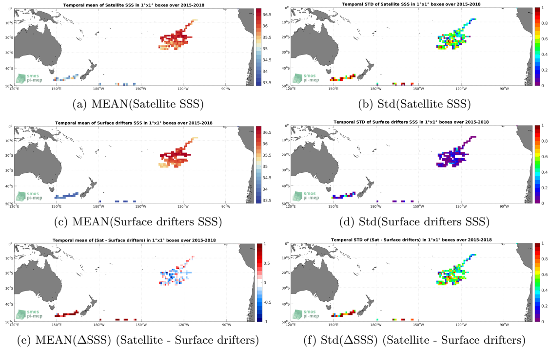
Figure 5: Temporal mean (left) and Std (right) of SSS from SMAP SSS L2 v5.0 (JPL) (top), Surface drifters (middle), and of \Delta SSS (Satellite - Surface drifters). Only match-up pairs are used to generate these maps.
