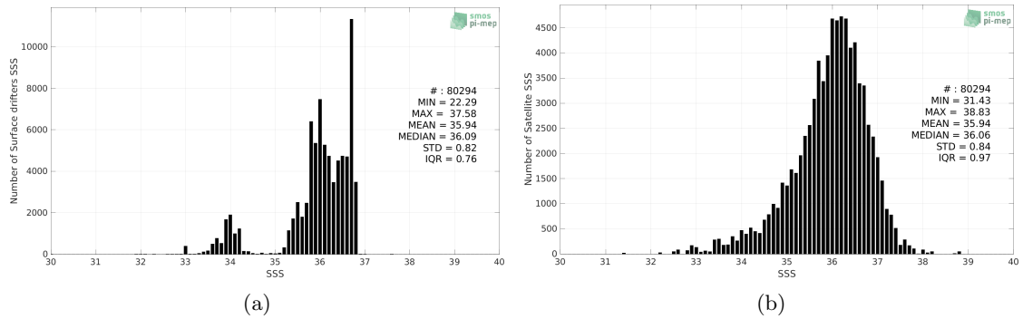
Figure 2: Histograms of SSS from Surface drifters (a) and SMAP SSS L2 v5.0 (JPL) (b) considering all match-up pairs per bins of 0.1 over the South Pacific Ocean Pi-MEP region and for the full satellite product period.
