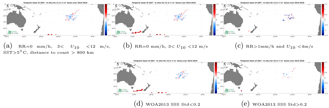
Figure 11: Temporal mean gridded over spatial boxes of size 1^\circ \times 1^\circ of \Delta\text{SSS} (SMAP SSS L2 v5.0 (JPL) - Surface drifters) for 5 different subdatasets corresponding to:RR=0 mm/h, 3 < U_{10} < 12 m/s, SST >5^\circ\text{C} , distance to coast > 800 km (a), RR=0 mm/h, 3 < U_{10} < 12 m/s (b), RR >1 mm/h and U_{10} < 4 m/s (c), WOA2013 SSS Std <0.2 (d), WOA2013 SSS Std >0.2 (e).
