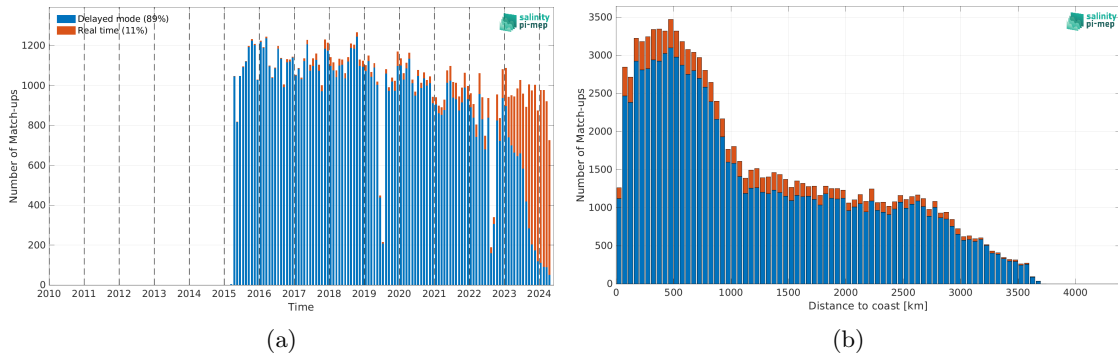
Figure 2: Number of match-ups between Argo and SMAP SSS L2 v5.0 (JPL) SSS as a function of time (a) and as function of the distance to coast (b) over the South Pacific Ocean Pi-MEP region and for the full satellite product period.
