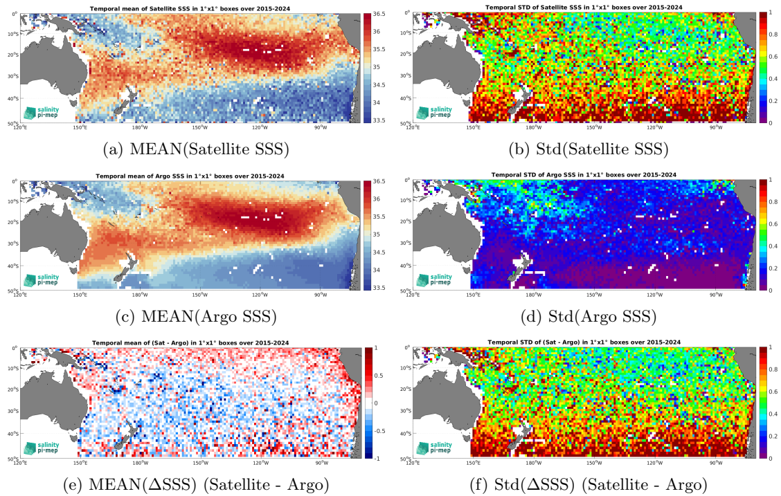
Figure 7: Temporal mean (left) and Std (right) of SSS from SMAP SSS L2 v5.0 (JPL) (top), Argo (middle), and of \Delta SSS (Satellite - Argo). Only match-up pairs are used to generate these maps.
