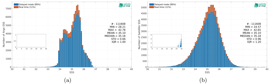
Figure 3: Histograms of SSS from Argo (a) and SMAP SSS L2 v5.0 (JPL) (b) considering all match-up pairs per bins of 0.1 over the South Pacific Ocean Pi-MEP region and for the full satellite product period.
