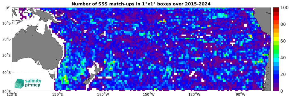
Figure 5: Number of SSS match-ups between Argo SSS and the SMAP SSS L2 v5.0 (JPL) SSS product for the South Pacific Ocean Pi-MEP region over 1^\circ \times 1^\circ boxes and for the full satellite product period.
