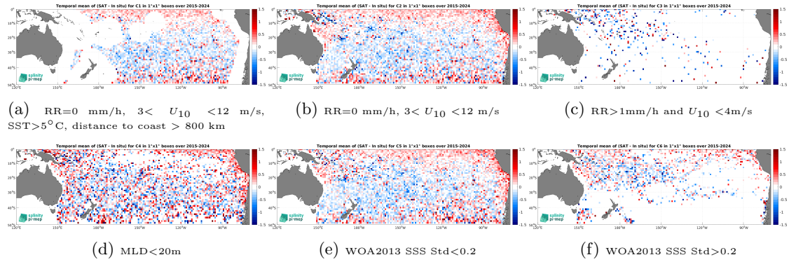
Figure 14: Temporal mean gridded over spatial boxes of size 1^\circ \times 1^\circ of \Delta SSS (SMAP SSS L2 v5.0 (JPL) - Argo) for 6 different subdatasets corresponding to:RR=0 mm/h, 3 < U_{10} < 12 m/s, SST>5°C, distance to coast > 800 km (a), RR=0 mm/h, 3 < U_{10} < 12 m/s (b), RR>1mm/h and U_{10} < 4 m/s (c),MLD<20m (d),WOA2013 SSS Std<0.2 (e),WOA2013 SSS Std>0.2 (f).
