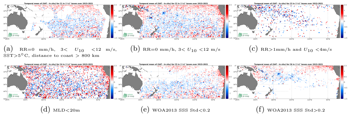
Figure 12: Temporal mean gridded over spatial boxes of size 1^\circ \times 1^\circ of \Delta SSS (SMAP SSS L2 v5.0 (JPL) - Argo) for 6 different subdatasets corresponding to:RR=0 mm/h, 3 < U_{10} < 12 m/s, SST>5°C, distance to coast > 800 km (a), RR=0 mm/h, 3 < U_{10} < 12 m/s (b), RR>1mm/h and U_{10} < 4 m/s (c),MLD<20m (d),WOA2013 SSS Std<0.2 (e),WOA2013 SSS Std>0.2 (f).
