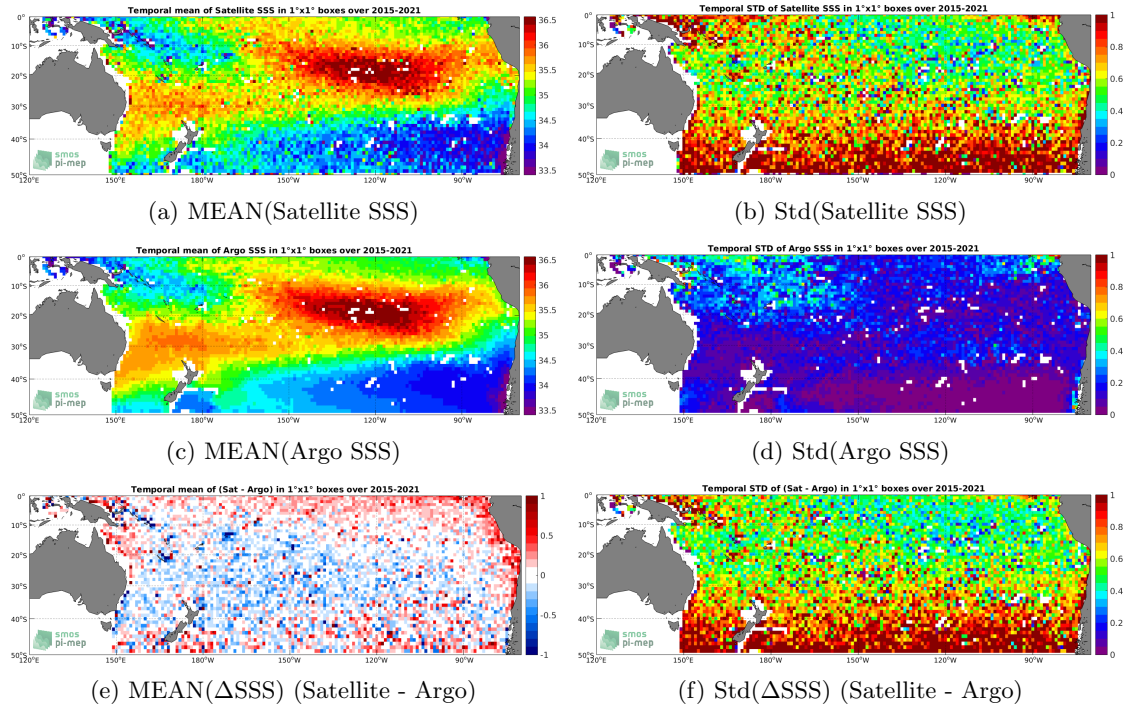
Figure 6: Temporal mean (left) and Std (right) of SSS from SMAP SSS L2 v5.0 (JPL) (top), Argo (middle), and of \Delta SSS (Satellite - Argo). Only match-up pairs are used to generate these maps.
