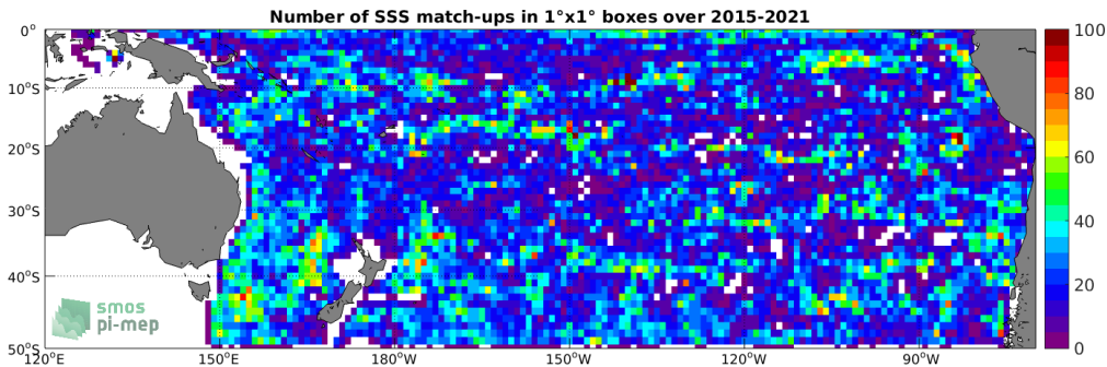
Figure 4: Number of SSS match-ups between Argo SSS and the SMAP SSS L2 v5.0 (JPL) SSS product for the South Pacific Ocean Pi-MEP region over 1^\circ \times 1^\circ boxes and for the full satellite product period.
