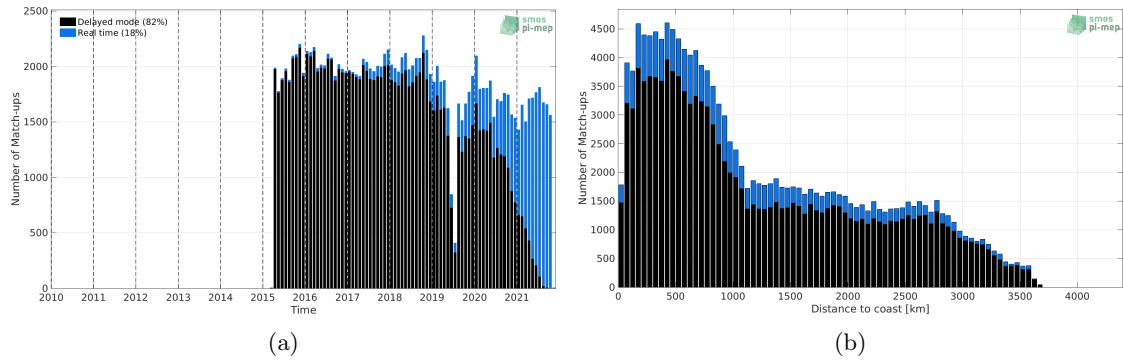
Figure 1: Number of match-ups between Argo and SMAP SSS L2 v5.0 (JPL) SSS as a function of time (a) and as function of the distance to coast (b) over the South Pacific Ocean Pi-MEP region and for the full satellite product period.
