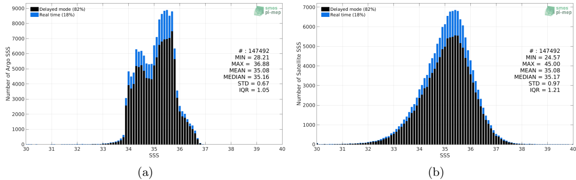
Figure 2: Histograms of SSS from Argo (a) and SMAP SSS L2 v5.0 (JPL) (b) considering all match-up pairs per bins of 0.1 over the South Pacific Ocean Pi-MEP region and for the full satellite product period.
