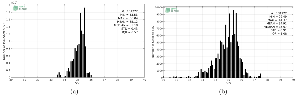
Figure 2: Histograms of SSS from TSG-SAMOS (a) and SMAP-L2-JPL-V4 (b) considering all match-up pairs per bins of 0.1 over the South Pacific Ocean Pi-MEP region and for the full satellite product period.
