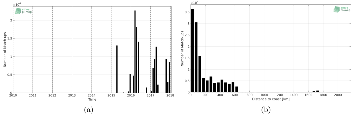
Figure 1: Number of match-ups between TSG-SAMOS and SMAP-L2-JPL-V4 SSS as a function of time (a) and as function of the distance to coast (b) over the South Pacific Ocean Pi-MEP region and for the full satellite product period.
