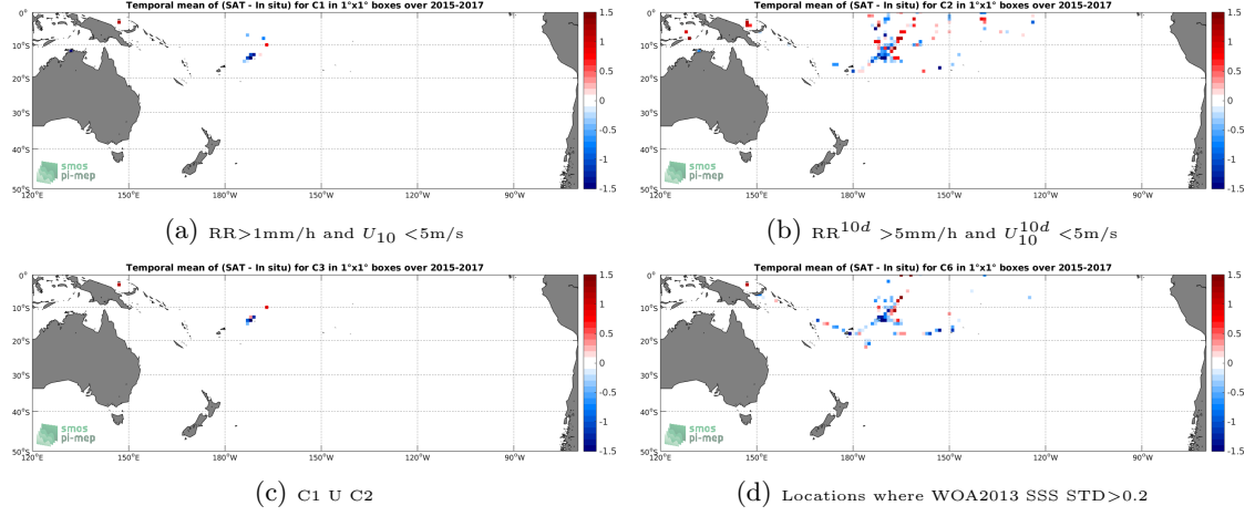
Figure 12: Temporal mean gridded over spatial boxes of size 1^\circ \times 1^\circ of \Delta SSS (SMAP-L2-JPL-V4 - TSG-SAMOS) for 4 different subdatasets corresponding to: RR > 1mm/h and U_{10} < 5\text{m/s} (a), RR^{10d} > 5\text{mm/h} and U_{10}^{10d} < 5\text{m/s} (b), C1 U C2 (c), Locations where WOA2013 SSS STD > 0.2 (d).
