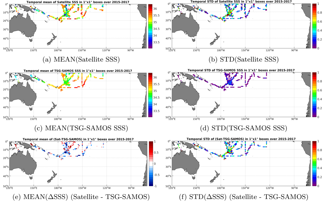
Figure 6: Temporal mean (left) and STD (right) of SSS from SMAP-L2-JPL-V4 (top), TSG-SAMOS (middle), and of \Delta SSS (Satellite - TSG-SAMOS). Only match-up pairs are used to generate these maps.
