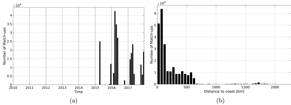
Figure 1: Number of match-ups between TSG-SAMOS and SMAP-L2-JPL-V4 SSS as a function of time (a) and as function of the distance to coast (b) over the South Pacific Ocean Pi-MEP region and for the full satellite product period.
