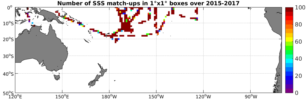
Figure 4: Number of SSS match-ups between TSG-SAMOS SSS and the SMAP-L2-JPL-V4 SSS product for the South Pacific Ocean Pi-MEP region over 1^\circ \times 1^\circ boxes and for the full satellite product period.
