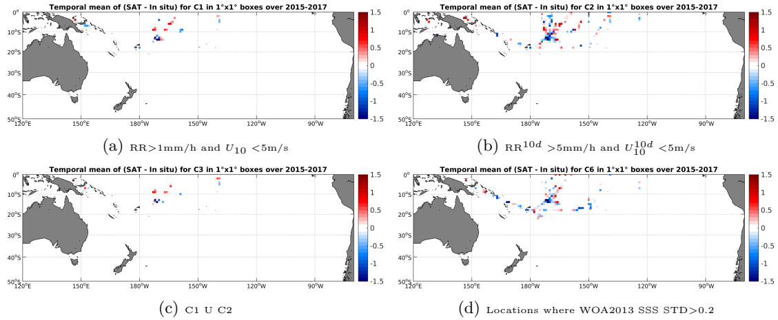
Figure 12: Temporal mean gridded over spatial boxes of size 1^\circ \times 1^\circ of \Delta SSS (SMAP-L2-JPL-V4 - TSG-SAMOS) for 4 different subdatasets corresponding to: RR > 1mm/h and U_{10} < 5 m/s (a), RR^{10d} > 5 mm/h and U_{10}^{10d} < 5 m/s (b), C1 U C2 (c), Locations where WOA2013 SSS STD > 0.2 (d).
