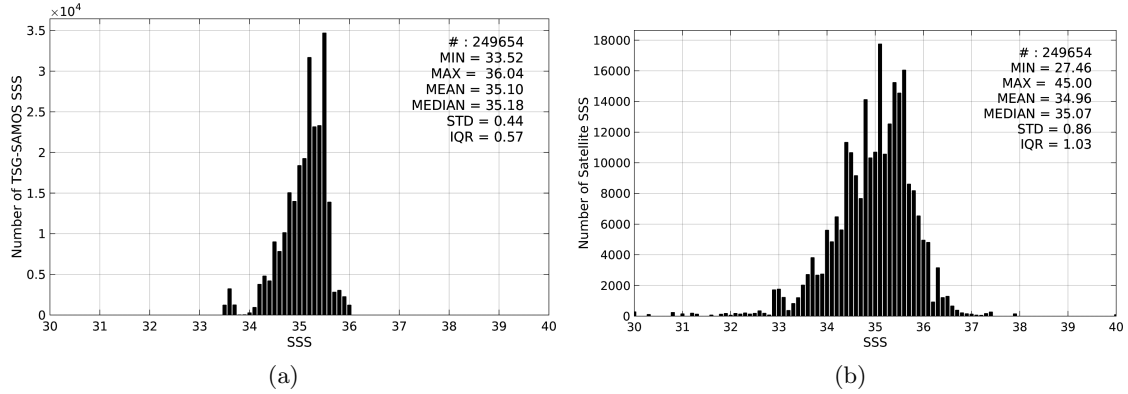
Figure 2: Histograms of SSS from TSG-SAMOS (a) and SMAP-L2-JPL-V4 (b) considering all match-up pairs per bins of 0.1 over the South Pacific Ocean Pi-MEP region and for the full satellite product period.
