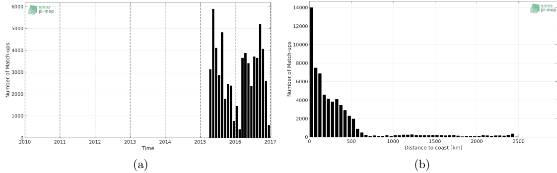
Figure 1: Number of match-ups between TSG-LEGOS-DM and SMAP-L2-JPL-V4 SSS as a function of time (a) and as function of the distance to coast (b) over the South Pacific Ocean Pi-MEP region and for the full satellite product period.
