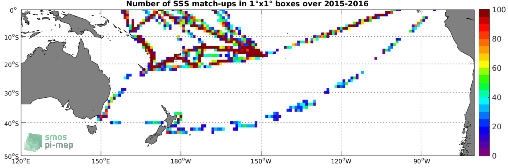
Figure 4: Number of SSS match-ups between TSG-LEGOS-DM SSS and the SMAP-L2-JPL-V4 SSS product for the South Pacific Ocean Pi-MEP region over 1^\circ \times 1^\circ boxes and for the full satellite product period.
