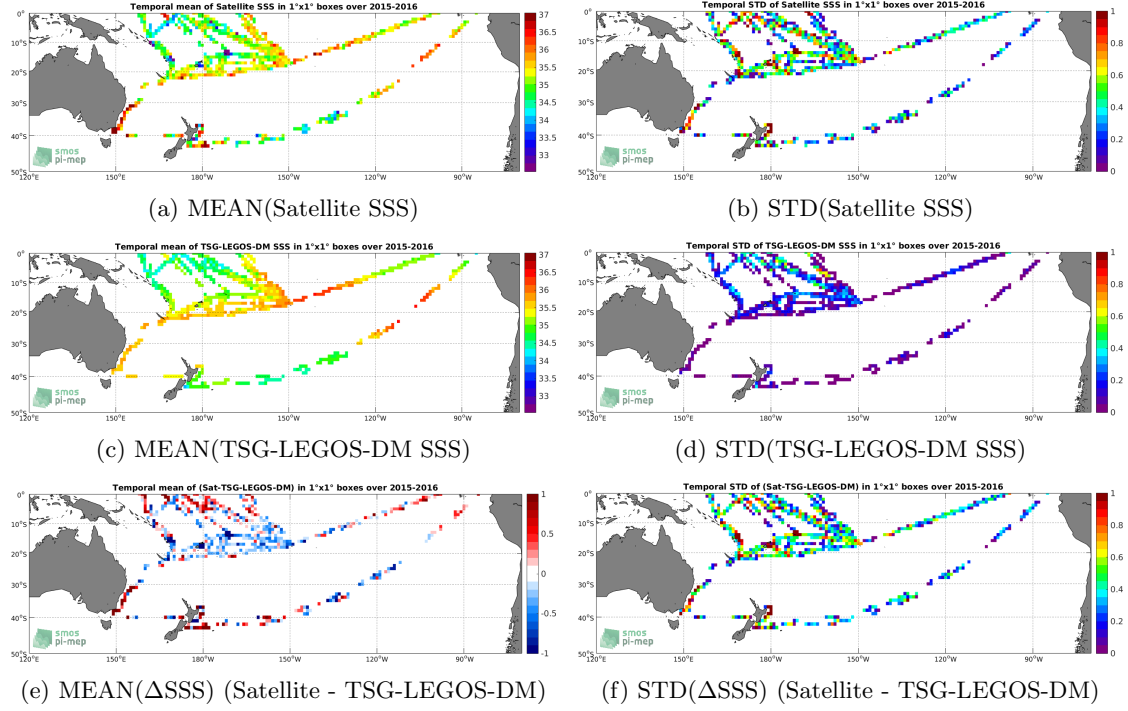
Figure 6: Temporal mean (left) and STD (right) of SSS from SMAP-L2-JPL-V4 (top), TSG-LEGOS-DM (middle), and of \Delta SSS (Satellite - TSG-LEGOS-DM). Only match-up pairs are used to generate these maps.
