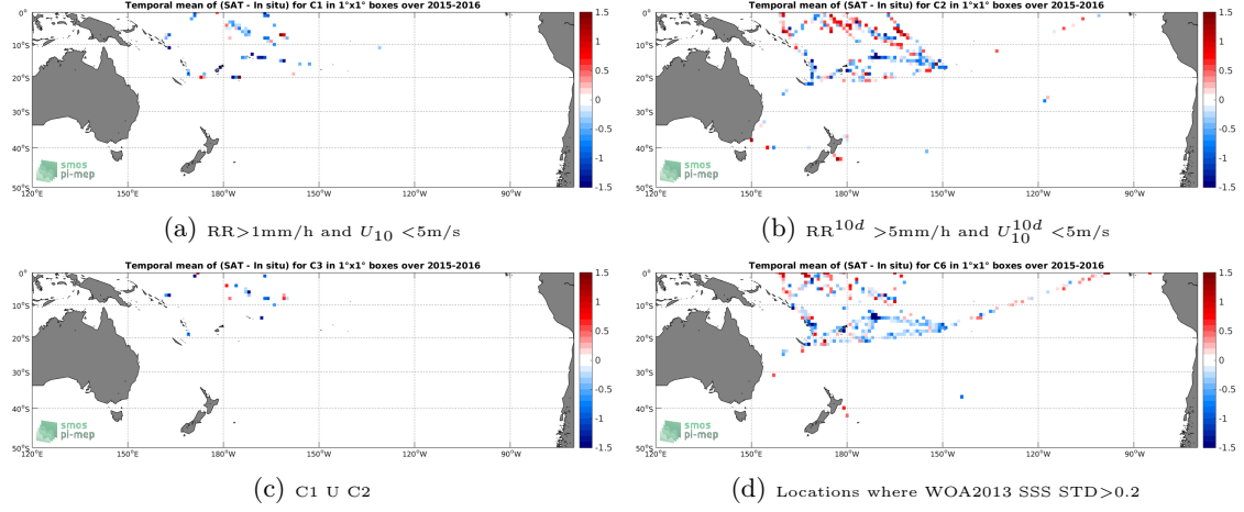
Figure 12: Temporal mean gridded over spatial boxes of size 1^\circ \times 1^\circ of \Delta SSS (SMAP-L2-JPL-V4 - TSG-LEGOS-DM) for 4 different subdatasets corresponding to: RR > 1\text{mm/h} and U_{10} < 5\text{m/s} (a), RR^{10d} > 5\text{mm/h} and U_{10}^{10d} < 5\text{m/s} (b), C1 U C2 (c), Locations where WOA2013 SSS STD > 0.2 (d).
