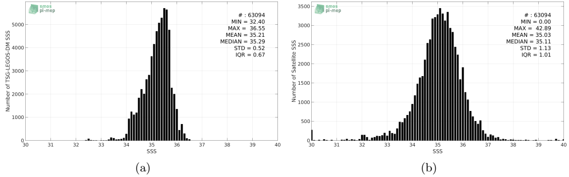
Figure 2: Histograms of SSS from TSG-LEGOS-DM (a) and SMAP-L2-JPL-V4 (b) considering all match-up pairs per bins of 0.1 over the South Pacific Ocean Pi-MEP region and for the full satellite product period.
