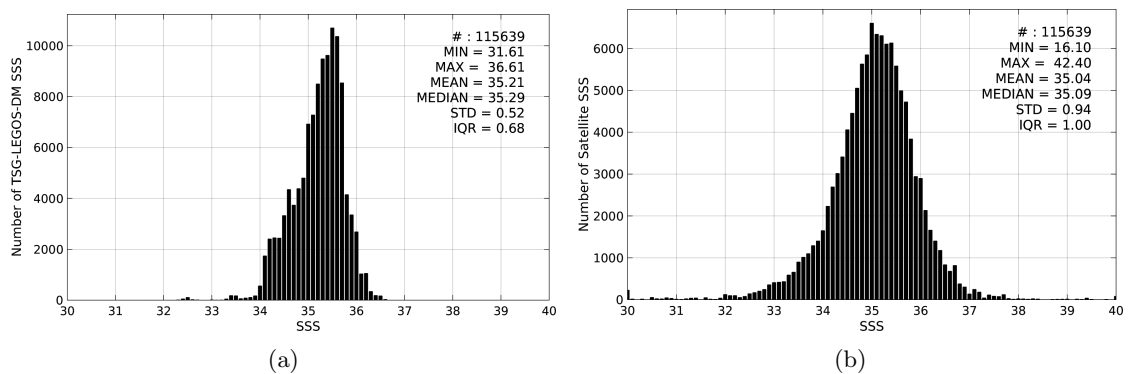
Figure 2: Histograms of SSS from TSG-LEGOS-DM (a) and SMAP-L2-JPL-V4 (b) considering all match-up pairs per bins of 0.1 over the South Pacific Ocean Pi-MEP region and for the full satellite product period.
