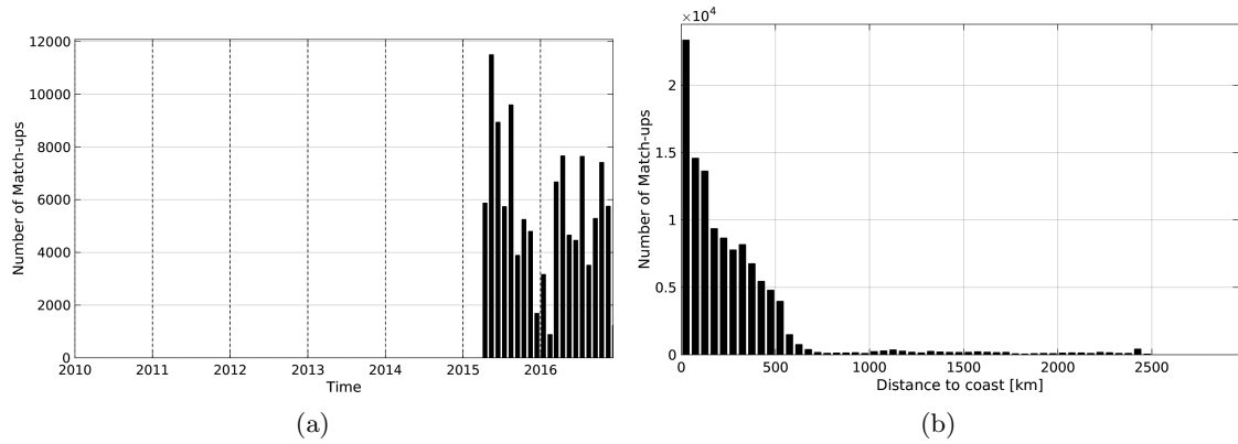
Figure 1: Number of match-ups between TSG-LEGOS-DM and SMAP-L2-JPL-V4 SSS as a function of time (a) and as function of the distance to coast (b) over the South Pacific Ocean Pi-MEP region and for the full satellite product period.
