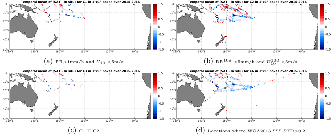
Figure 12: Temporal mean gridded over spatial boxes of size 1^\circ \times 1^\circ of \Delta SSS (SMAP-L2-JPL-V4 - TSG-LEGOS-DM) for 4 different subdatasets corresponding to: RR > 1mm/h and U_{10} < 5 m/s (a), RR^{10d} > 5 mm/h and U_{10}^{10d} < 5 m/s (b), C1 U C2 (c), Locations where WOA2013 SSS STD > 0.2 (d).
