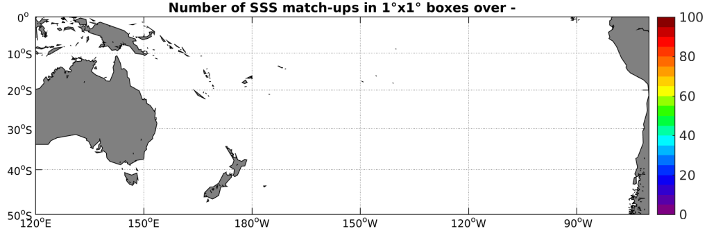
Figure 4: Number of SSS match-ups between TSG-GOSUD-Sailing-ship SSS and the SMAP-L2-JPL-V4 SSS product for the South Pacific Ocean Pi-MEP region over 1^\circ \times 1^\circ boxes and for the full satellite product period.
