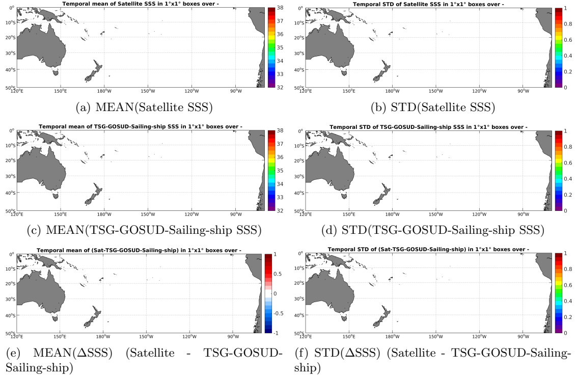
Figure 6: Temporal mean (left) and STD (right) of SSS from SMAP-L2-JPL-V4 (top), TSG-GOSUD-Sailing-ship (middle), and of \Delta SSS (Satellite - TSG-GOSUD-Sailing-ship). Only match-up pairs are used to generate these maps.
