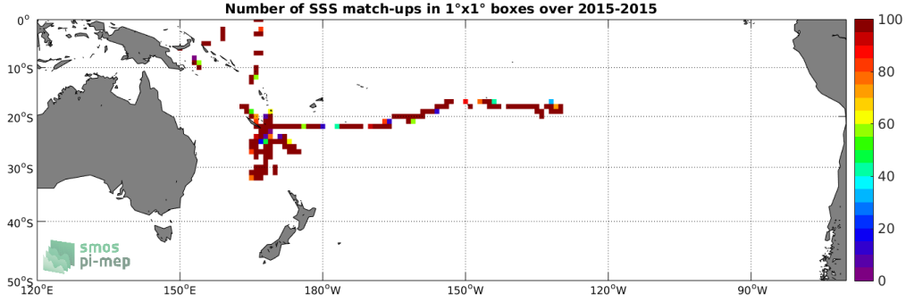
Figure 4: Number of SSS match-ups between TSG-GOSUD-Research-vessel SSS and the SMAP-L2-JPL-V4 SSS product for the South Pacific Ocean Pi-MEP region over 1^\circ \times 1^\circ boxes and for the full satellite product period.
