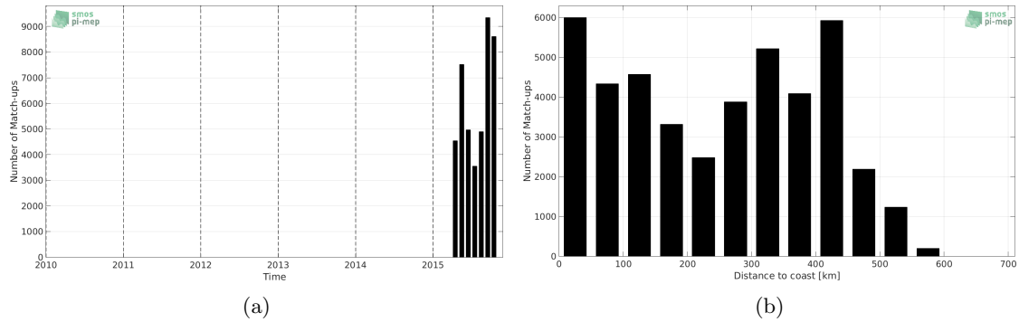
Figure 1: Number of match-ups between TSG-GOSUD-Research-vessel and SMAP-L2-JPL-V4 SSS as a function of time (a) and as function of the distance to coast (b) over the South Pacific Ocean Pi-MEP region and for the full satellite product period.
