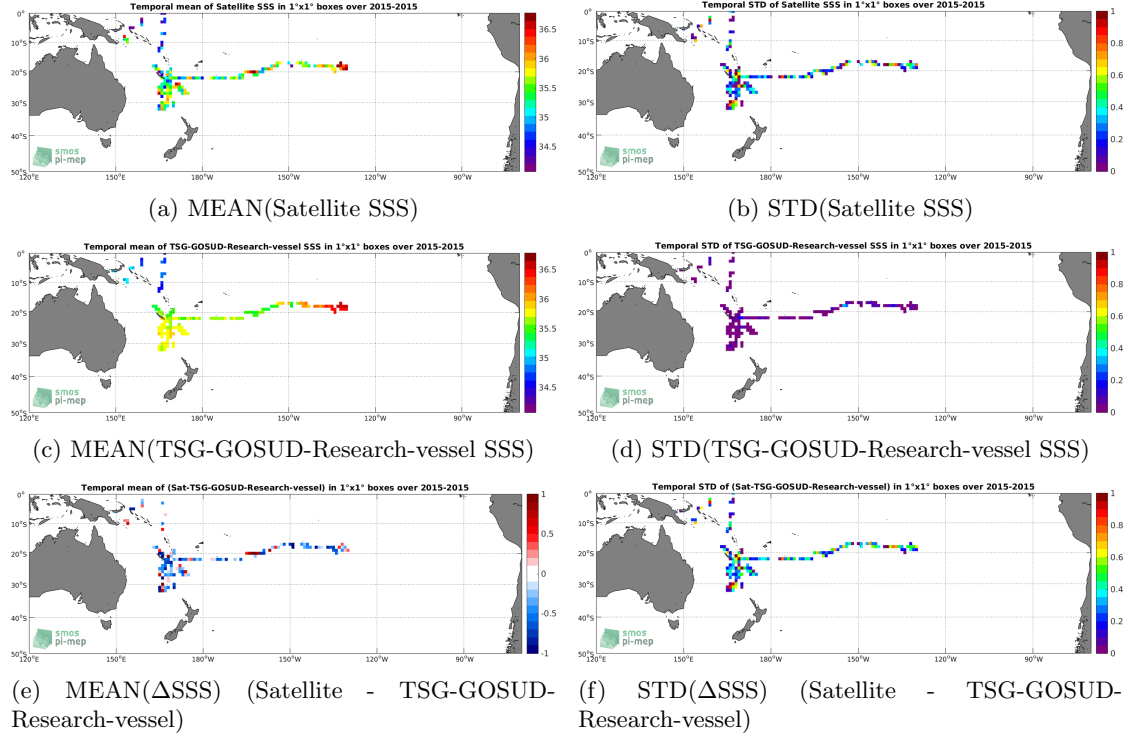
Figure 6: Temporal mean (left) and STD (right) of SSS from SMAP-L2-JPL-V4 (top), TSG-GOSUD-Research-vessel (middle), and of \Delta SSS (Satellite - TSG-GOSUD-Research-vessel). Only match-up pairs are used to generate these maps.
