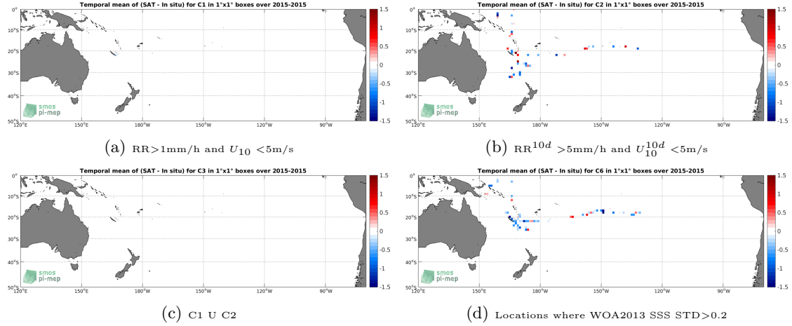
Figure 12: Temporal mean gridded over spatial boxes of size 1^\circ \times 1^\circ of \Delta SSS (SMAP-L2-JPL-V4 - TSG-GOSUD-Research-vessel) for 4 different subdatasets corresponding to: RR > 1\text{mm/h} and U_{10} < 5\text{m/s} (a), RR^{10d} > 5\text{mm/h} and U_{10}^{10d} < 5\text{m/s} (b), C1 U C2 (c), Locations where WOA2013 SSS STD > 0.2 (d).
