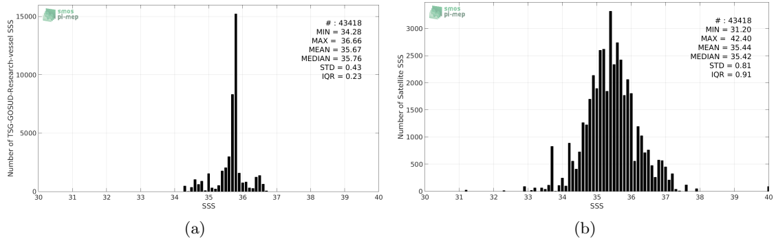
Figure 2: Histograms of SSS from TSG-GOSUD-Research-vessel (a) and SMAP-L2-JPL-V4 (b) considering all match-up pairs per bins of 0.1 over the South Pacific Ocean Pi-MEP region and for the full satellite product period.
