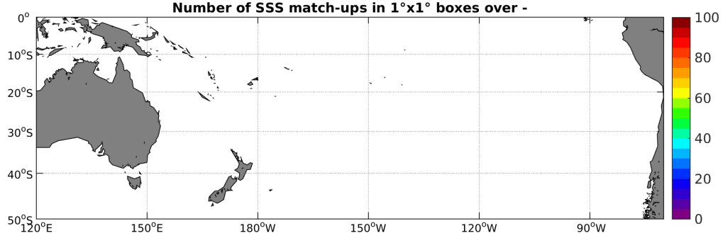
Figure 4: Number of SSS match-ups between Sea mammals SSS and the SMAP-L2-JPL-V4 SSS product for the South Pacific Ocean Pi-MEP region over 1^\circ \times 1^\circ boxes and for the full satellite product period.
