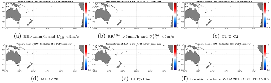
Figure 12: Temporal mean gridded over spatial boxes of size 1^\circ \times 1^\circ of \Delta SSS (SMAP-L2-JPL-V4 - Sea mammals) for 6 different subdatasets corresponding to: RR > 1\text{mm/h} and U_{10} < 5\text{m/s} (a), RR^{10d} > 5\text{mm/h} and U_{10}^{10d} < 5\text{m/s} (b), C1 U C2 (c), MLD < 20\text{m} (d), BLT > 10\text{m} (e), Locations where WOA2013 SSS STD > 0.2 (f).
