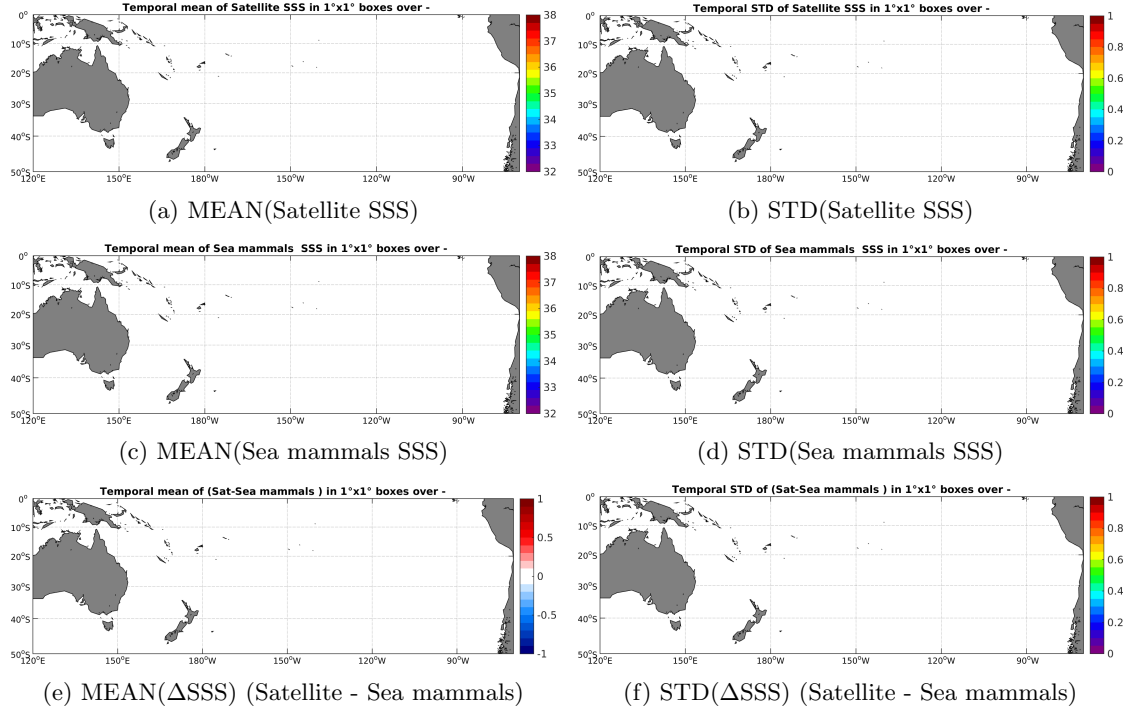
Figure 6: Temporal mean (left) and STD (right) of SSS from SMAP-L2-JPL-V4 (top), Sea mammals (middle), and of \Delta SSS (Satellite - Sea mammals). Only match-up pairs are used to generate these maps.
