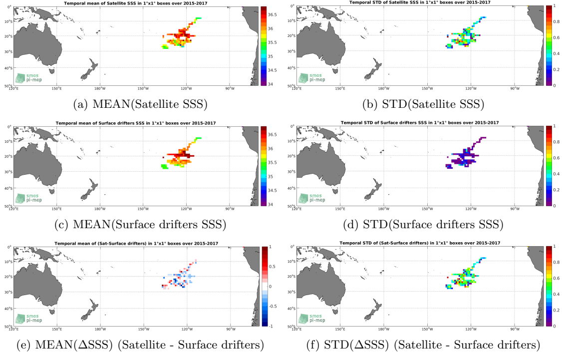
Figure 5: Temporal mean (left) and STD (right) of SSS from SMAP-L2-JPL-V4 (top), Surface drifters (middle), and of \Delta SSS (Satellite - Surface drifters). Only match-up pairs are used to generate these maps.
