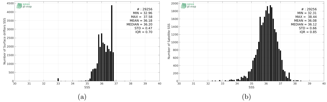
Figure 2: Histograms of SSS from Surface drifters (a) and SMAP-L2-JPL-V4 (b) considering all match-up pairs per bins of 0.1 over the South Pacific Ocean Pi-MEP region and for the full satellite product period.
