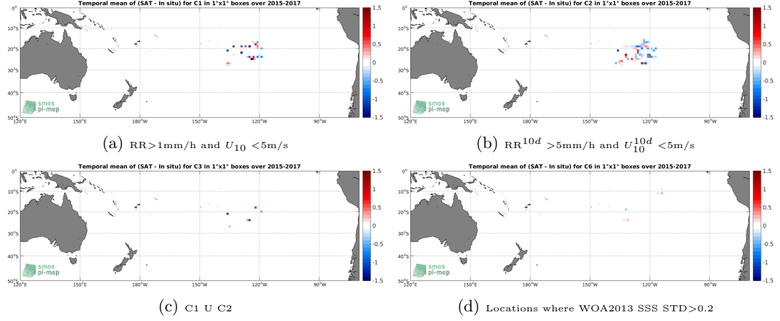
Figure 11: Temporal mean gridded over spatial boxes of size 1^\circ \times 1^\circ of \Delta SSS (SMAP-L2-JPL-V4 - Surface drifters) for 4 different subdatasets corresponding to: RR > 1 mm/h and U_{10} < 5 m/s (a), RR^{10d} > 5 mm/h and U_{10}^{10d} < 5 m/s (b), C1 U C2 (c), Locations where WOA2013 SSS STD > 0.2 (d).
