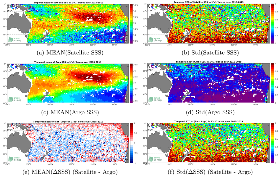
Figure 6: Temporal mean (left) and Std (right) of SSS from SMAP-L2-JPL-V4.3 (top), Argo (middle), and of \Delta SSS (Satellite - Argo). Only match-up pairs are used to generate these maps.
