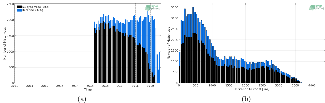
Figure 1: Number of match-ups between Argo and SMAP-L2-JPL-V4.3 SSS as a function of time (a) and as function of the distance to coast (b) over the South Pacific Ocean Pi-MEP region and for the full satellite product period.
