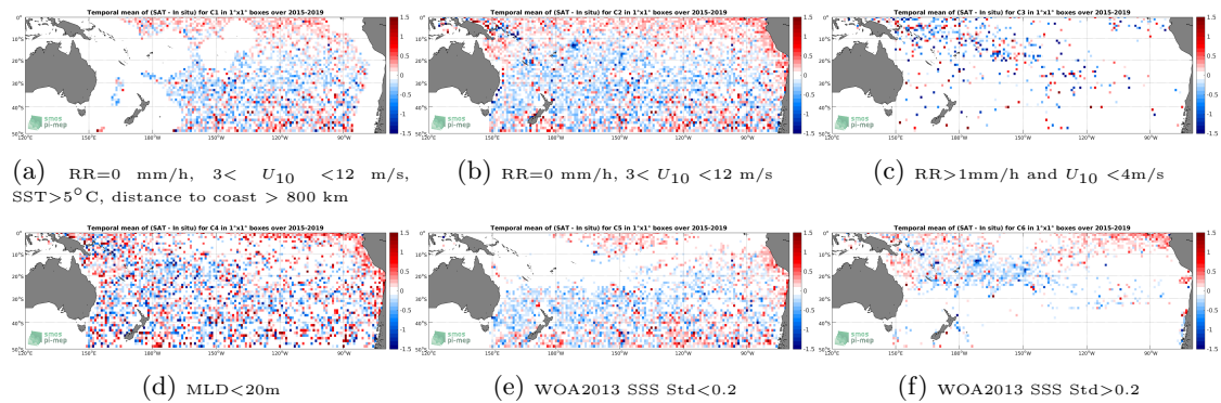
Figure 12: Temporal mean gridded over spatial boxes of size 1^\circ \times 1^\circ of \Delta SSS (SMAP-L2-JPL-V4.3 - Argo) for 6 different subdatasets corresponding to: RR=0 mm/h, 3 < U_{10} < 12 m/s, SST > 5^\circ C , distance to coast > 800 km (a), RR=0 mm/h, 3 < U_{10} < 12 m/s (b), RR > 1 mm/h and U_{10} < 4 m/s (c), MLD < 20 m (d), WOA2013 SSS Std < 0.2 (e), WOA2013 SSS Std > 0.2 (f).
