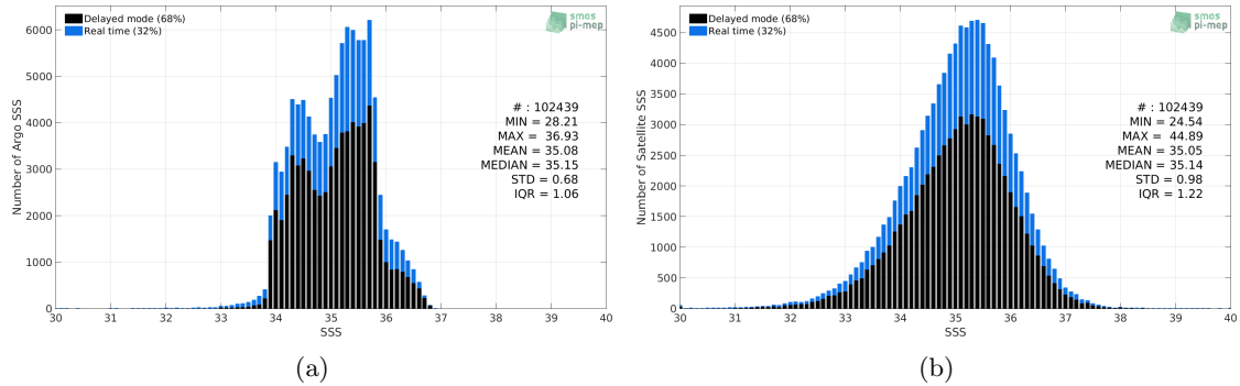
Figure 2: Histograms of SSS from Argo (a) and SMAP-L2-JPL-V4.3 (b) considering all match-up pairs per bins of 0.1 over the South Pacific Ocean Pi-MEP region and for the full satellite product period.
