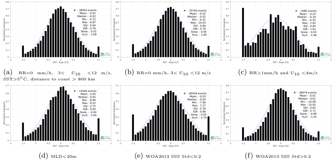
Figure 13: Normalized histogram of \Delta SSS (SMAP-L2-JPL-V4.3 - Argo) for 6 different sub-datasets corresponding to: RR=0 mm/h, 3 < U_{10} < 12 m/s, SST>5°C, distance to coast > 800 km (a), RR=0 mm/h, 3 < U_{10} < 12 m/s (b), RR>1mm/h and U_{10} < 4 m/s (c), MLD<20m (d), WOA2013 SSS Std<0.2 (e), WOA2013 SSS Std>0.2 (f).
