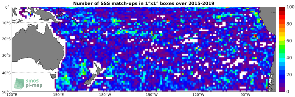
Figure 4: Number of SSS match-ups between Argo SSS and the SMAP-L2-JPL-V4.3 SSS product for the South Pacific Ocean Pi-MEP region over 1^\circ \times 1^\circ boxes and for the full satellite product period.
