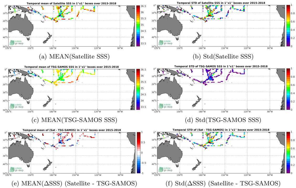
Figure 6: Temporal mean (left) and Std (right) of SSS from SMAP-L2-JPL-V4.2 (top), TSG-SAMOS (middle), and of \Delta SSS (Satellite - TSG-SAMOS). Only match-up pairs are used to generate these maps.
