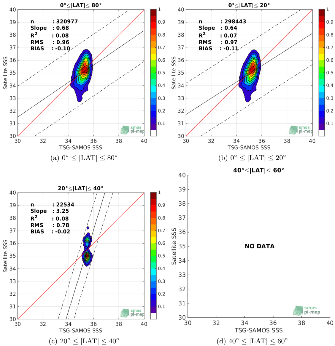
Figure 9: Contour maps of the concentration of SMAP-L2-JPL-V4.2 SSS (y-axis) versus TSG-SAMOS SSS (x-axis) at match-up pairs for different latitude bands. For each plot, the red line shows x=y . The black thin and dashed lines indicate a linear fit through the data cloud and the \pm 95\% confidence levels, respectively. The number match-up pairs n , the slope and R^2 coefficient of the linear fit, the root mean square (RMS) and the mean bias between satellite and in situ data are indicated for each latitude band in each plots.
