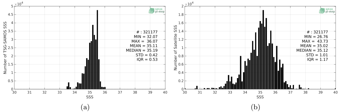
Figure 2: Histograms of SSS from TSG-SAMOS (a) and SMAP-L2-JPL-V4.2 (b) considering all match-up pairs per bins of 0.1 over the South Pacific Ocean Pi-MEP region and for the full satellite product period.
