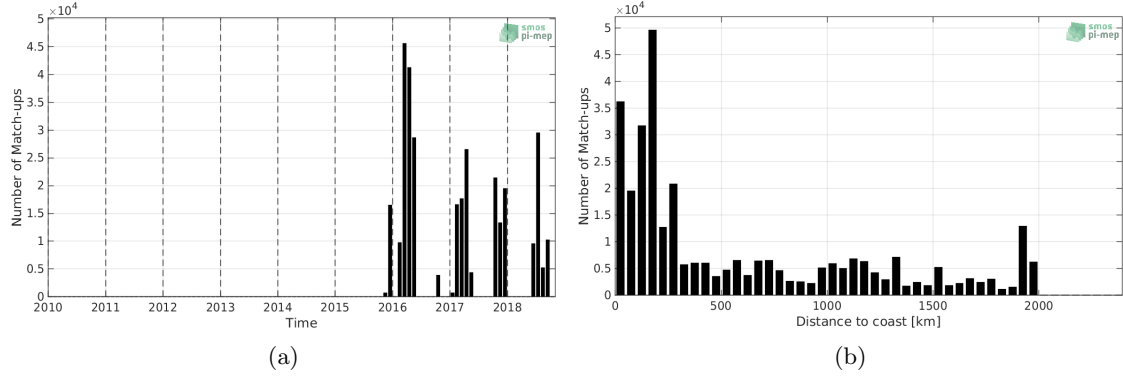
Figure 1: Number of match-ups between TSG-SAMOS and SMAP-L2-JPL-V4.2 SSS as a function of time (a) and as function of the distance to coast (b) over the South Pacific Ocean Pi-MEP region and for the full satellite product period.
