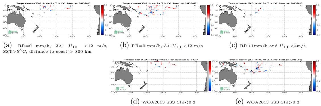
Figure 12: Temporal mean gridded over spatial boxes of size 1^\circ \times 1^\circ of \Delta SSS (SMAP-L2-JPL-V4.2 - TSG-SAMOS) for 5 different subdatasets corresponding to:RR=0 mm/h, 3 < U_{10} < 12 m/s, SST >5^\circ C, distance to coast > 800 km (a), RR=0 mm/h, 3 < U_{10} < 12 m/s (b), RR >1 mm/h and U_{10} < 4 m/s (c), WOA2013 SSS Std <0.2 (d), WOA2013 SSS Std >0.2 (e).
