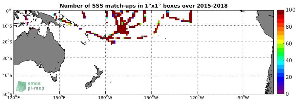
Figure 4: Number of SSS match-ups between TSG-SAMOS SSS and the SMAP-L2-JPL-V4.2 SSS product for the South Pacific Ocean Pi-MEP region over 1^\circ \times 1^\circ boxes and for the full satellite product period.
