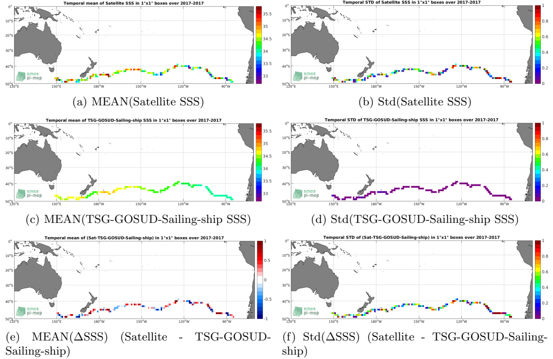
Figure 6: Temporal mean (left) and Std (right) of SSS from SMAP-L2-JPL-V4.2 (top), TSG-GOSUD-Sailing-ship (middle), and of \Delta SSS (Satellite - TSG-GOSUD-Sailing-ship). Only match-up pairs are used to generate these maps.
