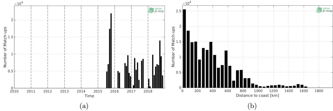
Figure 1: Number of match-ups between TSG-GOSUD-Research-vessel and SMAP-L2-JPL-V4.2 SSS as a function of time (a) and as function of the distance to coast (b) over the South Pacific Ocean Pi-MEP region and for the full satellite product period.
