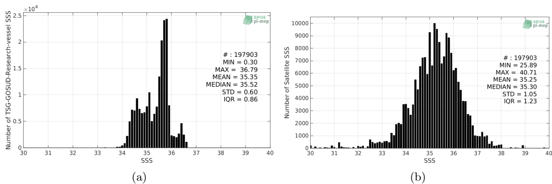
Figure 2: Histograms of SSS from TSG-GOSUD-Research-vessel (a) and SMAP-L2-JPL-V4.2 (b) considering all match-up pairs per bins of 0.1 over the South Pacific Ocean Pi-MEP region and for the full satellite product period.
