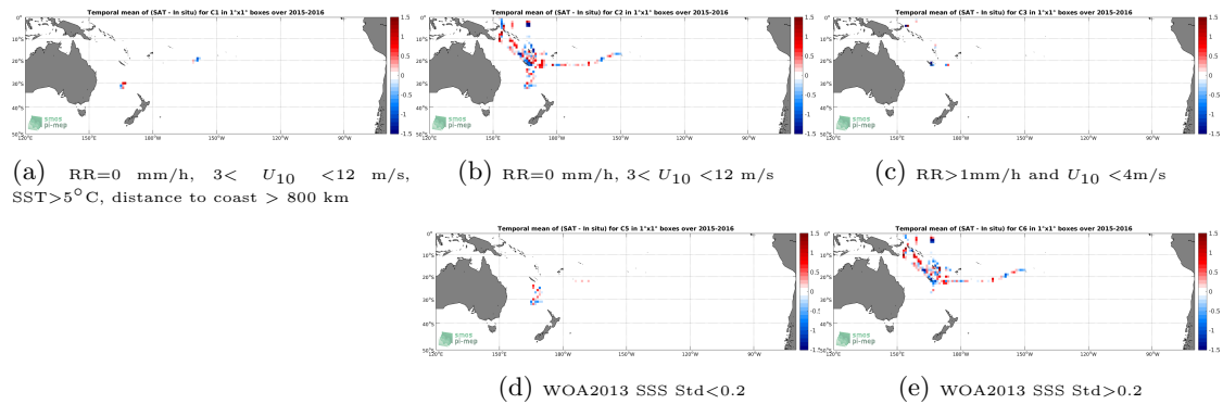
Figure 12: Temporal mean gridded over spatial boxes of size 1^\circ \times 1^\circ of \Delta SSS (SMAP-L2-JPL-V4.2 - TSG-GOSUD-Research-vessel) for 5 different subdatasets corresponding to:RR=0 mm/h, 3 < U_{10} < 12 m/s, SST >5^\circ\text{C} , distance to coast > 800 km (a), RR=0 mm/h, 3 < U_{10} < 12 m/s (b), RR >1 mm/h and U_{10} < 4 m/s (c), WOA2013 SSS Std <0.2 (d), WOA2013 SSS Std >0.2 (e).
