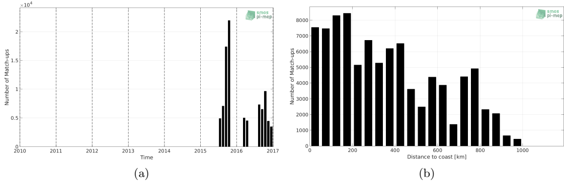
Figure 1: Number of match-ups between TSG-GOSUD-Research-vessel and SMAP-L2-JPL-V4.2 SSS as a function of time (a) and as function of the distance to coast (b) over the South Pacific Ocean Pi-MEP region and for the full satellite product period.
