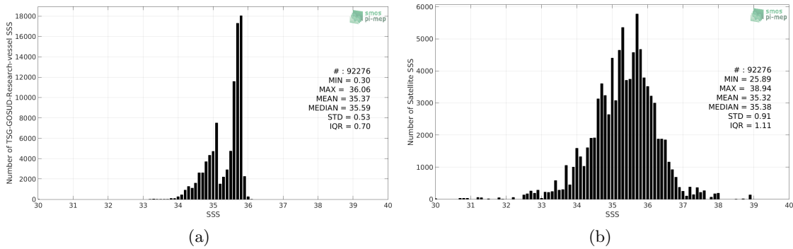
Figure 2: Histograms of SSS from TSG-GOSUD-Research-vessel (a) and SMAP-L2-JPL-V4.2 (b) considering all match-up pairs per bins of 0.1 over the South Pacific Ocean Pi-MEP region and for the full satellite product period.
