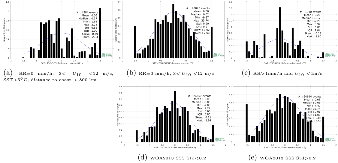
Figure 13: Normalized histogram of \Delta SSS (SMAP-L2-JPL-V4.2 - TSG-GOSUD-Research-vessel) for 5 different subdatasets corresponding to: RR=0 mm/h, 3 < U_{10} < 12 m/s, SST>5°C, distance to coast > 800 km (a), RR=0 mm/h, 3 < U_{10} < 12 m/s (b), RR>1mm/h and U_{10} < 4 m/s (c), WOA2013 SSS Std<0.2 (d), WOA2013 SSS Std>0.2 (e).
