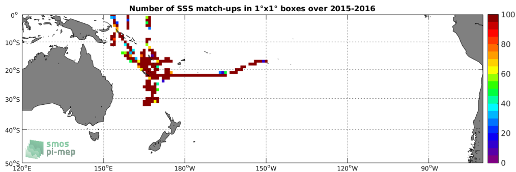
Figure 4: Number of SSS match-ups between TSG-GOSUD-Research-vessel SSS and the SMAP-L2-JPL-V4.2 SSS product for the South Pacific Ocean Pi-MEP region over 1^\circ \times 1^\circ boxes and for the full satellite product period.
