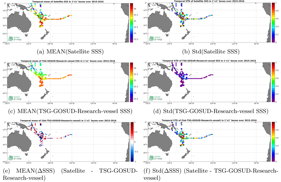
Figure 6: Temporal mean (left) and Std (right) of SSS from SMAP-L2-JPL-V4.2 (top), TSG-GOSUD-Research-vessel (middle), and of \Delta SSS (Satellite - TSG-GOSUD-Research-vessel). Only match-up pairs are used to generate these maps.
