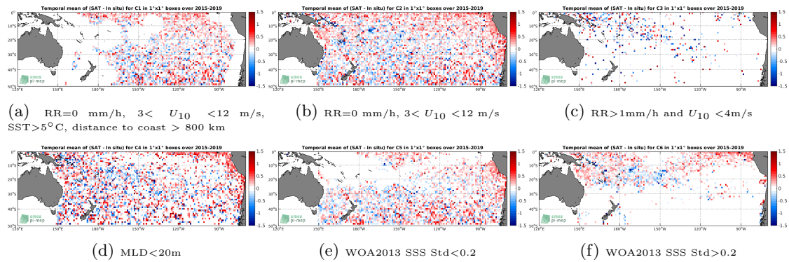
Figure 12: Temporal mean gridded over spatial boxes of size 1^\circ \times 1^\circ of \Delta SSS (SMAP-L2-JPL-V4.2 - Argo) for 6 different subdatasets corresponding to:RR=0 mm/h, 3 < U_{10} < 12 m/s, SST >5^\circ C, distance to coast > 800 km (a), RR=0 mm/h, 3 < U_{10} < 12 m/s (b), RR >1 mm/h and U_{10} < 4 m/s (c),MLD <20 m (d),WOA2013 SSS Std <0.2 (e),WOA2013 SSS Std >0.2 (f).
