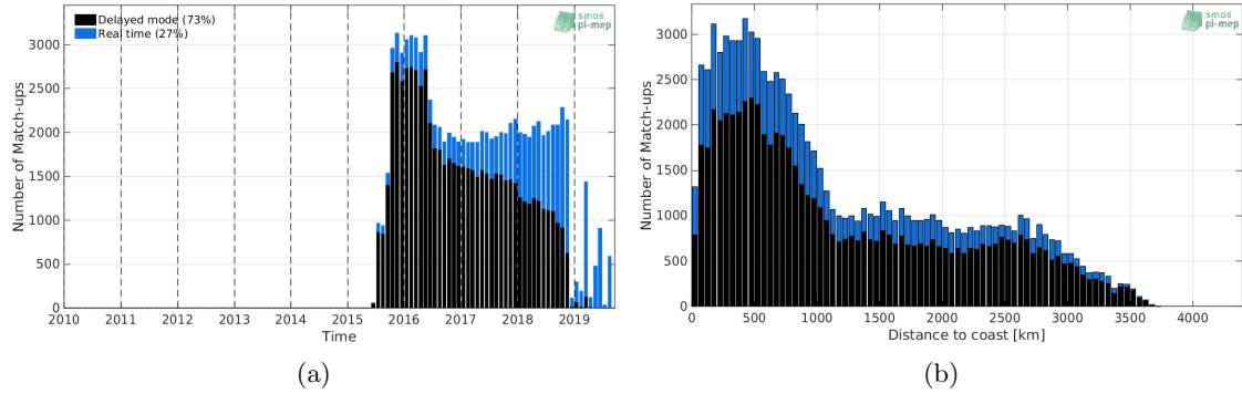
Figure 1: Number of match-ups between Argo and SMAP-L2-JPL-V4.2 SSS as a function of time (a) and as function of the distance to coast (b) over the South Pacific Ocean Pi-MEP region and for the full satellite product period.
