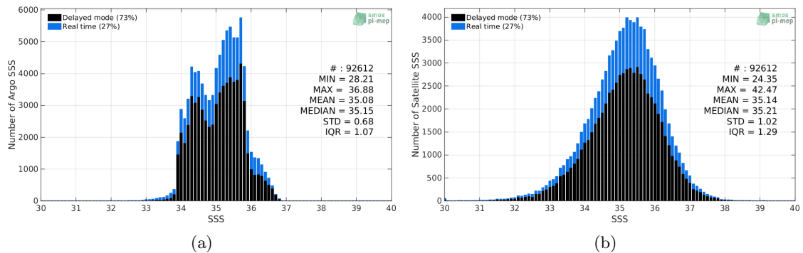
Figure 2: Histograms of SSS from Argo (a) and SMAP-L2-JPL-V4.2 (b) considering all match-up pairs per bins of 0.1 over the South Pacific Ocean Pi-MEP region and for the full satellite product period.
