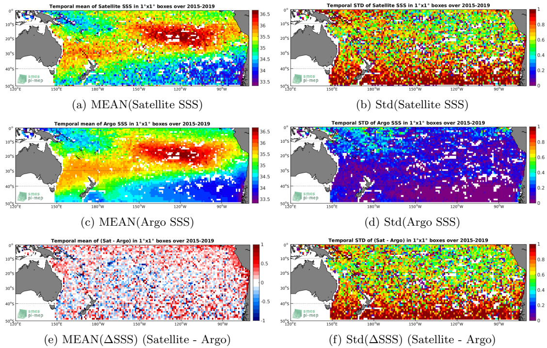
Figure 6: Temporal mean (left) and Std (right) of SSS from SMAP-L2-JPL-V4.2 (top), Argo (middle), and of \Delta SSS (Satellite - Argo). Only match-up pairs are used to generate these maps.
