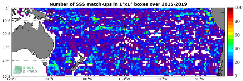
Figure 4: Number of SSS match-ups between Argo SSS and the SMAP-L2-JPL-V4.2 SSS product for the South Pacific Ocean Pi-MEP region over 1^\circ \times 1^\circ boxes and for the full satellite product period.
