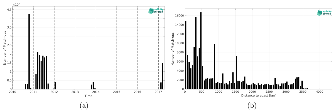
Figure 2: Number of match-ups between TSG (GOSUD-Sailing-ship) and ISAS SSS as a function of time (a) and as function of the distance to coast (b) over the South Pacific Ocean Pi-MEP region and for the full satellite product period.
