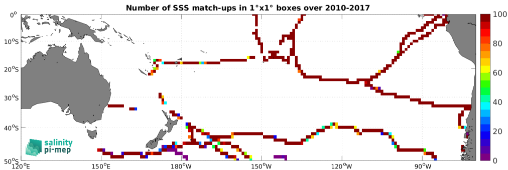
Figure 5: Number of SSS match-ups between TSG (GOSUD-Sailing-ship) SSS and the ISAS SSS product for the South Pacific Ocean Pi-MEP region over 1^\circ \times 1^\circ boxes and for the full satellite product period.
