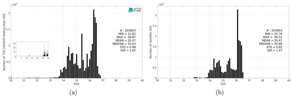
Figure 3: Histograms of SSS from TSG (GOSUD-Sailing-ship) (a) and ISAS (b) considering all match-up pairs per bins of 0.1 over the South Pacific Ocean Pi-MEP region and for the full satellite product period.
