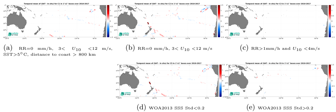
Figure 14: Temporal mean gridded over spatial boxes of size 1^\circ \times 1^\circ of \Delta SSS (ISAS - TSG (GOSUD-Sailing-ship)) for 5 different subdatasets corresponding to:RR=0 mm/h, 3 < U_{10} < 12 m/s, SST>5°C, distance to coast > 800 km (a), RR=0 mm/h, 3 < U_{10} < 12 m/s (b), RR>1mm/h and U_{10} < 4 m/s (c), WOA2013 SSS Std<0.2 (d), WOA2013 SSS Std>0.2 (e).
