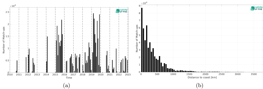
Figure 2: Number of match-ups between TSG (GOSUD-Research-vessel) and ISAS v7 - Monthly (Ifremer-LOPS-CMEMS) SSS as a function of time (a) and as function of the distance to coast (b) over the South Pacific Ocean Pi-MEP region and for the full satellite product period.
