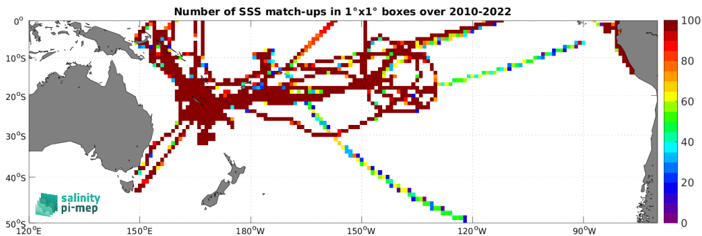
Figure 5: Number of SSS match-ups between TSG (GOSUD-Research-vessel) SSS and the ISAS v7 - Monthly (Ifremer-LOPS-CMEMS) SSS product for the South Pacific Ocean Pi-MEP region over 1^\circ \times 1^\circ boxes and for the full satellite product period.
