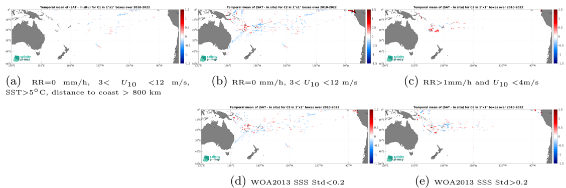
Figure 14: Temporal mean gridded over spatial boxes of size 1^\circ \times 1^\circ of \Delta SSS (ISAS v7 - Monthly (Ifremer-LOPS-CMEMS) - TSG (GOSUD-Research-vessel)) for 5 different subdatasets corresponding to:RR=0 mm/h, 3 < U_{10} < 12 m/s, SST >5^\circ\text{C} , distance to coast > 800 km (a), RR=0 mm/h, 3 < U_{10} < 12 m/s (b), RR >1 mm/h and U_{10} < 4 m/s (c), WOA2013 SSS Std <0.2 (d), WOA2013 SSS Std >0.2 (e).
