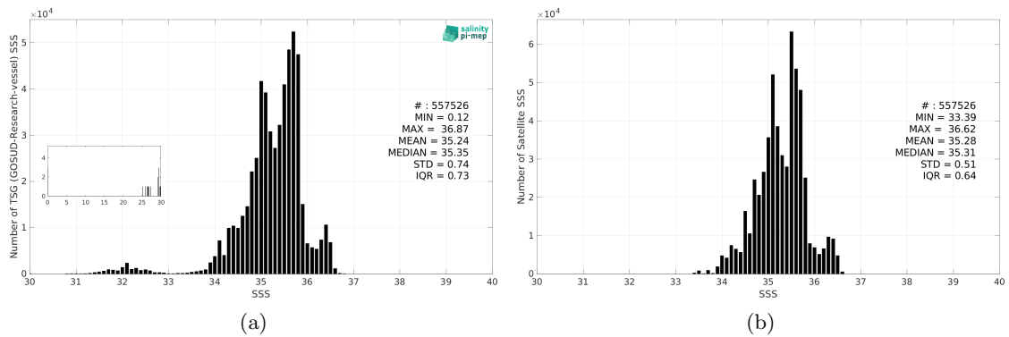
Figure 3: Histograms of SSS from TSG (GOSUD-Research-vessel) (a) and ISAS v7 - Monthly (Ifremer-LOPS-CMEMS) (b) considering all match-up pairs per bins of 0.1 over the South Pacific Ocean Pi-MEP region and for the full satellite product period.
