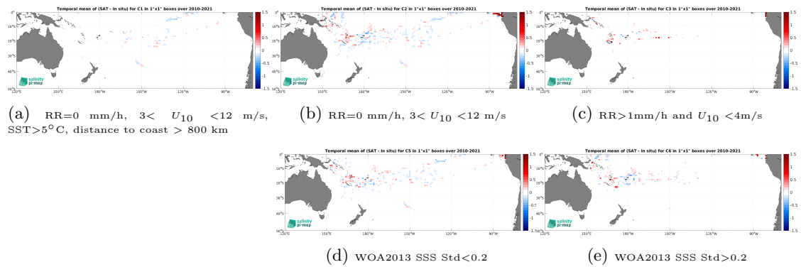
Figure 14: Temporal mean gridded over spatial boxes of size 1^\circ \times 1^\circ of \Delta SSS (ISAS - TSG (GOSUD-Research-vessel)) for 5 different subdatasets corresponding to:RR=0 mm/h, 3 < U_{10} < 12 m/s, SST>5°C, distance to coast > 800 km (a), RR=0 mm/h, 3 < U_{10} < 12 m/s (b), RR>1mm/h and U_{10} < 4 m/s (c), WOA2013 SSS Std<0.2 (d), WOA2013 SSS Std>0.2 (e).
