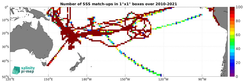
Figure 5: Number of SSS match-ups between TSG (GOSUD-Research-vessel) SSS and the ISAS SSS product for the South Pacific Ocean Pi-MEP region over 1^\circ \times 1^\circ boxes and for the full satellite product period.
