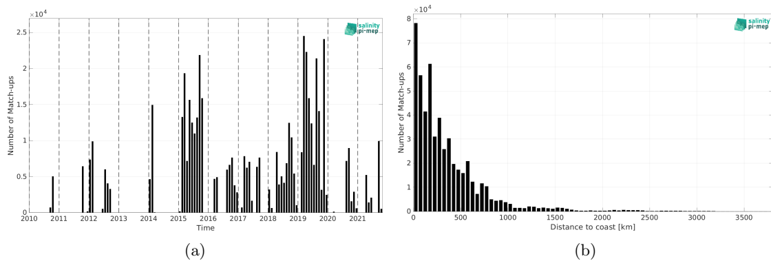
Figure 2: Number of match-ups between TSG (GOSUD-Research-vessel) and ISAS SSS as a function of time (a) and as function of the distance to coast (b) over the South Pacific Ocean Pi-MEP region and for the full satellite product period.
