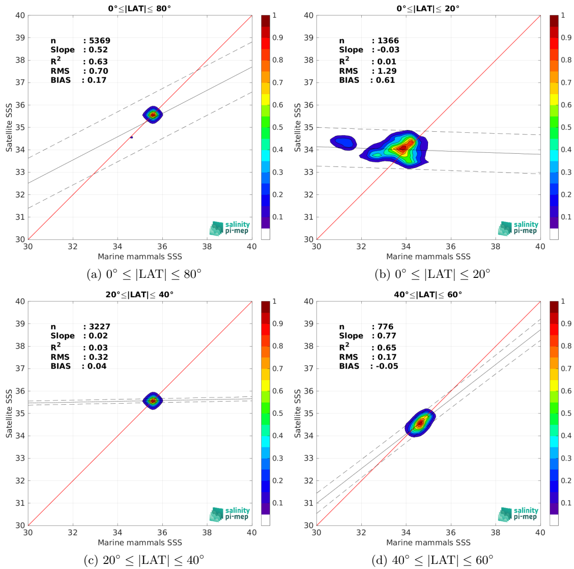
Figure 10: Contour maps of the concentration of ISAS v7 - Monthly (Ifremer-LOPS-CMEMS) SSS (y-axis) versus Marine mammals SSS (x-axis) at match-up pairs for different latitude bands. For each plot, the red line shows x=y . The black thin and dashed lines indicate a linear fit through the data cloud and the \pm 95\% confidence levels, respectively. The number match-up pairs n , the slope and R^2 coefficient of the linear fit, the root mean square (RMS) and the mean bias between satellite and in situ data are indicated for each latitude band in each plots.
