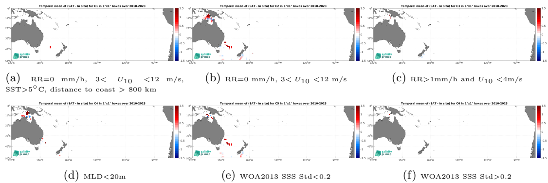
Figure 14: Temporal mean gridded over spatial boxes of size 1^\circ \times 1^\circ of \Delta SSS (ISAS v7 - Monthly (Ifremer-LOPS-CMEMS) - Marine mammals) for 6 different subdatasets corresponding to:RR=0 mm/h, 3 < U_{10} < 12 m/s, SST >5^\circ\text{C} , distance to coast > 800 km (a), RR=0 mm/h, 3 < U_{10} < 12 m/s (b), RR >1 mm/h and U_{10} < 4 m/s (c),MLD <20 m (d),WOA2013 SSS Std <0.2 (e),WOA2013 SSS Std >0.2 (f).
