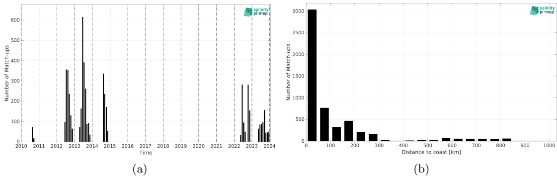
Figure 2: Number of match-ups between Marine mammals and ISAS v7 - Monthly (Ifremer-LOPS-CMEMS) SSS as a function of time (a) and as function of the distance to coast (b) over the South Pacific Ocean Pi-MEP region and for the full satellite product period.
