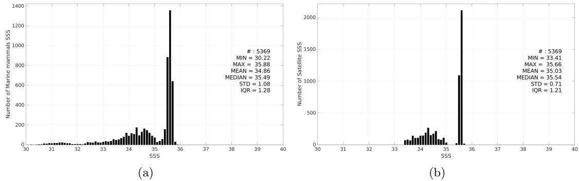
Figure 3: Histograms of SSS from Marine mammals (a) and ISAS v7 - Monthly (Ifremer-LOPS-CMEMS) (b) considering all match-up pairs per bins of 0.1 over the South Pacific Ocean Pi-MEP region and for the full satellite product period.
