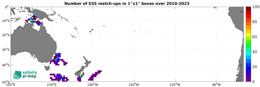
Figure 5: Number of SSS match-ups between Marine mammals SSS and the ISAS v7 - Monthly (Ifremer-LOPS-CMEMS) SSS product for the South Pacific Ocean Pi-MEP region over 1^\circ \times 1^\circ boxes and for the full satellite product period.
