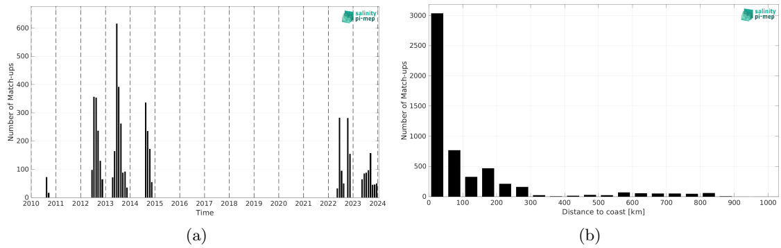
Figure 2: Number of match-ups between Marine mammals and ISAS SSS as a function of time (a) and as function of the distance to coast (b) over the South Pacific Ocean Pi-MEP region and for the full satellite product period.
