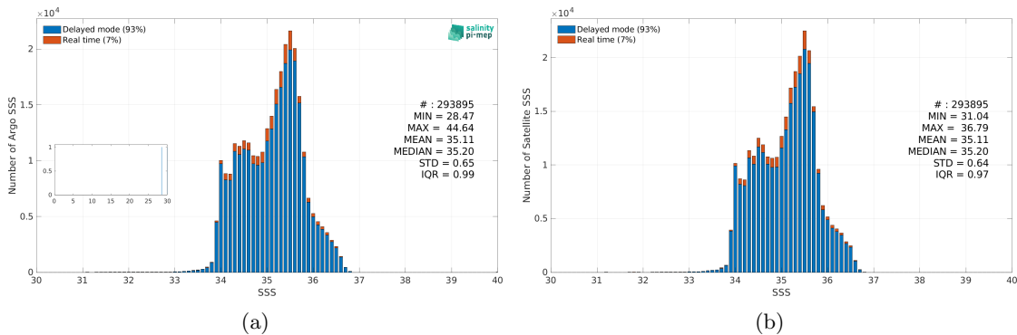
Figure 3: Histograms of SSS from Argo (a) and ISAS (b) considering all match-up pairs per bins of 0.1 over the South Pacific Ocean Pi-MEP region and for the full satellite product period.
