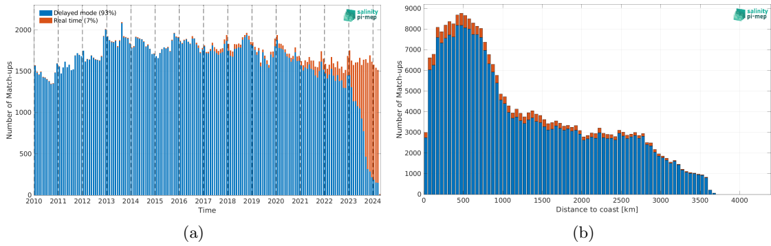
Figure 2: Number of match-ups between Argo and ISAS SSS as a function of time (a) and as function of the distance to coast (b) over the South Pacific Ocean Pi-MEP region and for the full satellite product period.
