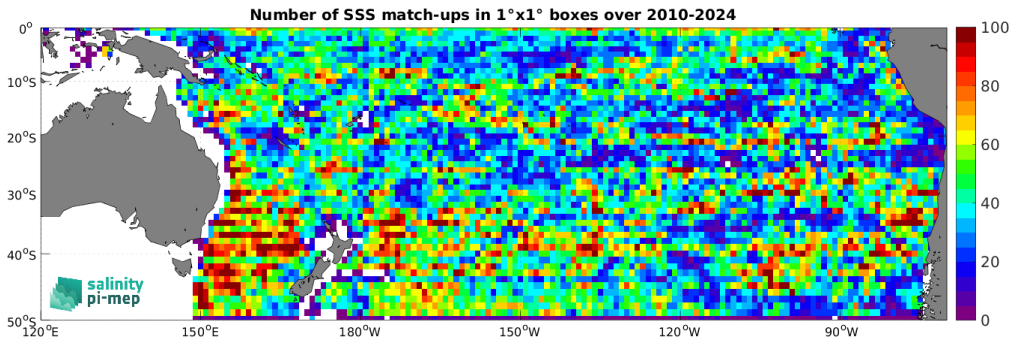
Figure 5: Number of SSS match-ups between Argo SSS and the ISAS SSS product for the South Pacific Ocean Pi-MEP region over 1^\circ \times 1^\circ boxes and for the full satellite product period.
