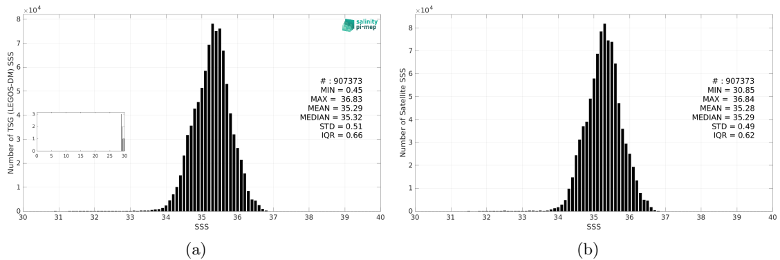
Figure 3: Histograms of SSS from TSG (LEGOS-DM) (a) and CCI SSS L4 Merged-OI v5.5 - 7-day running (ESA) (b) considering all match-up pairs per bins of 0.1 over the South Pacific Ocean Pi-MEP region and for the full satellite product period.
