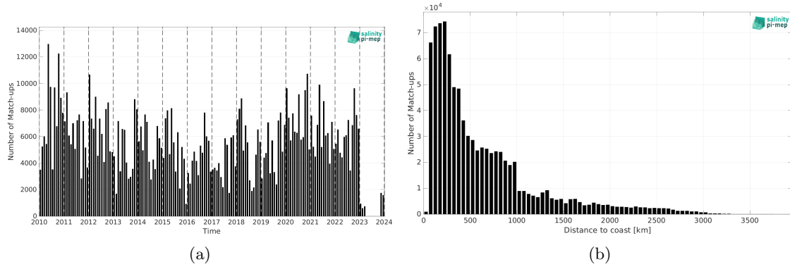
Figure 2: Number of match-ups between TSG (LEGOS-DM) and CCI SSS L4 Merged-OI v5.5 - 7-day running (ESA) SSS as a function of time (a) and as function of the distance to coast (b) over the South Pacific Ocean Pi-MEP region and for the full satellite product period.
