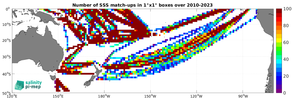
Figure 5: Number of SSS match-ups between TSG (LEGOS-DM) SSS and the CCI SSS L4 Merged-OI v5.5 - 7-day running (ESA) SSS product for the South Pacific Ocean Pi-MEP region over 1^\circ \times 1^\circ boxes and for the full satellite product period.
