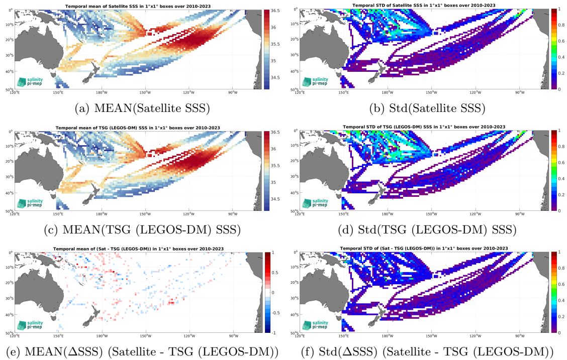
Figure 7: Temporal mean (left) and Std (right) of SSS from CCI SSS L4 Merged-OI v5.5 - 7-day running (ESA) (top), TSG (LEGOS-DM) (middle), and of \Delta SSS (Satellite - TSG (LEGOS-DM)). Only match-up pairs are used to generate these maps.
