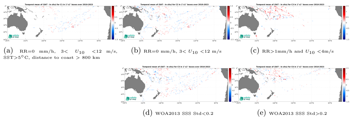
Figure 14: Temporal mean gridded over spatial boxes of size 1^\circ \times 1^\circ of \Delta\text{SSS} (CCI SSS L4 Merged-OI v5.5 - 7-day running (ESA) - TSG (LEGOS-DM)) for 5 different subdatasets corresponding to:RR=0 mm/h, 3 < U_{10} < 12 m/s, SST >5^\circ\text{C} , distance to coast > 800 km (a), RR=0 mm/h, 3 < U_{10} < 12 m/s (b), RR >1 mm/h and U_{10} < 4 m/s (c), WOA2013 SSS Std <0.2 (d), WOA2013 SSS Std >0.2 (e).
