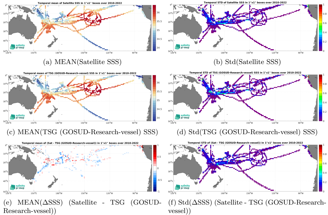
Figure 7: Temporal mean (left) and Std (right) of SSS from CCI SSS L4 Merged-OI v5.5 - 7-day running (ESA) (top), TSG (GOSUD-Research-vessel) (middle), and of \Delta SSS (Satellite - TSG (GOSUD-Research-vessel)). Only match-up pairs are used to generate these maps.
