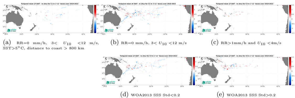
Figure 14: Temporal mean gridded over spatial boxes of size 1^\circ \times 1^\circ of \Delta SSS (CCI SSS L4 Merged-OI v5.5 - 7-day running (ESA) - TSG (GOSUD-Research-vessel)) for 5 different subdatasets corresponding to:RR=0 mm/h, 3 < U_{10} < 12 m/s, SST >5^\circ\text{C} , distance to coast > 800 km (a), RR=0 mm/h, 3 < U_{10} < 12 m/s (b), RR >1 mm/h and U_{10} < 4 m/s (c), WOA2013 SSS Std <0.2 (d), WOA2013 SSS Std >0.2 (e).
