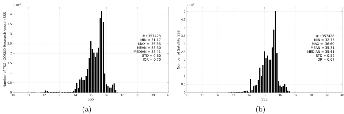
Figure 3: Histograms of SSS from TSG (GOSUD-Research-vessel) (a) and CCI SSS L4 Merged-OI v5.5 - 7-day running (ESA) (b) considering all match-up pairs per bins of 0.1 over the South Pacific Ocean Pi-MEP region and for the full satellite product period.
