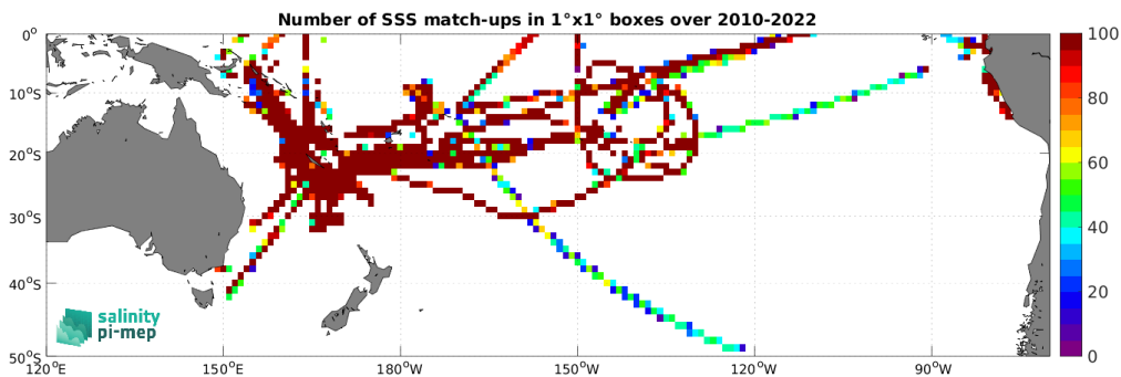
Figure 5: Number of SSS match-ups between TSG (GOSUD-Research-vessel) SSS and the CCI SSS L4 Merged-OI v5.5 - 7-day running (ESA) SSS product for the South Pacific Ocean Pi-MEP region over 1^\circ \times 1^\circ boxes and for the full satellite product period.
