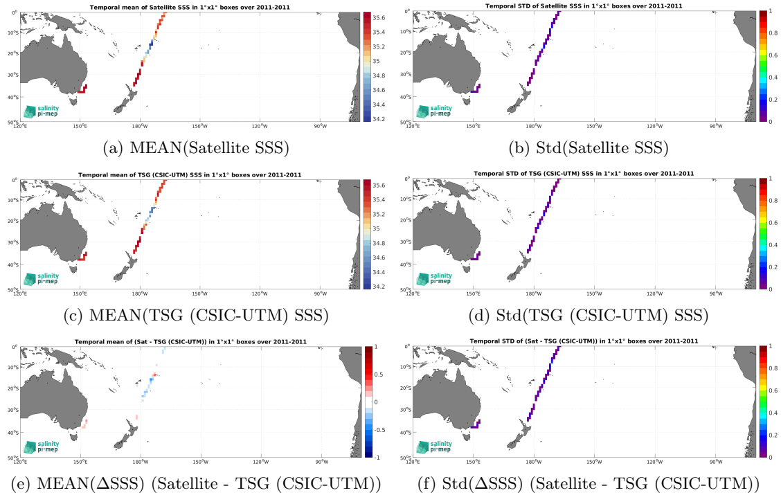
Figure 7: Temporal mean (left) and Std (right) of SSS from CCI SSS L4 Merged-OI v5.5 - 7-day running (ESA) (top), TSG (CSIC-UTM) (middle), and of \Delta SSS (Satellite - TSG (CSIC-UTM)). Only match-up pairs are used to generate these maps.
