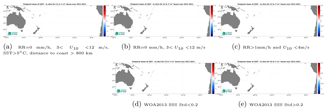
Figure 14: Temporal mean gridded over spatial boxes of size 1^\circ \times 1^\circ of \Delta\text{SSS} (CCI SSS L4 Merged-OI v5.5 - 7-day running (ESA) - TSG (CSIC-UTM)) for 5 different subdatasets corresponding to:RR=0 mm/h, 3 < U_{10} < 12 m/s, SST >5^\circ\text{C} , distance to coast > 800 km (a), RR=0 mm/h, 3 < U_{10} < 12 m/s (b), RR >1 mm/h and U_{10} < 4 m/s (c), WOA2013 SSS Std <0.2 (d), WOA2013 SSS Std >0.2 (e).
