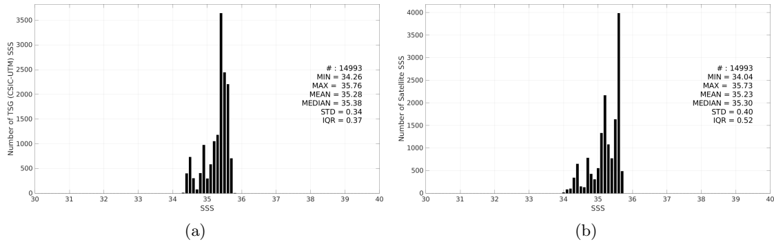
Figure 3: Histograms of SSS from TSG (CSIC-UTM) (a) and CCI SSS L4 Merged-OI v5.5 - 7-day running (ESA) (b) considering all match-up pairs per bins of 0.1 over the South Pacific Ocean Pi-MEP region and for the full satellite product period.
