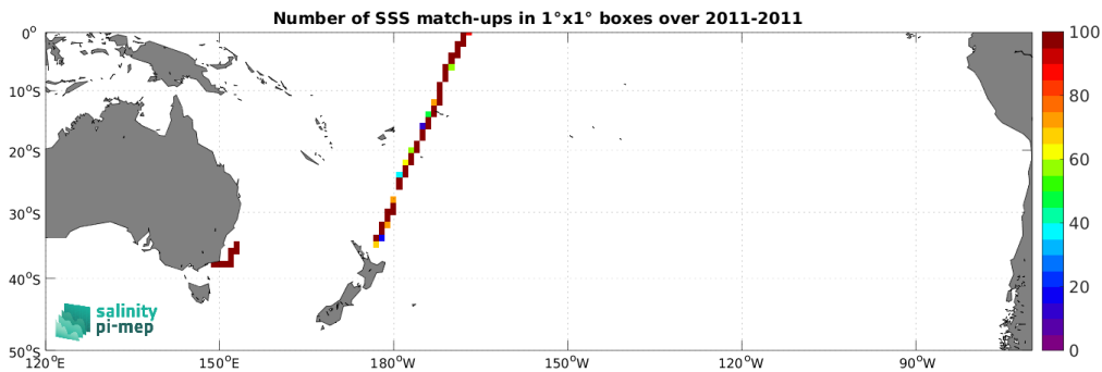
Figure 5: Number of SSS match-ups between TSG (CSIC-UTM) SSS and the CCI SSS L4 Merged-OI v5.5 - 7-day running (ESA) SSS product for the South Pacific Ocean Pi-MEP region over 1^\circ \times 1^\circ boxes and for the full satellite product period.
