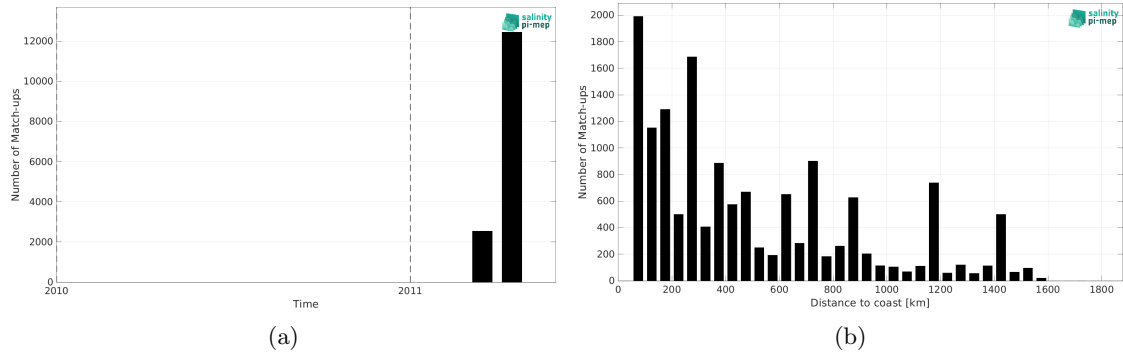
Figure 2: Number of match-ups between TSG (CSIC-UTM) and CCI SSS L4 Merged-OI v5.5 - 7-day running (ESA) SSS as a function of time (a) and as function of the distance to coast (b) over the South Pacific Ocean Pi-MEP region and for the full satellite product period.
