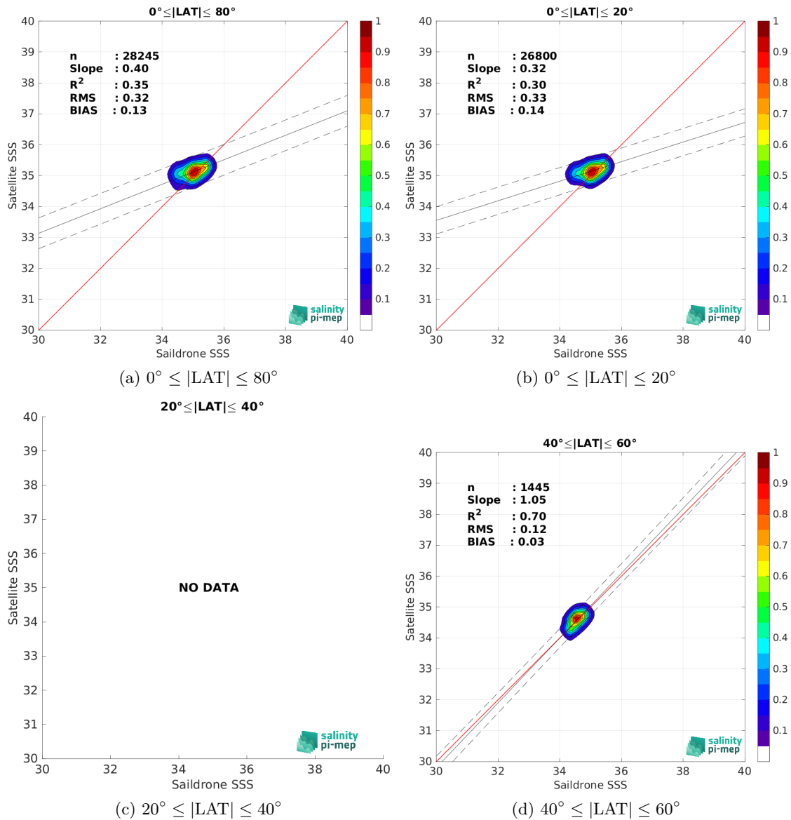
Figure 10: Contour maps of the concentration of CCI SSS L4 Merged-OI v5.5 - 7-day running (ESA) SSS (y-axis) versus Saldrone SSS (x-axis) at match-up pairs for different latitude bands. For each plot, the red line shows x=y . The black thin and dashed lines indicate a linear fit through the data cloud and the \pm 95\% confidence levels, respectively. The number match-up pairs n , the slope and R^2 coefficient of the linear fit, the root mean square (RMS) and the mean bias between satellite and in situ data are indicated for each latitude band in each plots.
