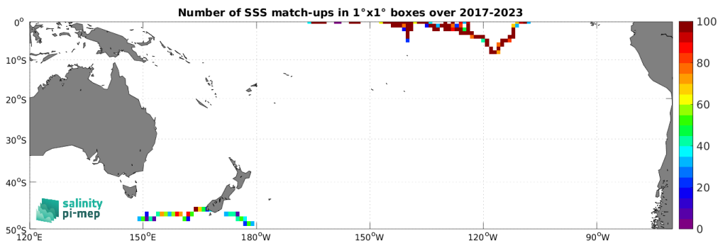
Figure 5: Number of SSS match-ups between Saildrone SSS and the CCI SSS L4 Merged-OI v5.5 - 7-day running (ESA) SSS product for the South Pacific Ocean Pi-MEP region over 1^\circ \times 1^\circ boxes and for the full satellite product period.
