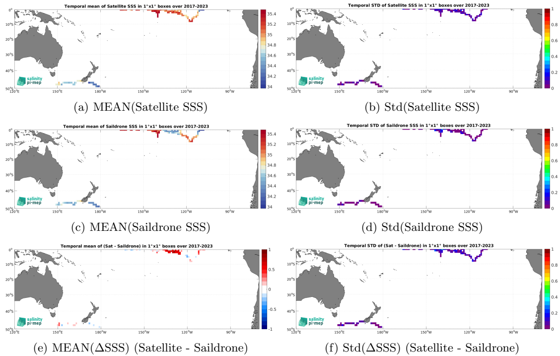
Figure 7: Temporal mean (left) and Std (right) of SSS from CCI SSS L4 Merged-OI v5.5 - 7-day running (ESA) (top), Saildrone (middle), and of \Delta SSS (Satellite - Saildrone). Only match-up pairs are used to generate these maps.
