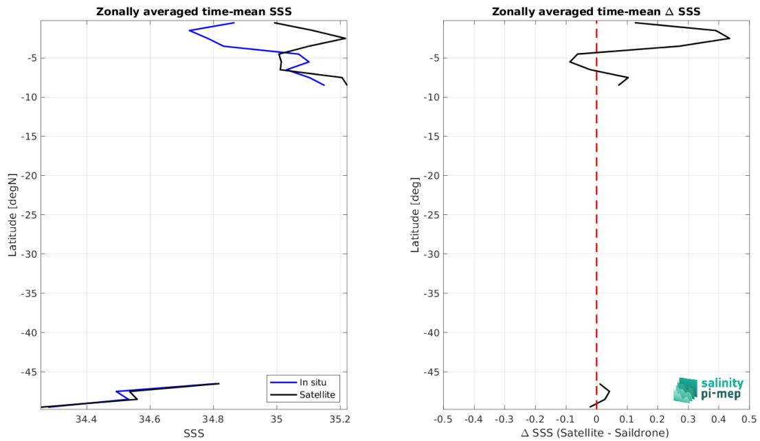
Figure 9: Left panel: Zonal mean SSS from CCI SSS L4 Merged-OI v5.5 - 7-day running (ESA) satellite product (black) and from Sairdronne (blue). Right panel: Zonal mean of \Delta SSS (Satellite - Sairdronne) for all the collected Pi-MEP match-up pairs estimated over the full satellite product period.
