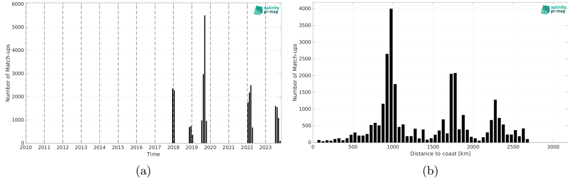
Figure 2: Number of match-ups between Saildrone and CCI SSS L4 Merged-OI v5.5 - 7-day running (ESA) SSS as a function of time (a) and as function of the distance to coast (b) over the South Pacific Ocean Pi-MEP region and for the full satellite product period.
