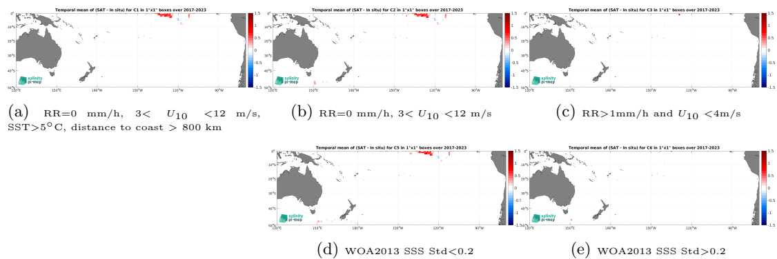
Figure 14: Temporal mean gridded over spatial boxes of size 1^\circ \times 1^\circ of \Delta\text{SSS} (CCI SSS L4 Merged-OI v5.5 - 7-day running (ESA) - Sairdrone) for 5 different subdatasets corresponding to:RR=0 mm/h, 3 < U_{10} < 12 m/s, SST >5^\circ\text{C} , distance to coast > 800 km (a), RR=0 mm/h, 3 < U_{10} < 12 m/s (b), RR >1 mm/h and U_{10} < 4 m/s (c), WOA2013 SSS Std <0.2 (d), WOA2013 SSS Std >0.2 (e).
