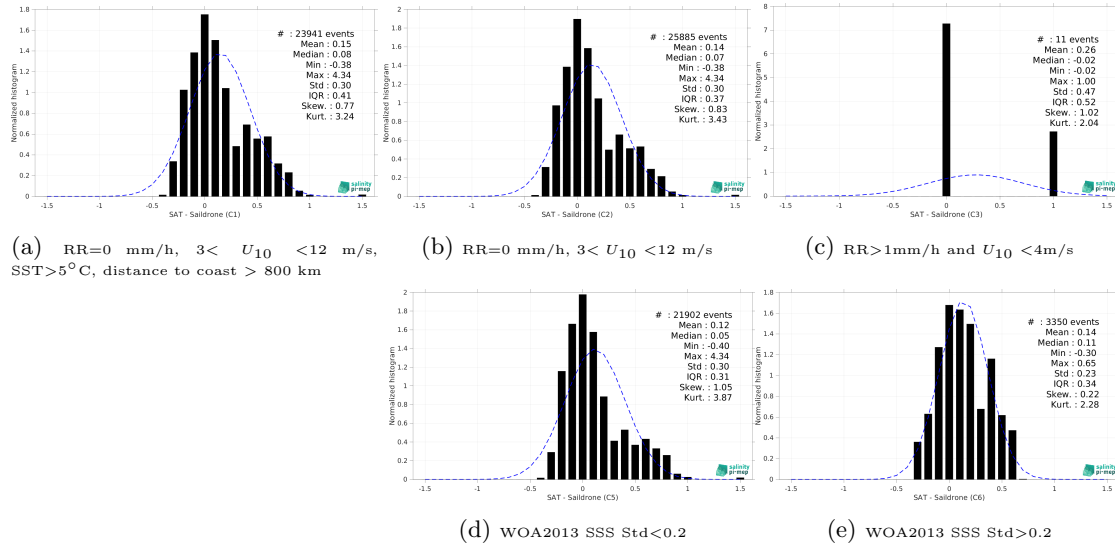
Figure 15: Normalized histogram of \Delta SSS (CCI SSS L4 Merged-OI v5.5 - 7-day running (ESA) - Saldrone) for 5 different subdatasets corresponding to: RR=0 mm/h, 3 < U_{10} < 12 m/s, SST > 5°C, distance to coast > 800 km (a), RR=0 mm/h, 3 < U_{10} < 12 m/s (b), RR > 1mm/h and U_{10} < 4 m/s (c), WOA2013 SSS Std < 0.2 (d), WOA2013 SSS Std > 0.2 (e).
