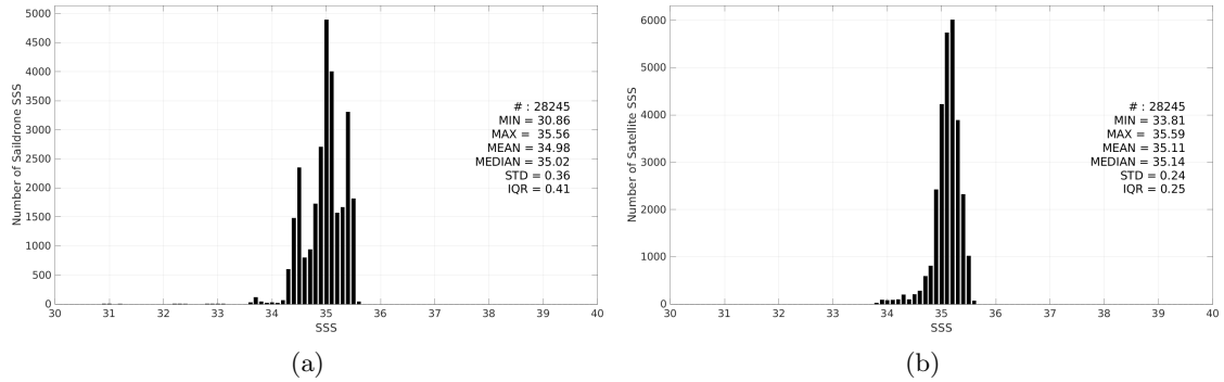
Figure 3: Histograms of SSS from Saildrone (a) and CCI SSS L4 Merged-OI v5.5 - 7-day running (ESA) (b) considering all match-up pairs per bins of 0.1 over the South Pacific Ocean Pi-MEP region and for the full satellite product period.
