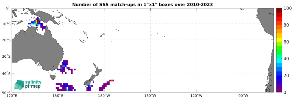
Figure 5: Number of SSS match-ups between Marine mammals SSS and the CCI SSS L4 Merged-OI v5.5 - 7-day running (ESA) SSS product for the South Pacific Ocean Pi-MEP region over 1^\circ \times 1^\circ boxes and for the full satellite product period.
