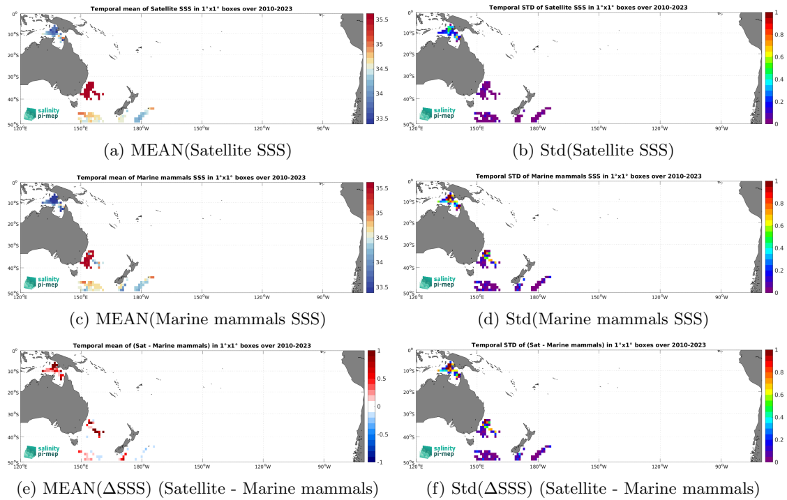
Figure 7: Temporal mean (left) and Std (right) of SSS from CCI SSS L4 Merged-OI v5.5 - 7-day running (ESA) (top), Marine mammals (middle), and of \Delta SSS (Satellite - Marine mammals). Only match-up pairs are used to generate these maps.
