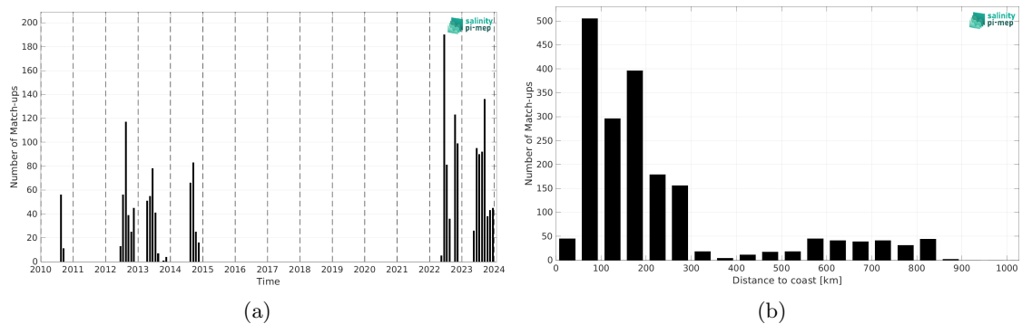
Figure 2: Number of match-ups between Marine mammals and CCI SSS L4 Merged-OI v5.5 - 7-day running (ESA) SSS as a function of time (a) and as function of the distance to coast (b) over the South Pacific Ocean Pi-MEP region and for the full satellite product period.
