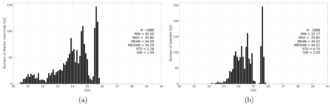
Figure 3: Histograms of SSS from Marine mammals (a) and CCI SSS L4 Merged-OI v5.5 - 7-day running (ESA) (b) considering all match-up pairs per bins of 0.1 over the South Pacific Ocean Pi-MEP region and for the full satellite product period.
