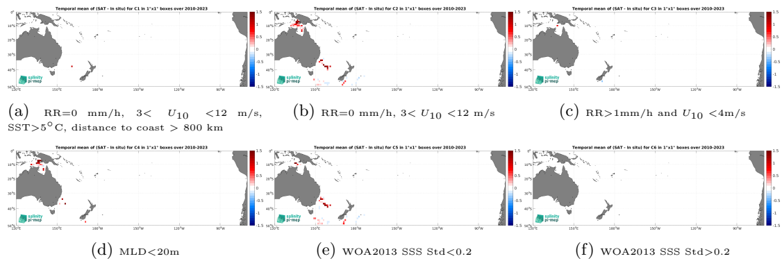
Figure 14: Temporal mean gridded over spatial boxes of size 1^\circ \times 1^\circ of \Delta SSS (CCI SSS L4 Merged-OI v5.5 - 7-day running (ESA) - Marine mammals) for 6 different subdatasets corresponding to:RR=0 mm/h, 3 < U_{10} < 12 m/s, SST >5^\circ C, distance to coast > 800 km (a), RR=0 mm/h, 3 < U_{10} < 12 m/s (b), RR >1 mm/h and U_{10} < 4 m/s (c),MLD <20 m (d),WOA2013 SSS Std <0.2 (e),WOA2013 SSS Std >0.2 (f).
