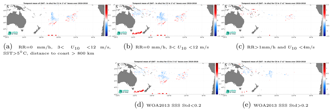
Figure 13: Temporal mean gridded over spatial boxes of size 1^\circ \times 1^\circ of \Delta SSS (CCI SSS L4 Merged-OI v5.5 - 7-day running (ESA) - Surface drifters) for 5 different subdatasets corresponding to:RR=0 mm/h, 3 < U_{10} < 12 m/s, SST >5^\circ C, distance to coast > 800 km (a), RR=0 mm/h, 3 < U_{10} < 12 m/s (b), RR >1 mm/h and U_{10} < 4 m/s (c), WOA2013 SSS Std <0.2 (d), WOA2013 SSS Std >0.2 (e).
