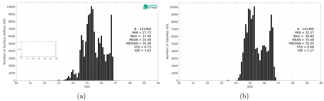
Figure 3: Histograms of SSS from Surface drifters (a) and CCI SSS L4 Merged-OI v5.5 - 7-day running (ESA) (b) considering all match-up pairs per bins of 0.1 over the South Pacific Ocean Pi-MEP region and for the full satellite product period.
