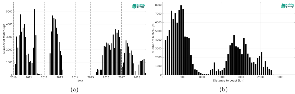
Figure 2: Number of match-ups between Surface drifters and CCI SSS L4 Merged-OI v5.5 - 7-day running (ESA) SSS as a function of time (a) and as function of the distance to coast (b) over the South Pacific Ocean Pi-MEP region and for the full satellite product period.
