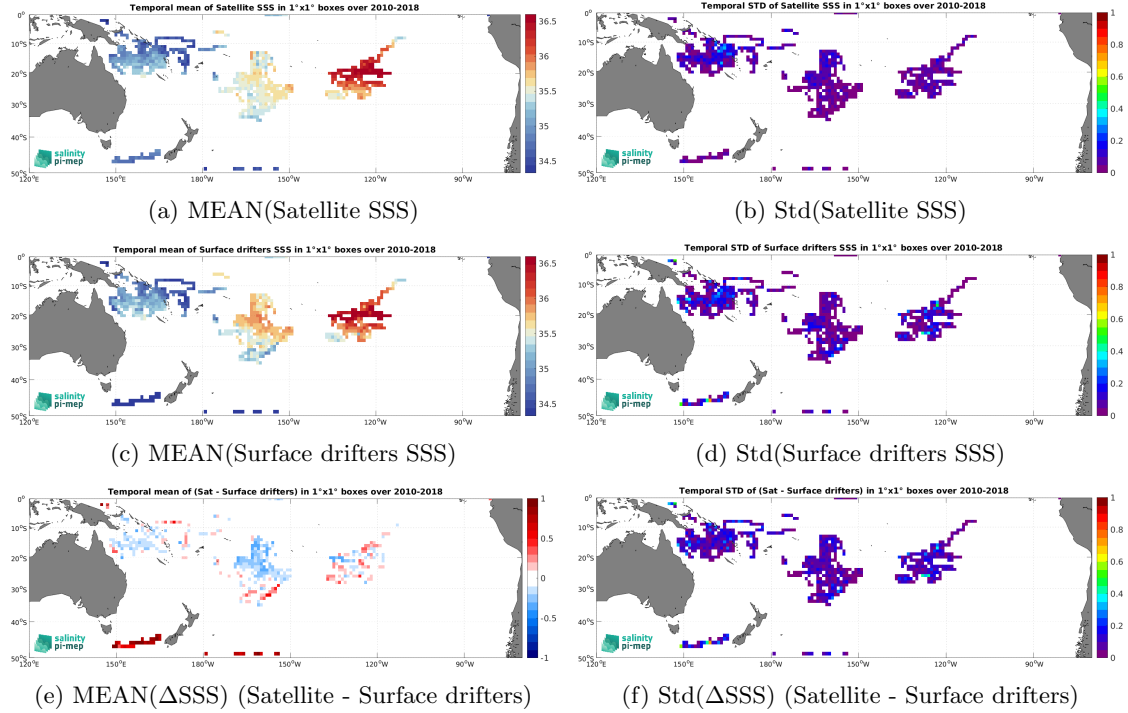
Figure 6: Temporal mean (left) and Std (right) of SSS from CCI SSS L4 Merged-OI v5.5 - 7-day running (ESA) (top), Surface drifters (middle), and of \Delta SSS (Satellite - Surface drifters). Only match-up pairs are used to generate these maps.
