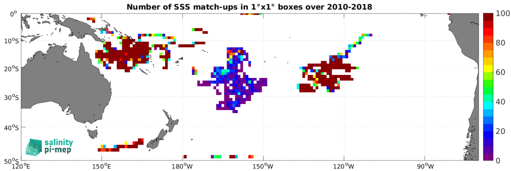
Figure 4: Number of SSS match-ups between Surface drifters SSS and the CCI SSS L4 Merged-OI v5.5 - 7-day running (ESA) SSS product for the South Pacific Ocean Pi-MEP region over 1^\circ \times 1^\circ boxes and for the full satellite product period.
