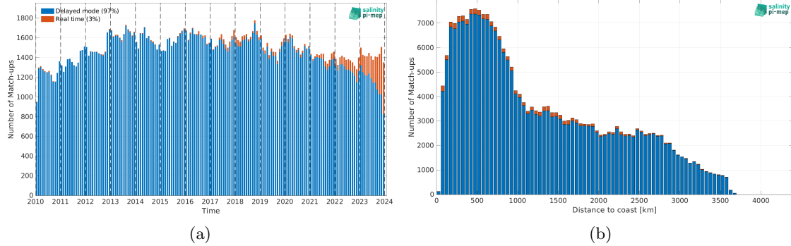
Figure 2: Number of match-ups between Argo and CCI SSS L4 Merged-OI v5.5 - 7-day running (ESA) SSS as a function of time (a) and as function of the distance to coast (b) over the South Pacific Ocean Pi-MEP region and for the full satellite product period.
