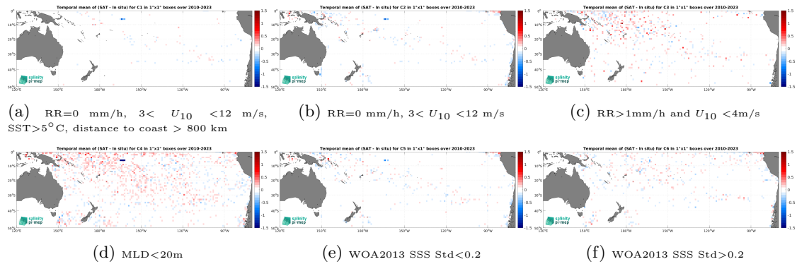
Figure 14: Temporal mean gridded over spatial boxes of size 1^\circ \times 1^\circ of \Delta SSS (CCI SSS L4 Merged-OI v5.5 - 7-day running (ESA) - Argo) for 6 different subdatasets corresponding to:RR=0 mm/h, 3 < U_{10} < 12 m/s, SST >5^\circ C, distance to coast > 800 km (a), RR=0 mm/h, 3 < U_{10} < 12 m/s (b), RR >1 mm/h and U_{10} < 4 m/s (c),MLD <20 m (d),WOA2013 SSS Std <0.2 (e),WOA2013 SSS Std >0.2 (f).
