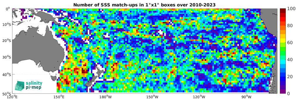
Figure 5: Number of SSS match-ups between Argo SSS and the CCI SSS L4 Merged-OI v5.5 - 7-day running (ESA) SSS product for the South Pacific Ocean Pi-MEP region over 1^\circ \times 1^\circ boxes and for the full satellite product period.
