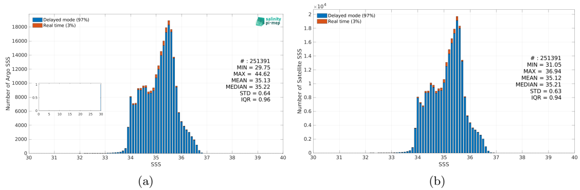
Figure 3: Histograms of SSS from Argo (a) and CCI SSS L4 Merged-OI v5.5 - 7-day running (ESA) (b) considering all match-up pairs per bins of 0.1 over the South Pacific Ocean Pi-MEP region and for the full satellite product period.
