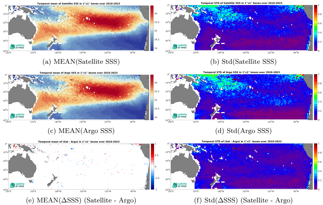
Figure 7: Temporal mean (left) and Std (right) of SSS from CCI SSS L4 Merged-OI v5.5 - 7-day running (ESA) (top), Argo (middle), and of \Delta SSS (Satellite - Argo). Only match-up pairs are used to generate these maps.
