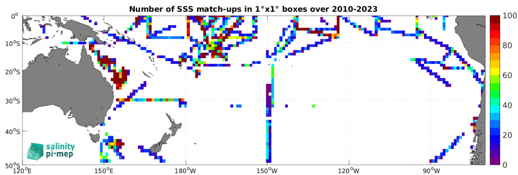
Figure 5: Number of SSS match-ups between TSG (SAMOS) SSS and the CCI SSS L4 Merged-OI v5.5 - 30-day running (ESA) SSS product for the South Pacific Ocean Pi-MEP region over 1^\circ \times 1^\circ boxes and for the full satellite product period.
