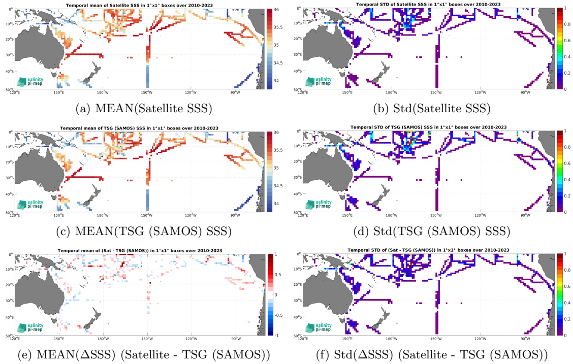
Figure 7: Temporal mean (left) and Std (right) of SSS from CCI SSS L4 Merged-OI v5.5 - 30-day running (ESA) (top), TSG (SAMOS) (middle), and of \Delta SSS (Satellite - TSG (SAMOS)). Only match-up pairs are used to generate these maps.
