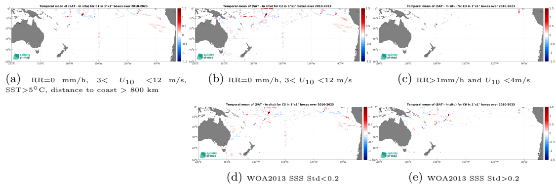
Figure 14: Temporal mean gridded over spatial boxes of size 1^\circ \times 1^\circ of \Delta\text{SSS} (CCI SSS L4 Merged-OI v5.5 - 30-day running (ESA) - TSG (SAMOS)) for 5 different subdatasets corresponding to:RR=0 mm/h, 3 < U_{10} < 12 m/s, SST>5°C, distance to coast > 800 km (a), RR=0 mm/h, 3 < U_{10} < 12 m/s (b), RR>1mm/h and U_{10} < 4 m/s (c), WOA2013 SSS Std<0.2 (d), WOA2013 SSS Std>0.2 (e).
