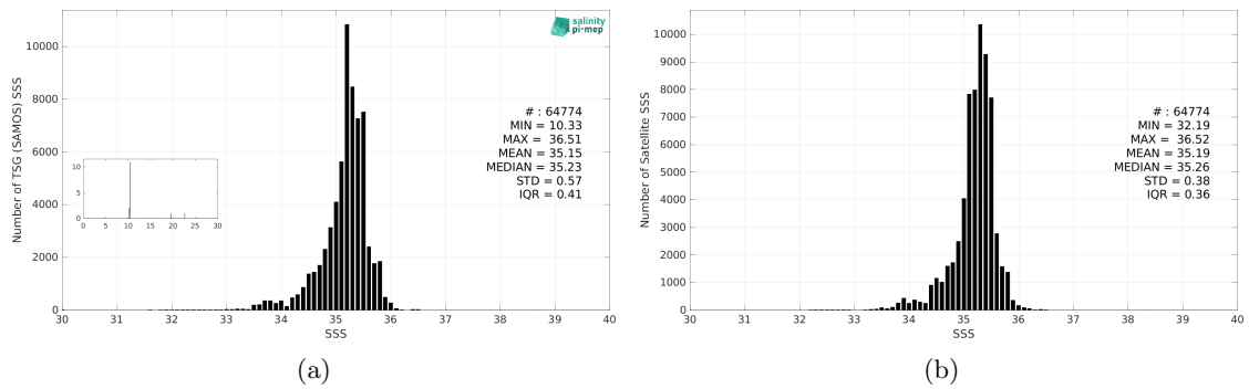
Figure 3: Histograms of SSS from TSG (SAMOS) (a) and CCI SSS L4 Merged-OI v5.5 - 30-day running (ESA) (b) considering all match-up pairs per bins of 0.1 over the South Pacific Ocean Pi-MEP region and for the full satellite product period.
