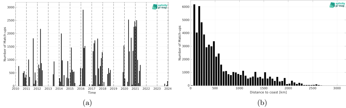
Figure 2: Number of match-ups between TSG (SAMOS) and CCI SSS L4 Merged-OI v5.5 - 30-day running (ESA) SSS as a function of time (a) and as function of the distance to coast (b) over the South Pacific Ocean Pi-MEP region and for the full satellite product period.
