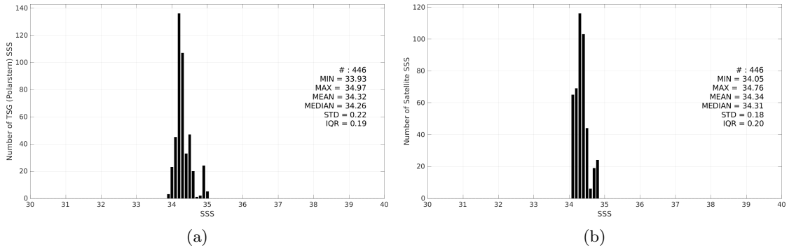
Figure 3: Histograms of SSS from TSG (Polarstern) (a) and CCI SSS L4 Merged-OI v5.5 - 30-day running (ESA) (b) considering all match-up pairs per bins of 0.1 over the South Pacific Ocean Pi-MEP region and for the full satellite product period.
