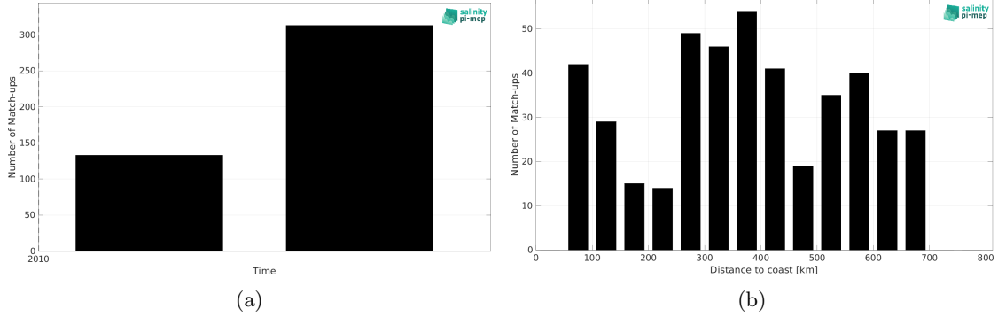
Figure 2: Number of match-ups between TSG (Polarstern) and CCI SSS L4 Merged-OI v5.5 - 30-day running (ESA) SSS as a function of time (a) and as function of the distance to coast (b) over the South Pacific Ocean Pi-MEP region and for the full satellite product period.
