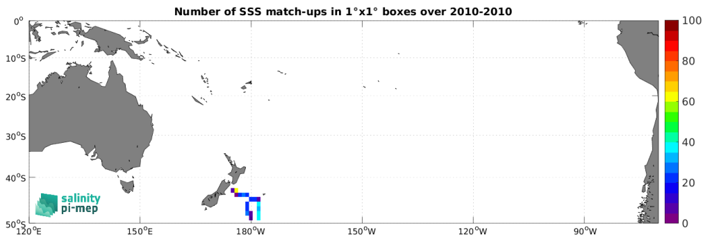
Figure 5: Number of SSS match-ups between TSG (Polarstern) SSS and the CCI SSS L4 Merged-OI v5.5 - 30-day running (ESA) SSS product for the South Pacific Ocean Pi-MEP region over 1^\circ \times 1^\circ boxes and for the full satellite product period.
