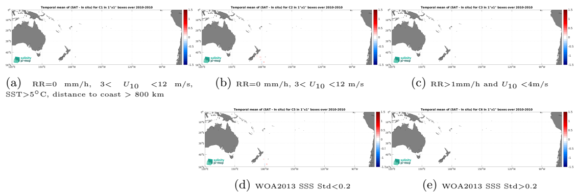
Figure 14: Temporal mean gridded over spatial boxes of size 1^\circ \times 1^\circ of \Delta\text{SSS} (CCI SSS L4 Merged-OI v5.5 - 30-day running (ESA) - TSG (Polarstern)) for 5 different subdatasets corresponding to:RR=0 mm/h, 3 < U_{10} < 12 m/s, SST>5°C, distance to coast > 800 km (a), RR=0 mm/h, 3 < U_{10} < 12 m/s (b), RR>1mm/h and U_{10} < 4 m/s (c), WOA2013 SSS Std<0.2 (d), WOA2013 SSS Std>0.2 (e).
