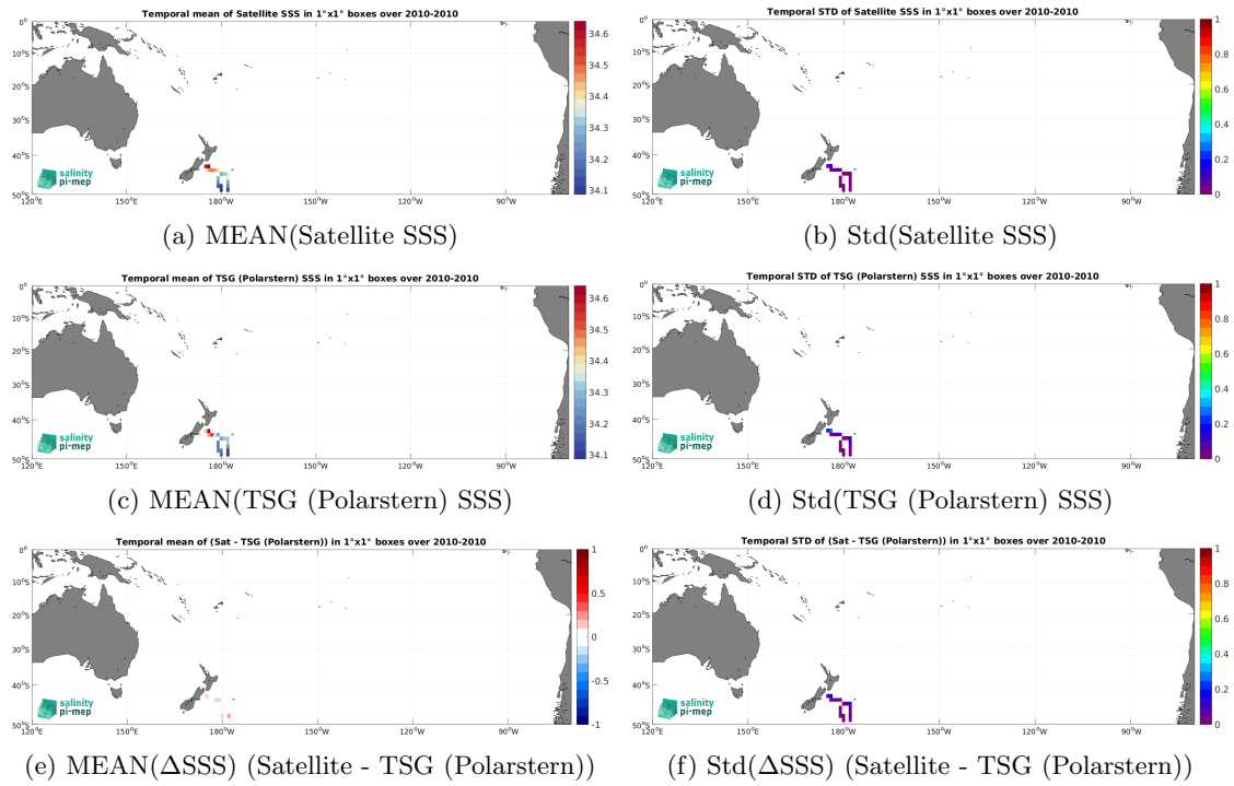
Figure 7: Temporal mean (left) and Std (right) of SSS from CCI SSS L4 Merged-OI v5.5 - 30-day running (ESA) (top), TSG (Polarstern) (middle), and of \Delta SSS (Satellite - TSG (Polarstern)). Only match-up pairs are used to generate these maps.
