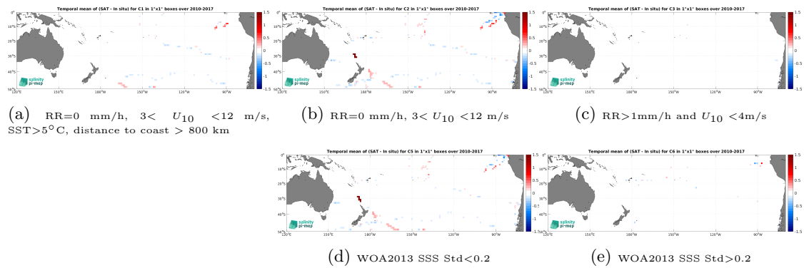
Figure 14: Temporal mean gridded over spatial boxes of size 1^\circ \times 1^\circ of \Delta\text{SSS} (CCI SSS L4 Merged-OI v5.5 - 30-day running (ESA) - TSG (GOSUD-Sailing-ship)) for 5 different subdatasets corresponding to:RR=0 mm/h, 3 < U_{10} < 12 m/s, SST >5^\circ\text{C} , distance to coast > 800 km (a), RR=0 mm/h, 3 < U_{10} < 12 m/s (b), RR >1 mm/h and U_{10} < 4 m/s (c), WOA2013 SSS Std <0.2 (d), WOA2013 SSS Std >0.2 (e).
