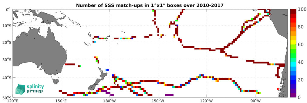
Figure 5: Number of SSS match-ups between TSG (GOSUD-Sailing-ship) SSS and the CCI SSS L4 Merged-OI v5.5 - 30-day running (ESA) SSS product for the South Pacific Ocean Pi-MEP region over 1^\circ \times 1^\circ boxes and for the full satellite product period.
