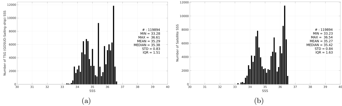
Figure 3: Histograms of SSS from TSG (GOSUD-Sailing-ship) (a) and CCI SSS L4 Merged-OI v5.5 - 30-day running (ESA) (b) considering all match-up pairs per bins of 0.1 over the South Pacific Ocean Pi-MEP region and for the full satellite product period.
