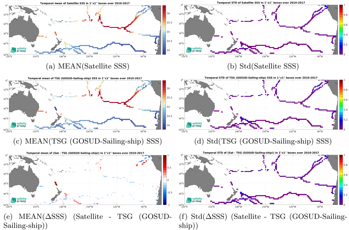
Figure 7: Temporal mean (left) and Std (right) of SSS from CCI SSS L4 Merged-OI v5.5 - 30-day running (ESA) (top), TSG (GOSUD-Sailing-ship) (middle), and of \Delta SSS (Satellite - TSG (GOSUD-Sailing-ship)). Only match-up pairs are used to generate these maps.
