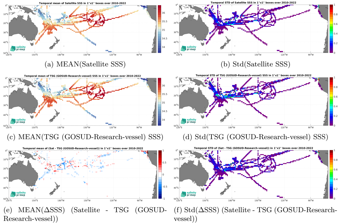
Figure 7: Temporal mean (left) and Std (right) of SSS from CCI SSS L4 Merged-OI v5.5 - 30-day running (ESA) (top), TSG (GOSUD-Research-vessel) (middle), and of \Delta SSS (Satellite - TSG (GOSUD-Research-vessel)). Only match-up pairs are used to generate these maps.
