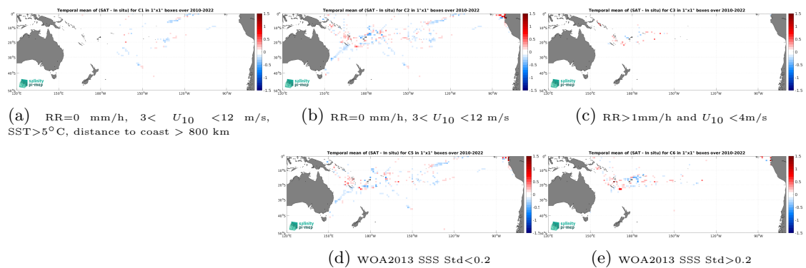
Figure 14: Temporal mean gridded over spatial boxes of size 1^\circ \times 1^\circ of \Delta\text{SSS} (CCI SSS L4 Merged-OI v5.5 - 30-day running (ESA) - TSG (GOSUD-Research-vessel)) for 5 different subdatasets corresponding to:RR=0 mm/h, 3 < U_{10} < 12 m/s, SST >5^\circ\text{C} , distance to coast > 800 km (a), RR=0 mm/h, 3 < U_{10} < 12 m/s (b), RR >1 mm/h and U_{10} < 4 m/s (c), WOA2013 SSS Std <0.2 (d), WOA2013 SSS Std >0.2 (e).
