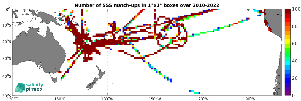
Figure 5: Number of SSS match-ups between TSG (GOSUD-Research-vessel) SSS and the CCI SSS L4 Merged-OI v5.5 - 30-day running (ESA) SSS product for the South Pacific Ocean Pi-MEP region over 1^\circ \times 1^\circ boxes and for the full satellite product period.
