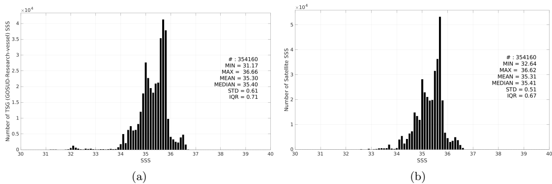
Figure 3: Histograms of SSS from TSG (GOSUD-Research-vessel) (a) and CCI SSS L4 Merged-OI v5.5 - 30-day running (ESA) (b) considering all match-up pairs per bins of 0.1 over the South Pacific Ocean Pi-MEP region and for the full satellite product period.
