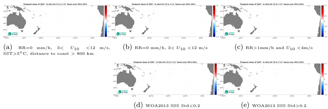
Figure 14: Temporal mean gridded over spatial boxes of size 1^\circ \times 1^\circ of \Delta\text{SSS} (CCI SSS L4 Merged-OI v5.5 - 30-day running (ESA) - TSG (CSIC-UTM)) for 5 different subdatasets corresponding to:RR=0 mm/h, 3 < U_{10} < 12 m/s, SST >5^\circ\text{C} , distance to coast > 800 km (a), RR=0 mm/h, 3 < U_{10} < 12 m/s (b), RR >1 mm/h and U_{10} < 4 m/s (c), WOA2013 SSS Std <0.2 (d), WOA2013 SSS Std >0.2 (e).
