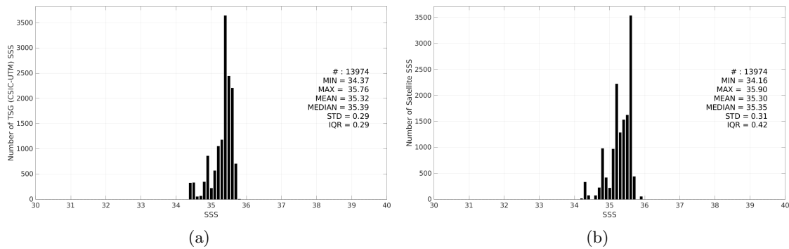
Figure 3: Histograms of SSS from TSG (CSIC-UTM) (a) and CCI SSS L4 Merged-OI v5.5 - 30-day running (ESA) (b) considering all match-up pairs per bins of 0.1 over the South Pacific Ocean Pi-MEP region and for the full satellite product period.
