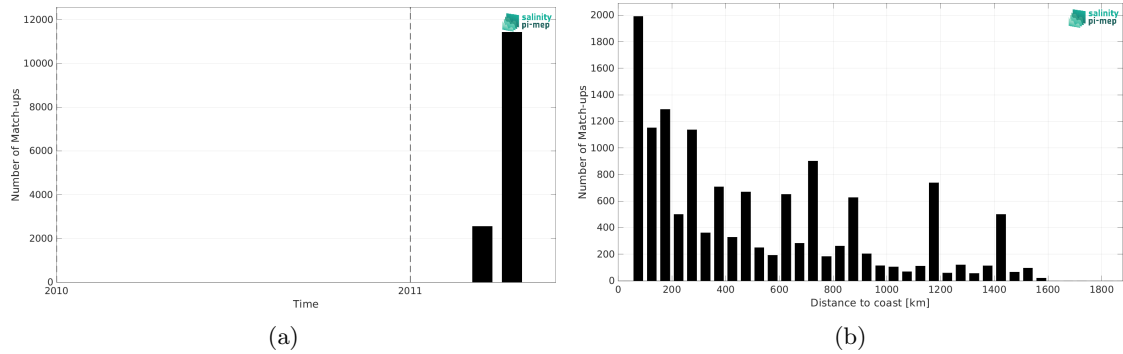
Figure 2: Number of match-ups between TSG (CSIC-UTM) and CCI SSS L4 Merged-OI v5.5 - 30-day running (ESA) SSS as a function of time (a) and as function of the distance to coast (b) over the South Pacific Ocean Pi-MEP region and for the full satellite product period.
