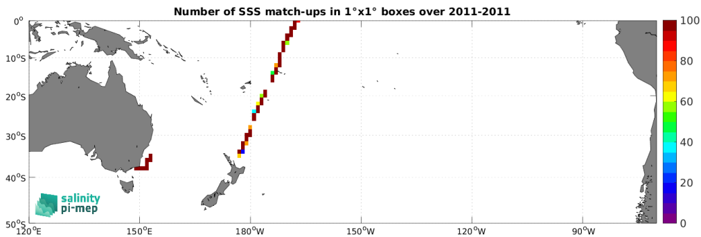
Figure 5: Number of SSS match-ups between TSG (CSIC-UTM) SSS and the CCI SSS L4 Merged-OI v5.5 - 30-day running (ESA) SSS product for the South Pacific Ocean Pi-MEP region over 1^\circ \times 1^\circ boxes and for the full satellite product period.
