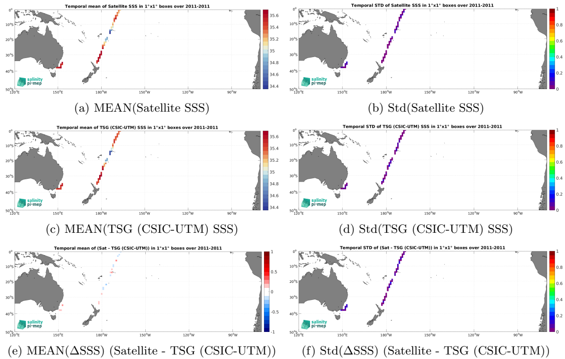
Figure 7: Temporal mean (left) and Std (right) of SSS from CCI SSS L4 Merged-OI v5.5 - 30-day running (ESA) (top), TSG (CSIC-UTM) (middle), and of \Delta SSS (Satellite - TSG (CSIC-UTM)). Only match-up pairs are used to generate these maps.
