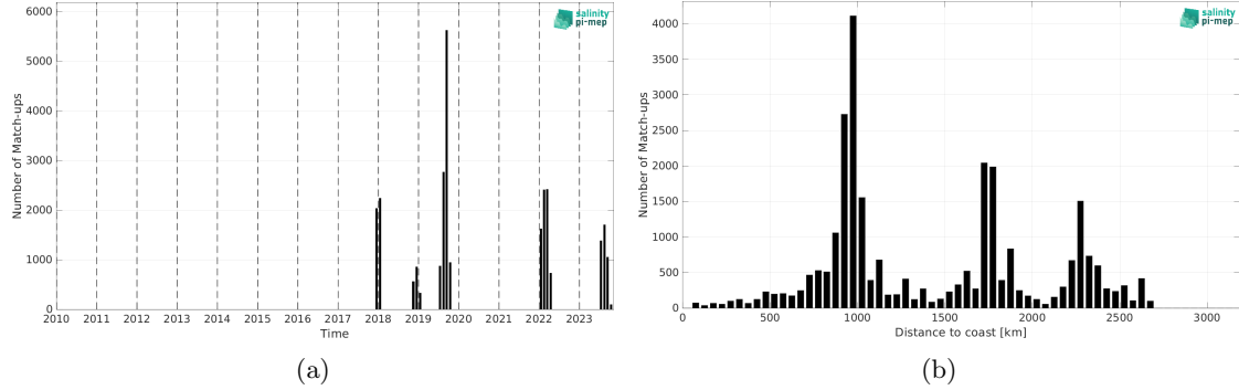
Figure 2: Number of match-ups between Saildrone and CCI SSS L4 Merged-OI v5.5 - 30-day running (ESA) SSS as a function of time (a) and as function of the distance to coast (b) over the South Pacific Ocean Pi-MEP region and for the full satellite product period.
