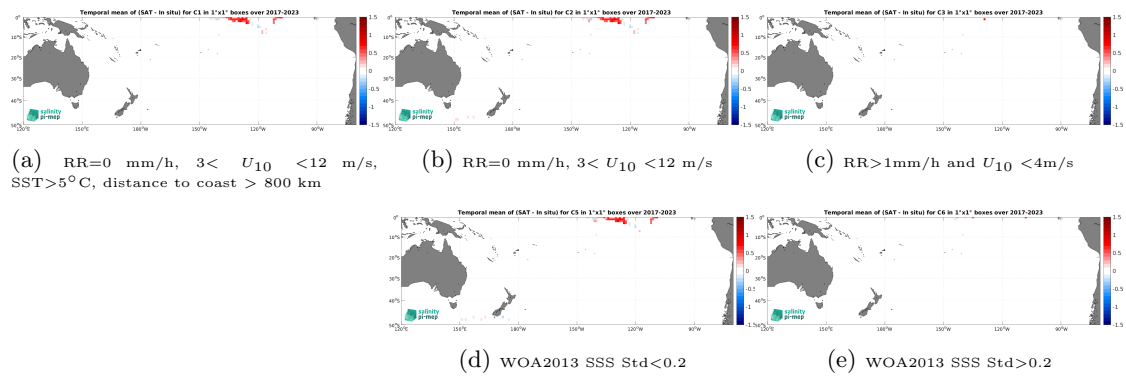
Figure 14: Temporal mean gridded over spatial boxes of size 1^\circ \times 1^\circ of \Delta\text{SSS} (CCI SSS L4 Merged-OI v5.5 - 30-day running (ESA) - Saildrone) for 5 different subdatasets corresponding to:RR=0 mm/h, 3 < U_{10} < 12 m/s, SST >5^\circ\text{C} , distance to coast > 800 km (a), RR=0 mm/h, 3 < U_{10} < 12 m/s (b), RR >1 mm/h and U_{10} < 4 m/s (c), WOA2013 SSS Std <0.2 (d), WOA2013 SSS Std >0.2 (e).
