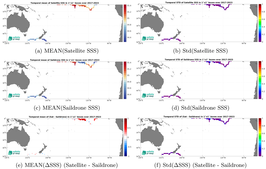
Figure 7: Temporal mean (left) and Std (right) of SSS from CCI SSS L4 Merged-OI v5.5 - 30-day running (ESA) (top), Saildrone (middle), and of \Delta SSS (Satellite - Saildrone). Only match-up pairs are used to generate these maps.
