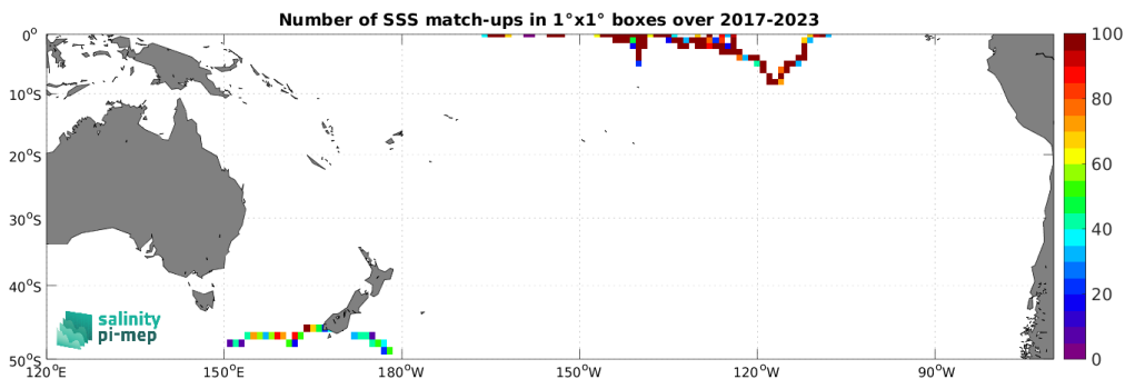
Figure 5: Number of SSS match-ups between Saildrone SSS and the CCI SSS L4 Merged-OI v5.5 - 30-day running (ESA) SSS product for the South Pacific Ocean Pi-MEP region over 1^\circ \times 1^\circ boxes and for the full satellite product period.
