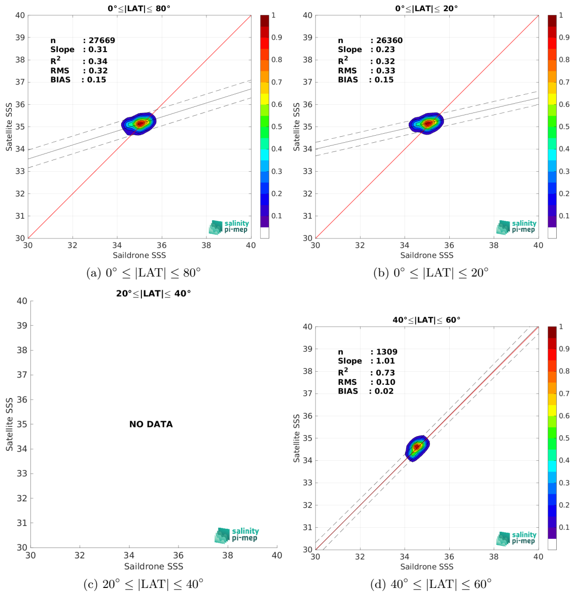
Figure 10: Contour maps of the concentration of CCI SSS L4 Merged-OI v5.5 - 30-day running (ESA) SSS (y-axis) versus Sairdron SSS (x-axis) at match-up pairs for different latitude bands. For each plot, the red line shows x=y . The black thin and dashed lines indicate a linear fit through the data cloud and the \pm 95\% confidence levels, respectively. The number match-up pairs n , the slope and R^2 coefficient of the linear fit, the root mean square (RMS) and the mean bias between satellite and in situ data are indicated for each latitude band in each plots.
