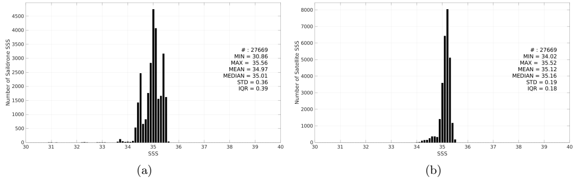
Figure 3: Histograms of SSS from Saildrone (a) and CCI SSS L4 Merged-OI v5.5 - 30-day running (ESA) (b) considering all match-up pairs per bins of 0.1 over the South Pacific Ocean Pi-MEP region and for the full satellite product period.
