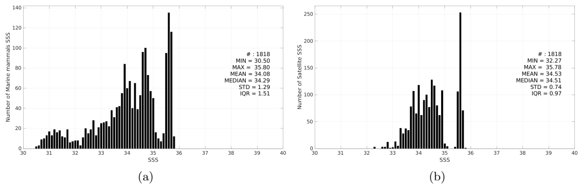
Figure 3: Histograms of SSS from Marine mammals (a) and CCI SSS L4 Merged-OI v5.5 - 30-day running (ESA) (b) considering all match-up pairs per bins of 0.1 over the South Pacific Ocean Pi-MEP region and for the full satellite product period.
