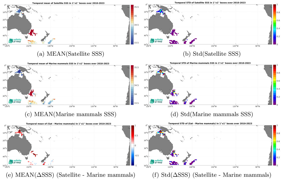
Figure 7: Temporal mean (left) and Std (right) of SSS from CCI SSS L4 Merged-OI v5.5 - 30-day running (ESA) (top), Marine mammals (middle), and of \Delta SSS (Satellite - Marine mammals). Only match-up pairs are used to generate these maps.
