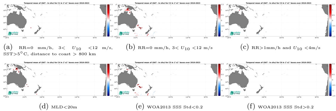
Figure 14: Temporal mean gridded over spatial boxes of size 1^\circ \times 1^\circ of \Delta SSS (CCI SSS L4 Merged-OI v5.5 - 30-day running (ESA) - Marine mammals) for 6 different subdatasets corresponding to:RR=0 mm/h, 3 < U_{10} < 12 m/s, SST >5^\circ C, distance to coast > 800 km (a), RR=0 mm/h, 3 < U_{10} < 12 m/s (b), RR >1 mm/h and U_{10} < 4 m/s (c),MLD <20 m (d),WOA2013 SSS Std <0.2 (e),WOA2013 SSS Std >0.2 (f).
