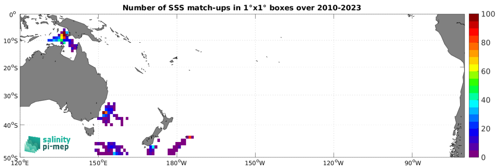
Figure 5: Number of SSS match-ups between Marine mammals SSS and the CCI SSS L4 Merged-OI v5.5 - 30-day running (ESA) SSS product for the South Pacific Ocean Pi-MEP region over 1^\circ \times 1^\circ boxes and for the full satellite product period.
