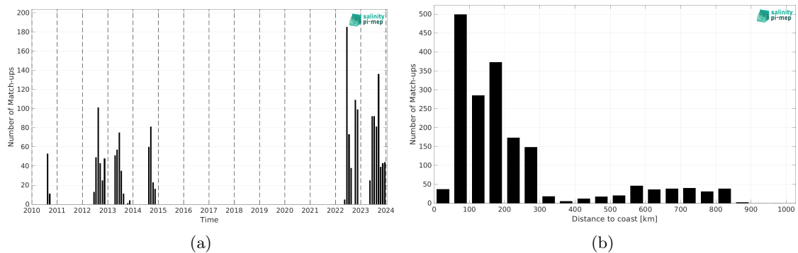
Figure 2: Number of match-ups between Marine mammals and CCI SSS L4 Merged-OI v5.5 - 30-day running (ESA) SSS as a function of time (a) and as function of the distance to coast (b) over the South Pacific Ocean Pi-MEP region and for the full satellite product period.
