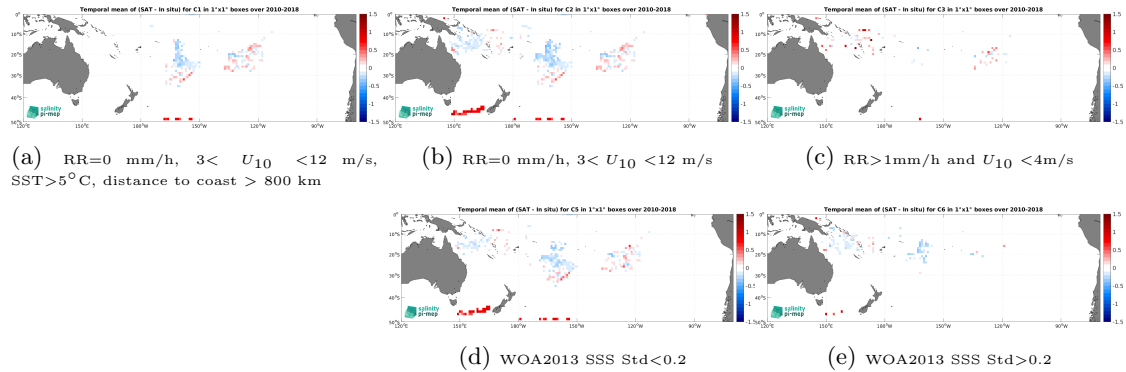
Figure 13: Temporal mean gridded over spatial boxes of size 1^\circ \times 1^\circ of \Delta SSS (CCI SSS L4 Merged-OI v5.5 - 30-day running (ESA) - Surface drifters) for 5 different subdatasets corresponding to:RR=0 mm/h, 3 < U_{10} < 12 m/s, SST >5^\circ C, distance to coast > 800 km (a), RR=0 mm/h, 3 < U_{10} < 12 m/s (b), RR >1 mm/h and U_{10} < 4 m/s (c), WOA2013 SSS Std <0.2 (d), WOA2013 SSS Std >0.2 (e).
