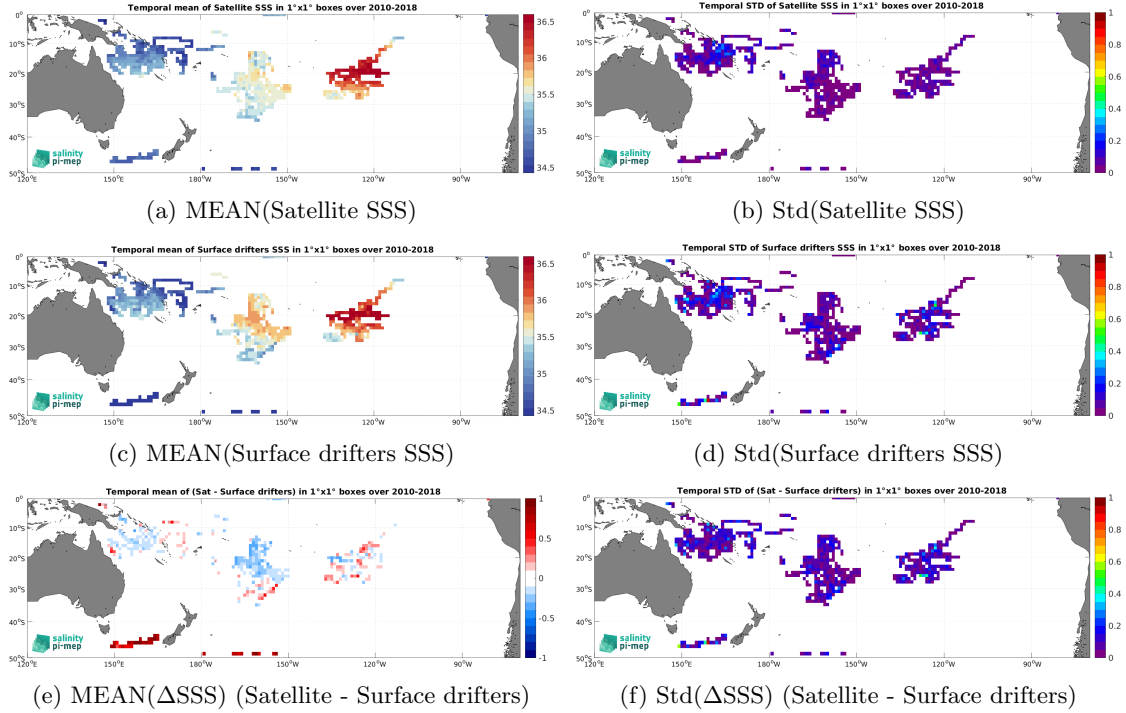
Figure 6: Temporal mean (left) and Std (right) of SSS from CCI SSS L4 Merged-OI v5.5 - 30-day running (ESA) (top), Surface drifters (middle), and of \Delta SSS (Satellite - Surface drifters). Only match-up pairs are used to generate these maps.
