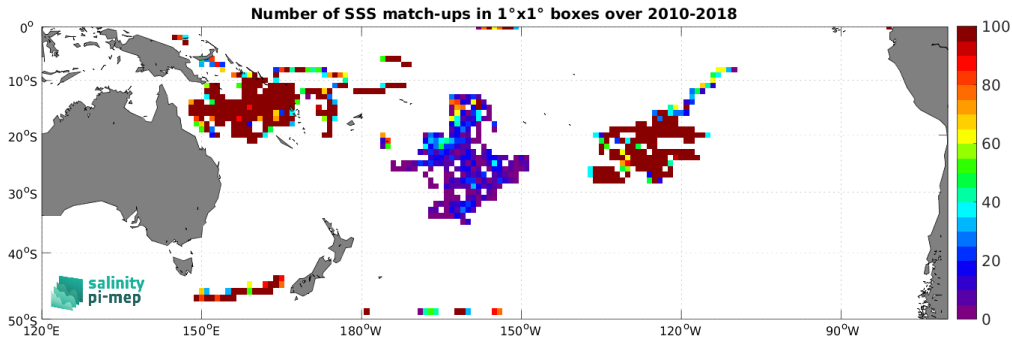
Figure 4: Number of SSS match-ups between Surface drifters SSS and the CCI SSS L4 Merged-OI v5.5 - 30-day running (ESA) SSS product for the South Pacific Ocean Pi-MEP region over 1^\circ \times 1^\circ boxes and for the full satellite product period.
