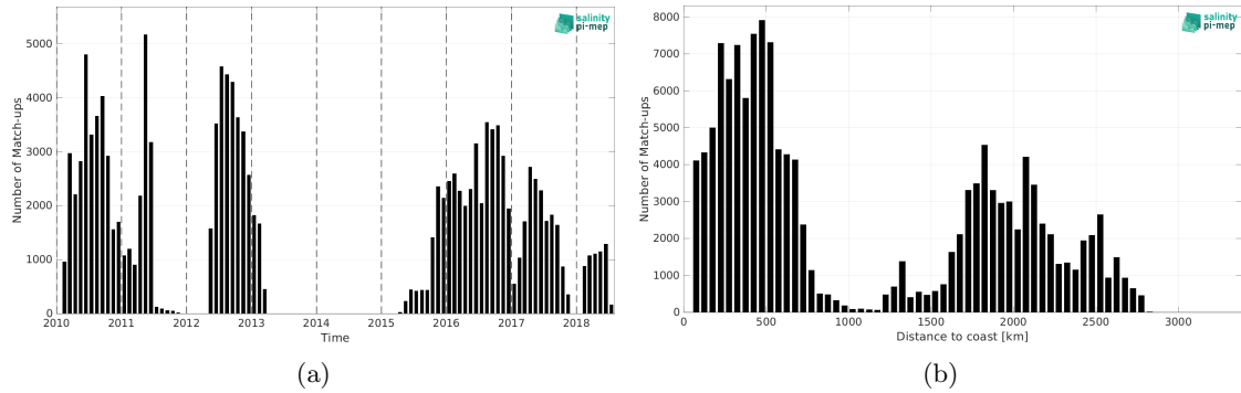
Figure 2: Number of match-ups between Surface drifters and CCI SSS L4 Merged-OI v5.5 - 30-day running (ESA) SSS as a function of time (a) and as function of the distance to coast (b) over the South Pacific Ocean Pi-MEP region and for the full satellite product period.
