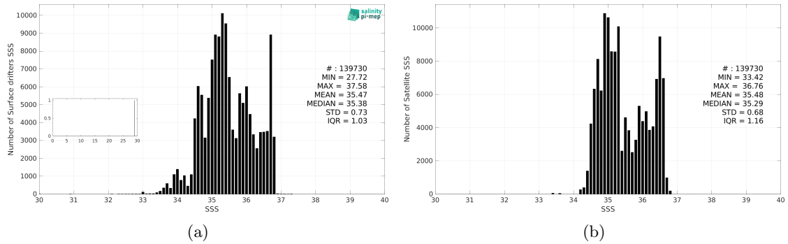
Figure 3: Histograms of SSS from Surface drifters (a) and CCI SSS L4 Merged-OI v5.5 - 30-day running (ESA) (b) considering all match-up pairs per bins of 0.1 over the South Pacific Ocean Pi-MEP region and for the full satellite product period.
